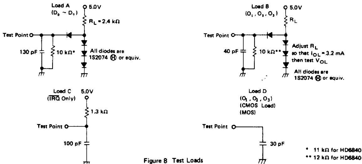
Figure 8 Test Loads
