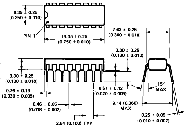
PACKAGE A LEAD FINISH: SOLDER DIPPED
