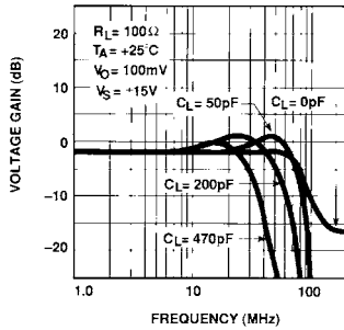
Voltage Gain vs Frequency for Various Capacitive Loads; RL = 100 Ohm
