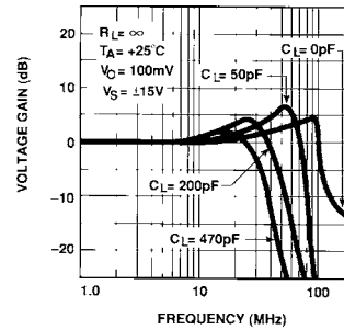
Voltage Gain vs Frequency for Various Capacitive Loads; RL = infinity
