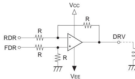
Fig. 5-21. Drive Circuit
