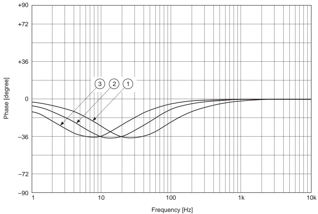
Fig. 5-26c. Servo LowBooster2 Characteristics [FCS, TRK] (MCK = 128Fs)
