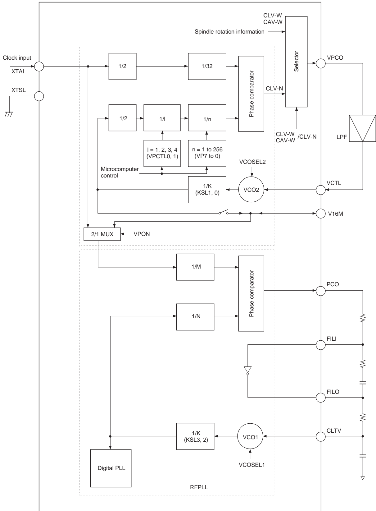
Block Diagram 4-1
