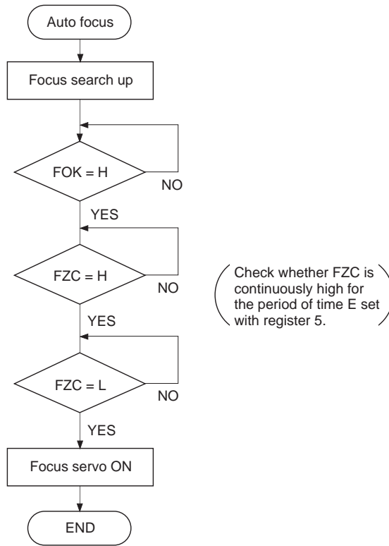
Fig. 4-6-(a). Auto Focus Flow Chart
