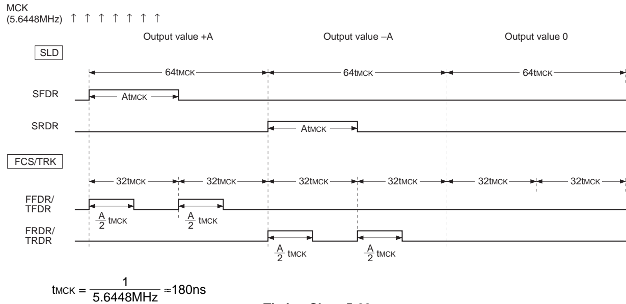
Timing Chart 5-20.
