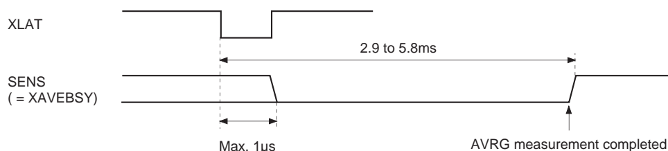
Timing Chart 5-2.
