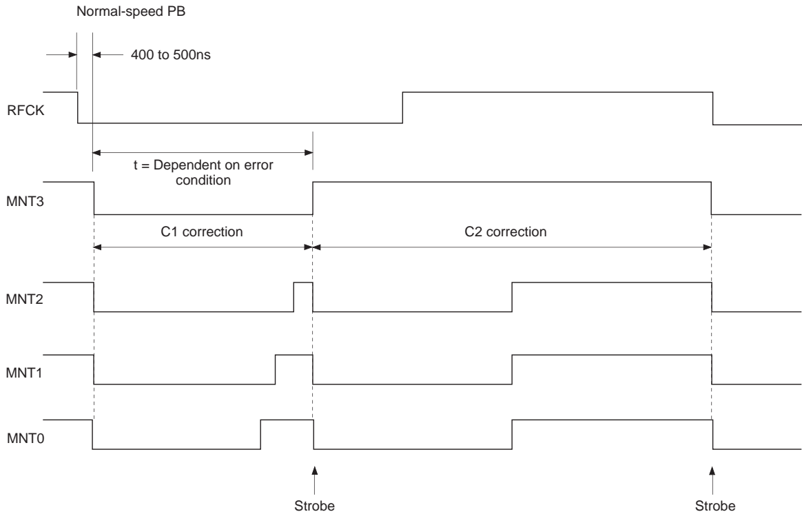
Timing Chart 4-3
