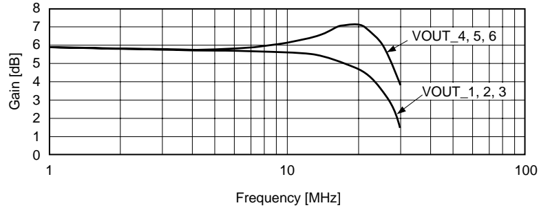
Video gain – VOUT_1, 2, 3, 4, 5, 6
