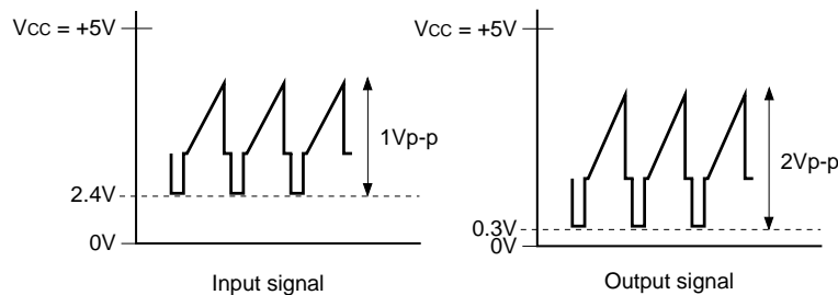
Fig. 10. CVBS/Y Waveforms
