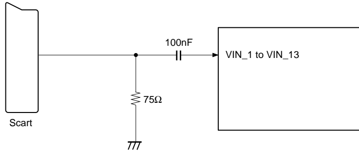
Fig. 15. Video Input Interface
