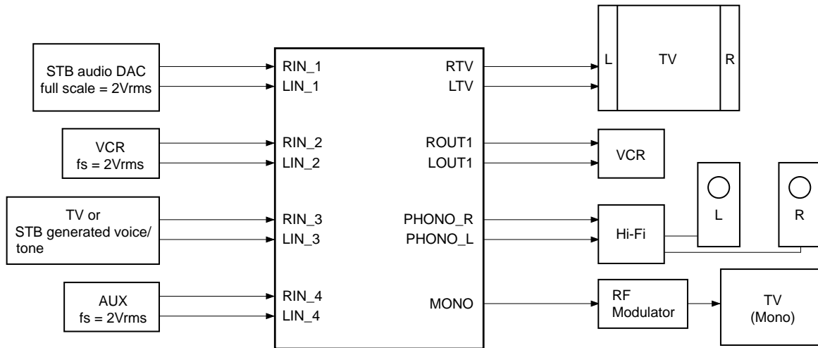
Fig. 23. Audio Application
