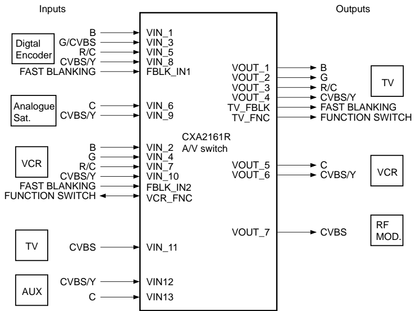
Fig. 22. Video Application with 4 Output Digital Encoder
