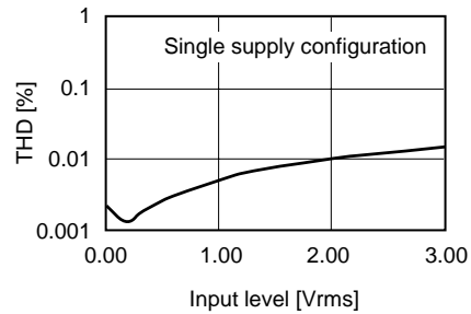
Audio output distortion ROUT1, LOU1
