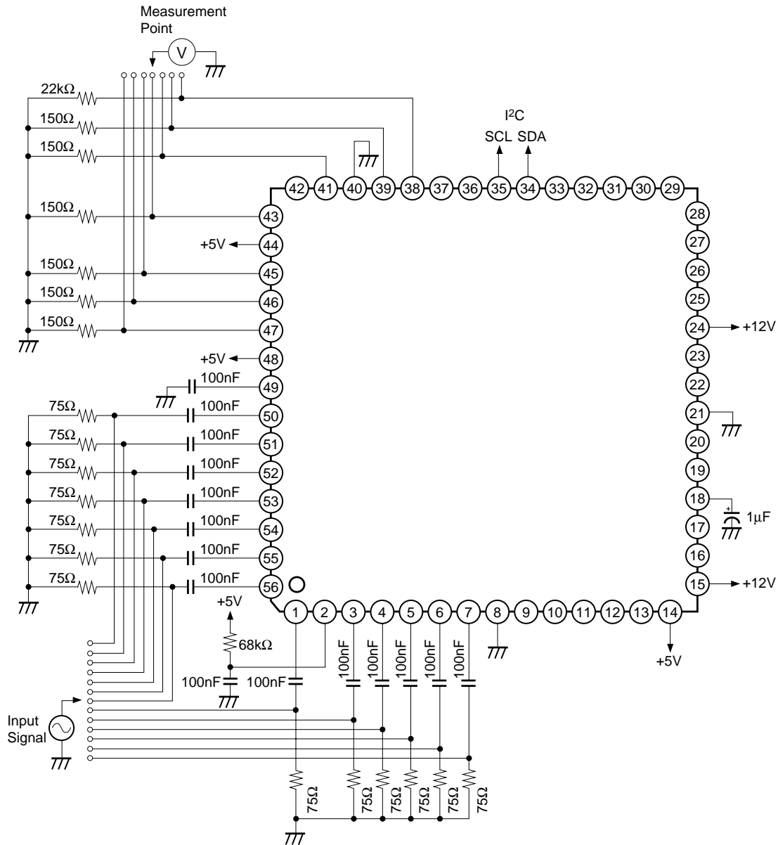
Fig. 2. Video System
