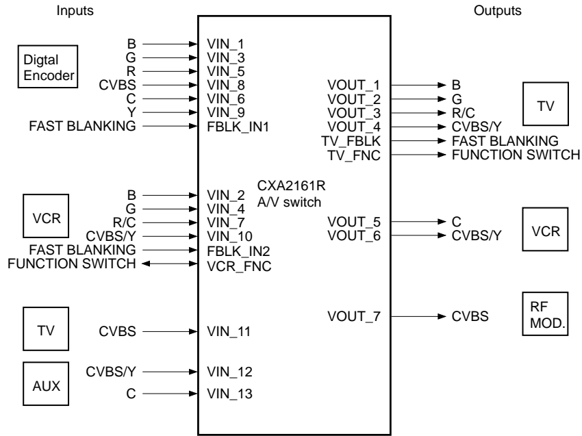
Fig. 21. Video Application with 6 Output Digital Encoder
