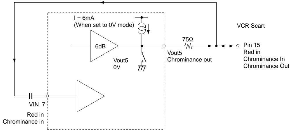
Fig 5. Bi-directional Line to VCR
