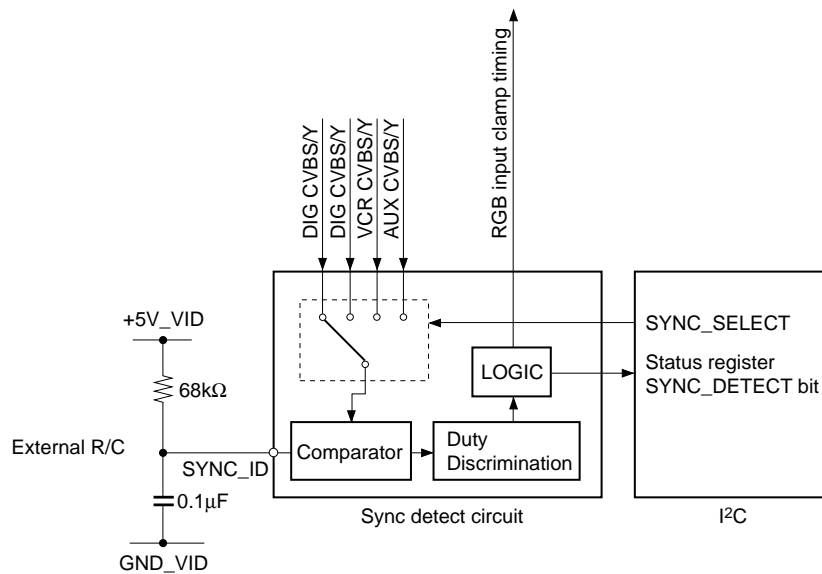
Fig. 12. Sync Detection Circuit
