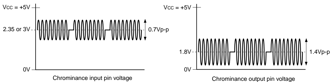
Fig. 13. Chrominance Waveforms
