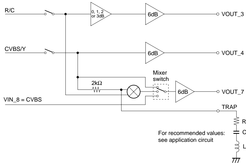
Fig. 14. Internal Y/C Mixer Circuit
