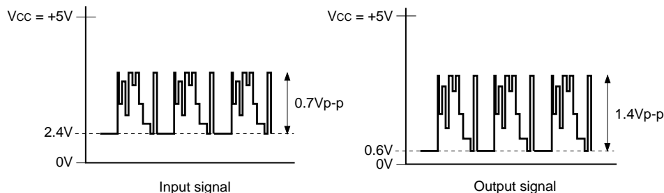
Fig. 11. RGB Waveforms
