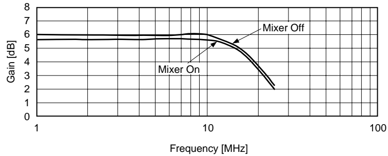
Video gain – VOUT_7
