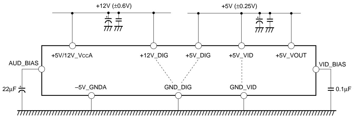
Fig. 25. Single Ended Supply
