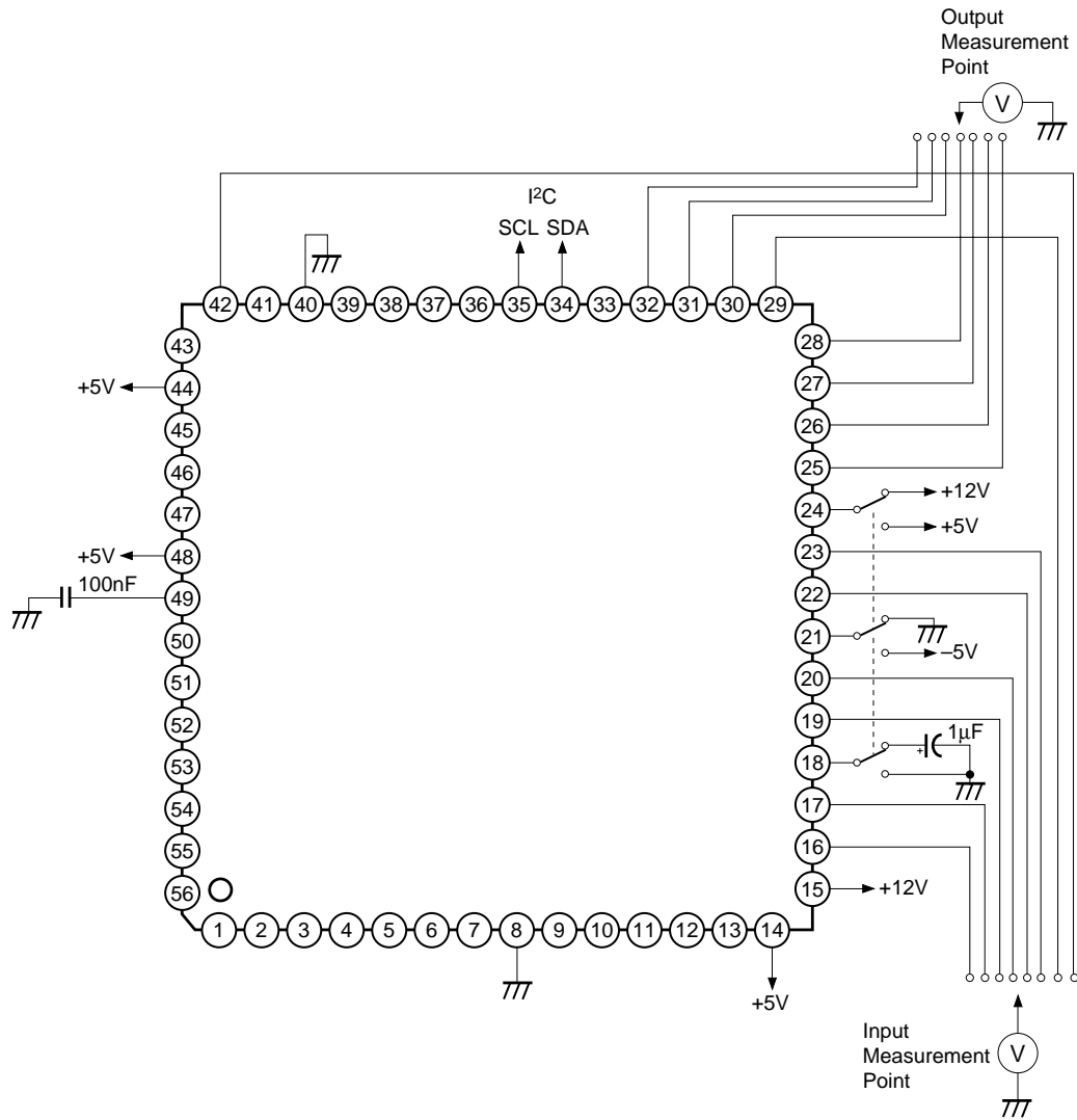
Fig. 3. Audio System (DC Tests)
