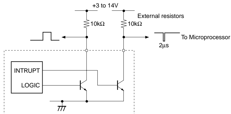
Fig. 8. INTRUPT and Logic Line Interface
