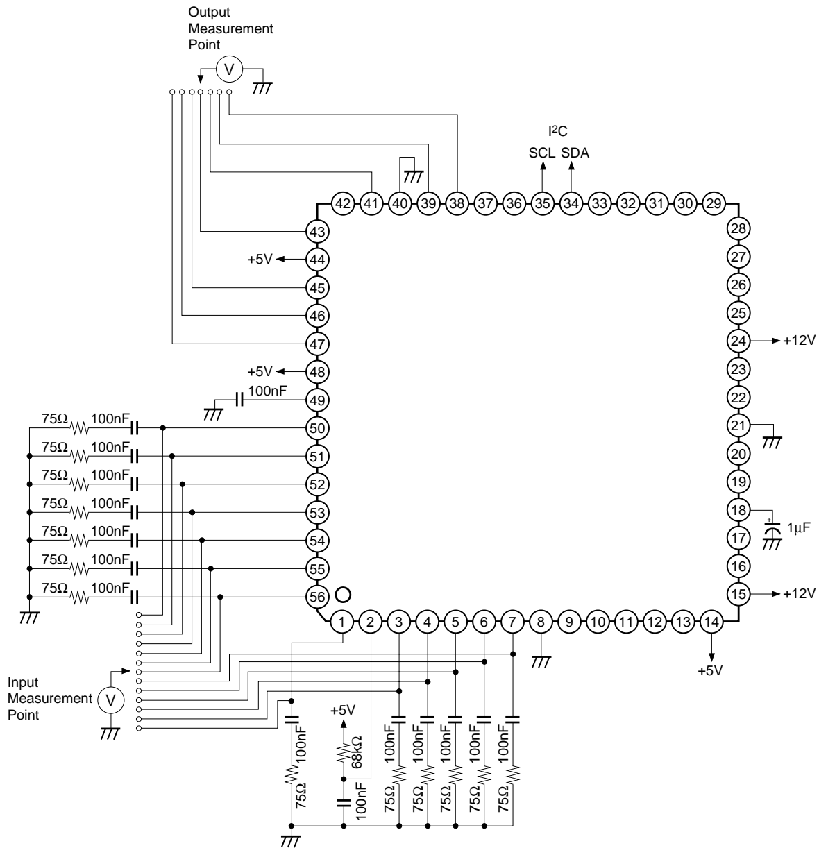
Fig. 1. Video System (DC Test)
