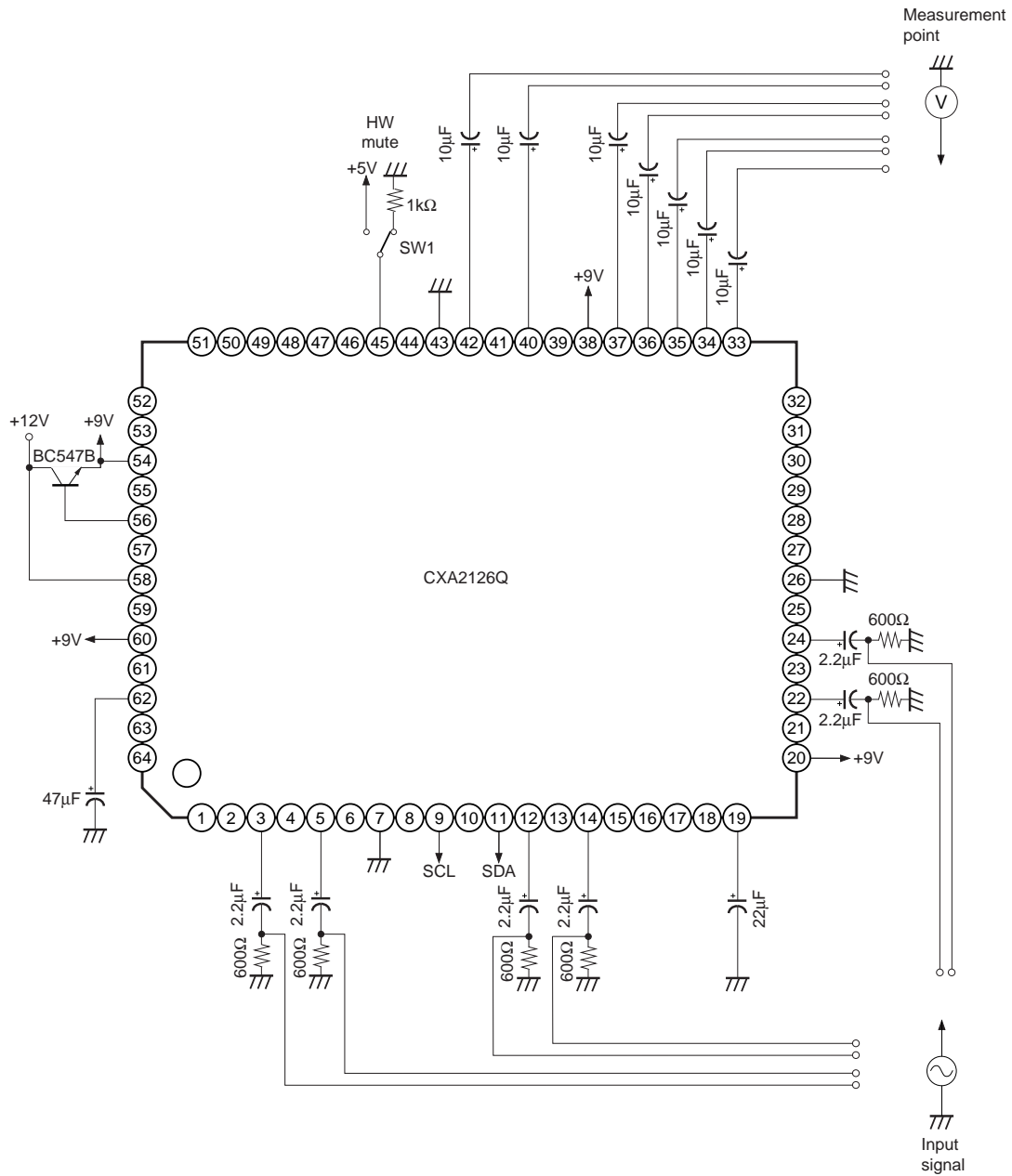
Fig. 7. Audio system (bandwidth and frequency response)
