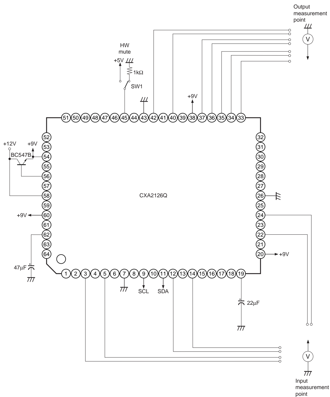
Fig. 5. Audio system (d.c. tests)
