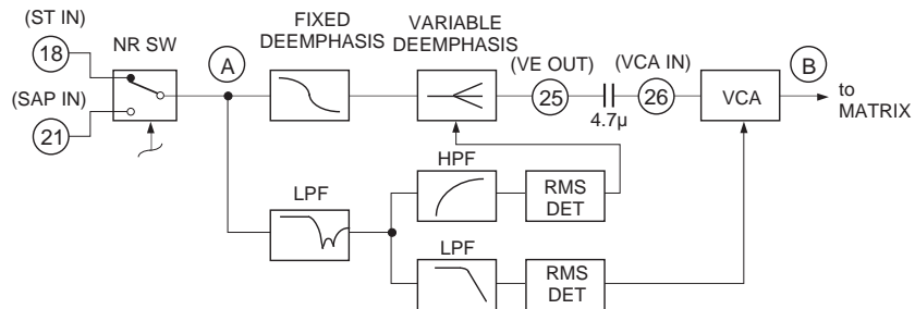
Fig 3. dbx-TV block
