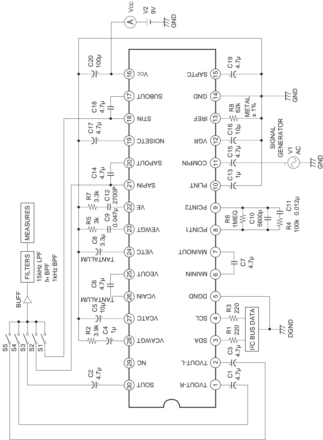
Electrical Characteristics Measurement Circuit
