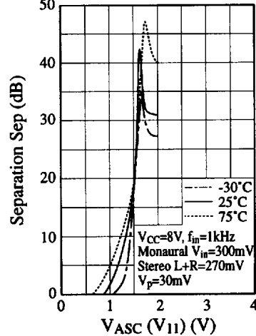
ASC Characteristics
