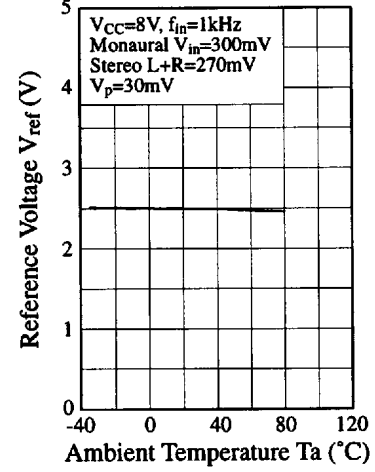
V_{REF} - T_a
