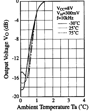
ATC Characteristics
