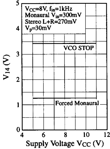
Forced Monaural ON Level - V_{CC}
