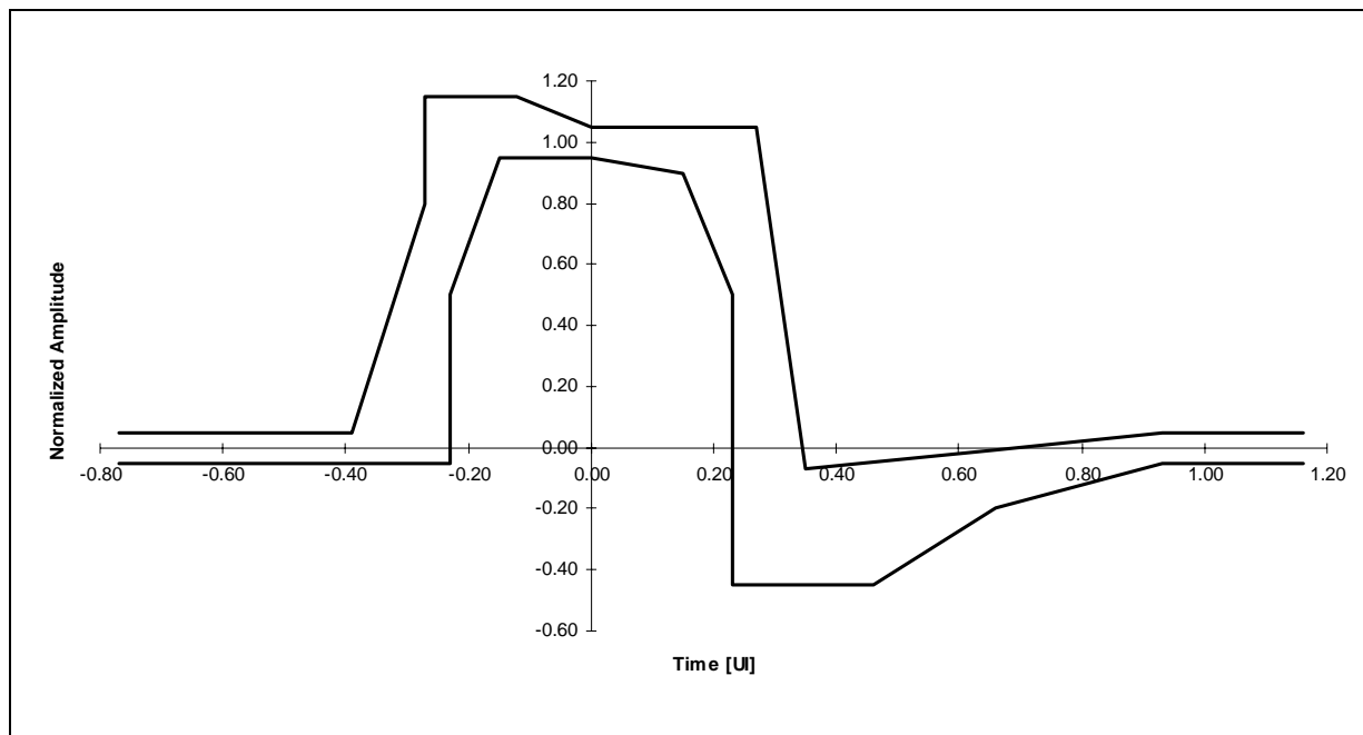
Figure 32. T1, T1.102 Mask Templates
