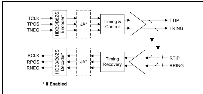
Figure 9. Analog Loopback
