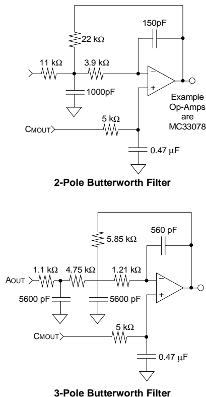
Figure 7. Butterworth Filters
