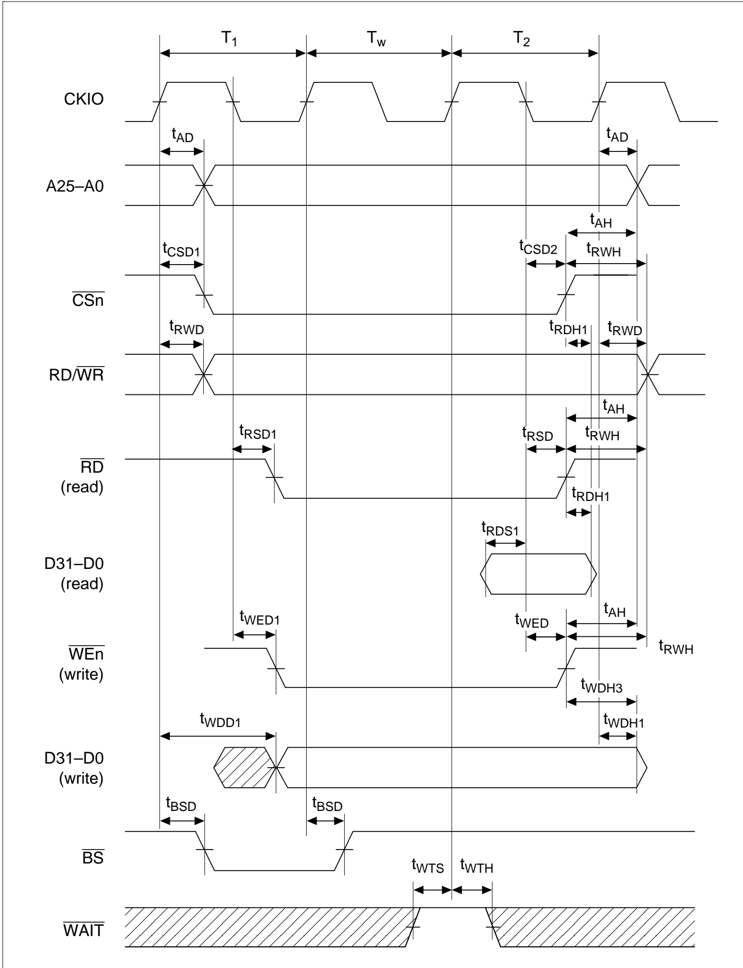
Figure 17.18 Basic Bus Cycle (1 Wait)
