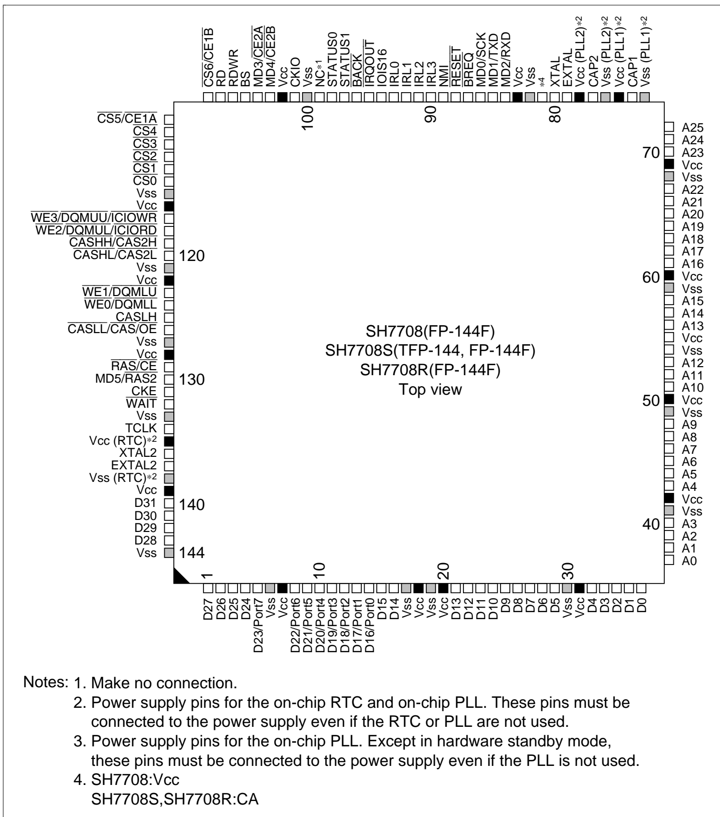
Figure 1.2 Pin Arrangement
