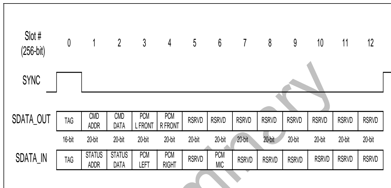
Figure 16-4. Bi-directional AC-link Frame with Slot Assignments
