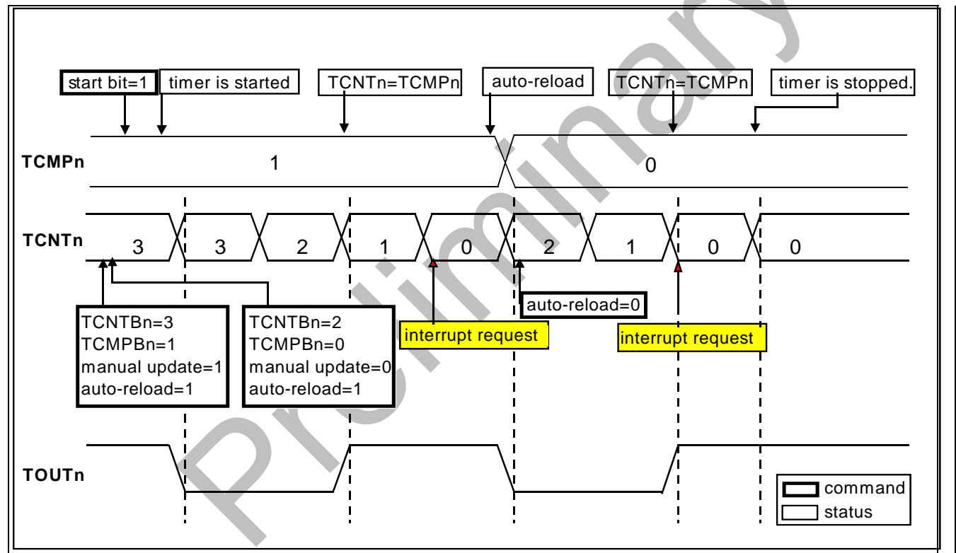
Figure 7-2. Timer operations
