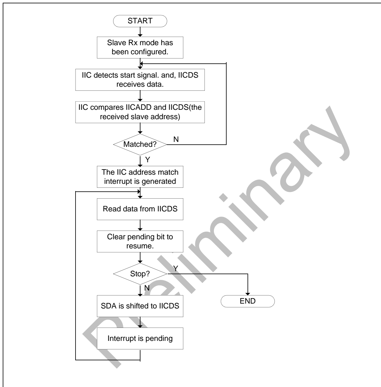
Figure 13-9 Operations for Slave / Receiver Mode
