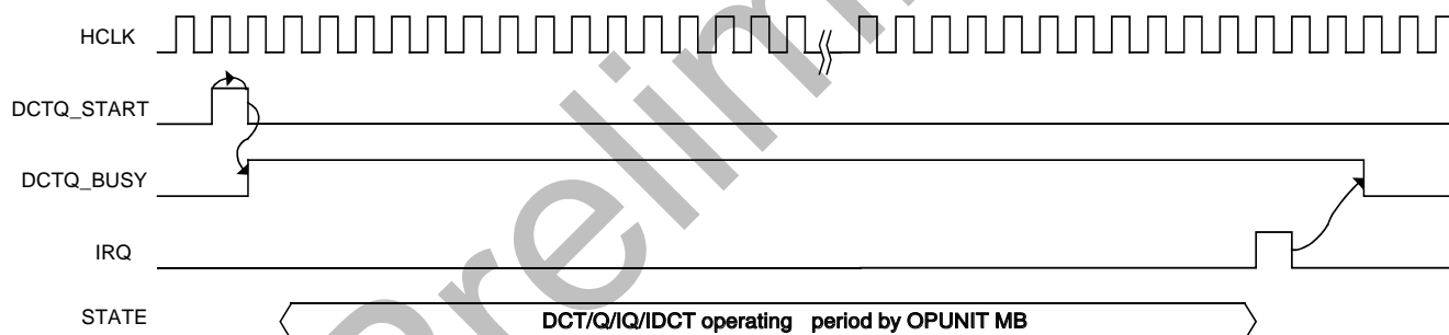
Figure 25-2. DCTQ operation timing diagram
