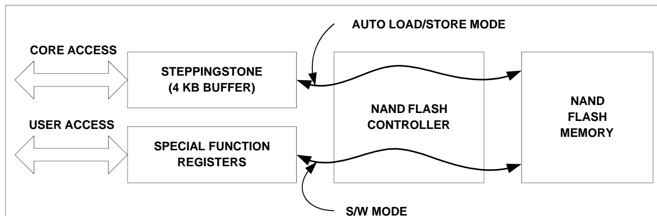
Figure 4-3 NAND Flash Controller Operation Mode Block Diagram
