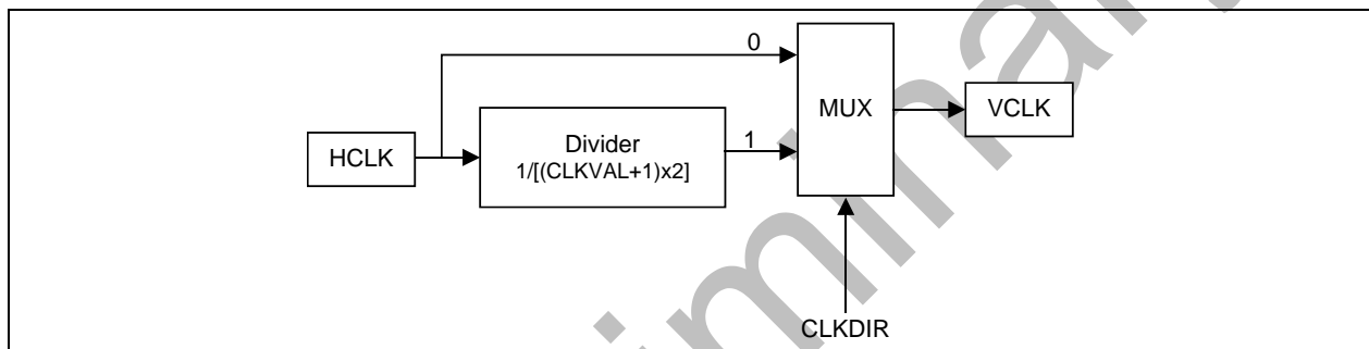
Figure 28-2. Clock Selection
