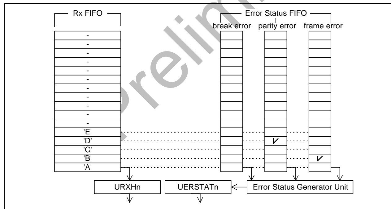
Figure 11-3. Example showing UART Receiving 5 Characters with 2 Errors
