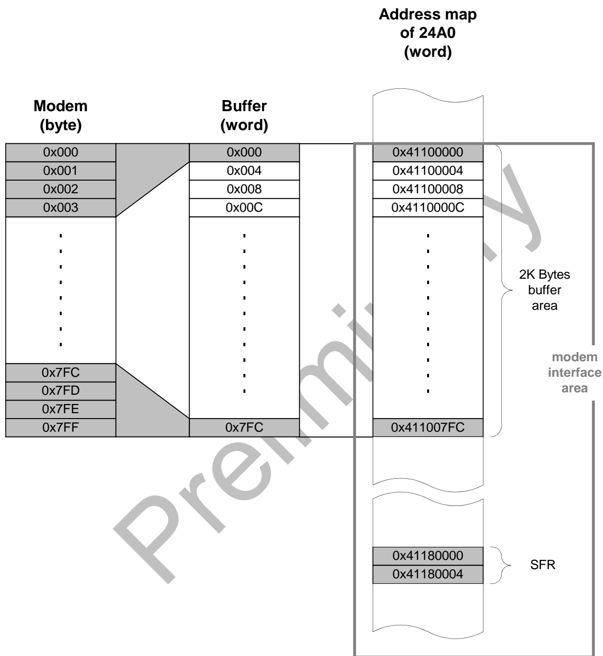
Figure 19-2 Modem interface address mapping
