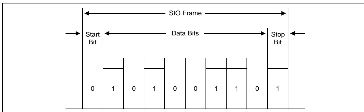
Figure 11-4. Serial I/O Frame Timing Diagram (Normal UART)
