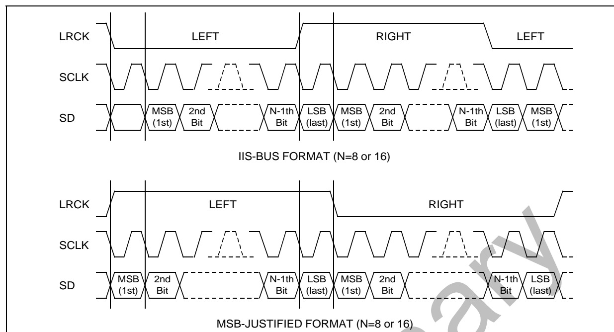
Figure 14-2. IIS-Bus and MSB(Left)-justified Data Interface Formats
