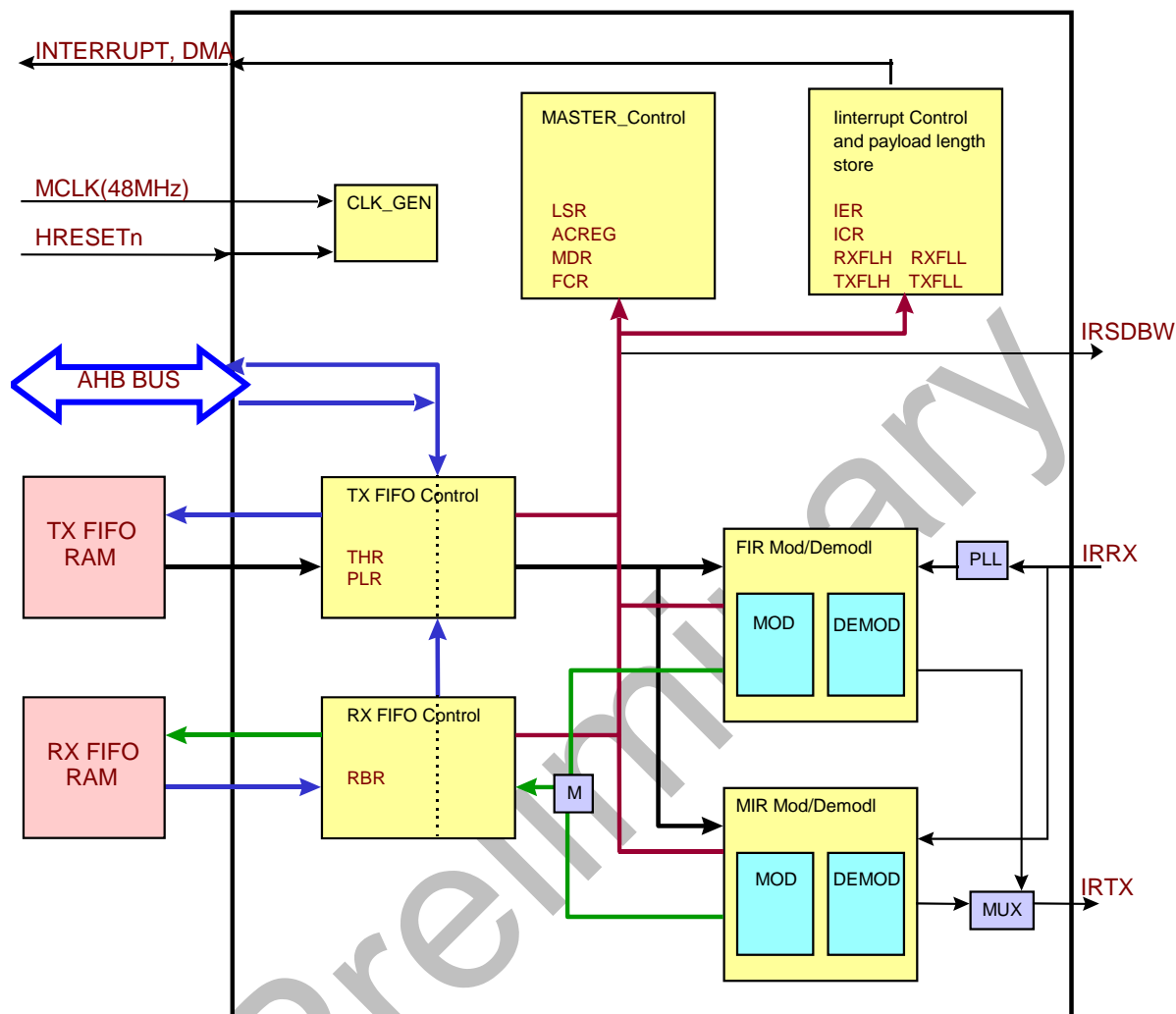
Figure 12-1. Block Diagram
