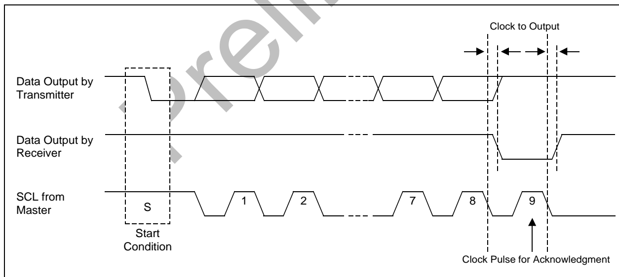
Figure 13-5. Acknowledge on the IIC-Bus
