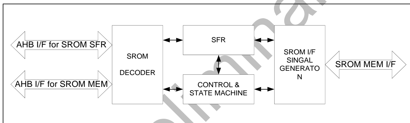
Figure 2-2 SROM Controller Block Diagram
