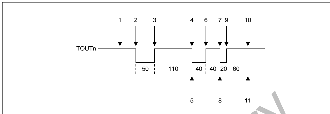
Figure 7-4. Example of a Timer Operation
