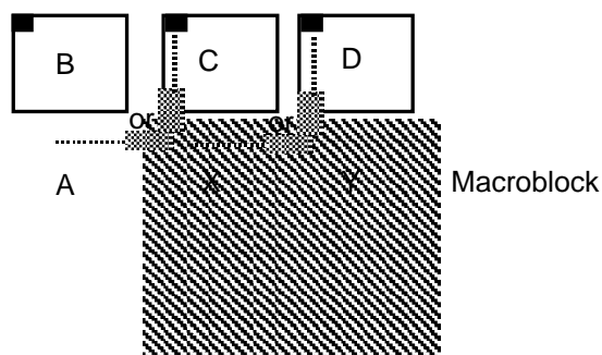
Figure 26-3 Previous neighboring blocks used in DC prediction
