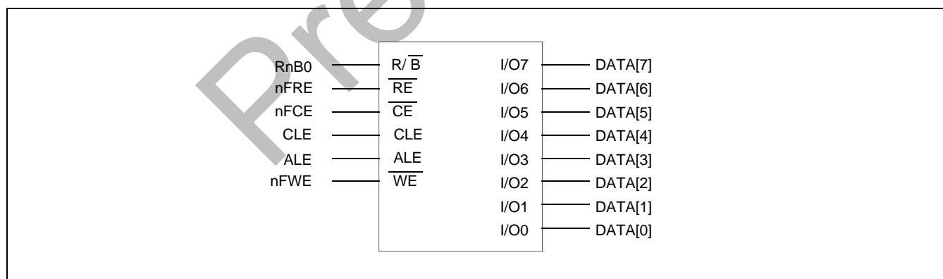
Figure 4-7 8-bit NAND Flash Memory Interface
