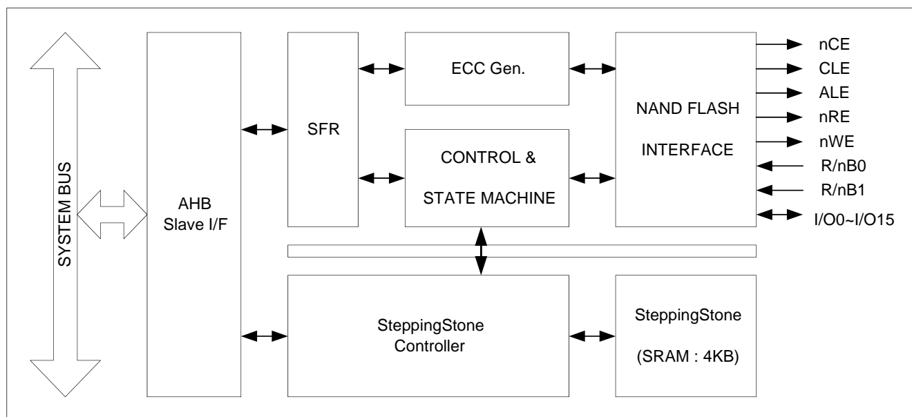
Figure 4-1 NAND Flash Controller Block Diagram
