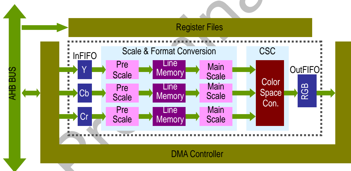
Figure 27-1. Block Diagram of Post Processor
