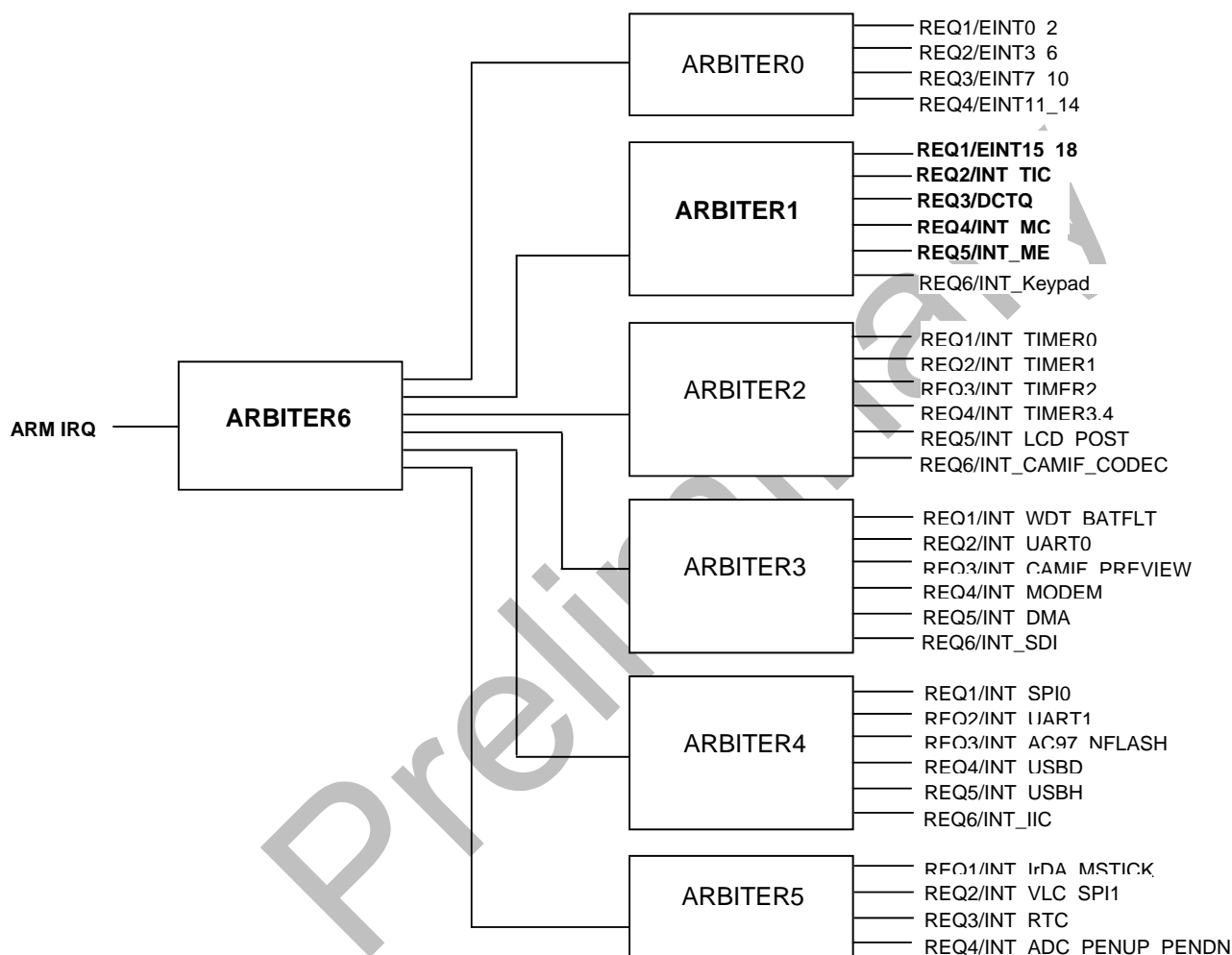
Figure 6-1. Priority Generating Block
