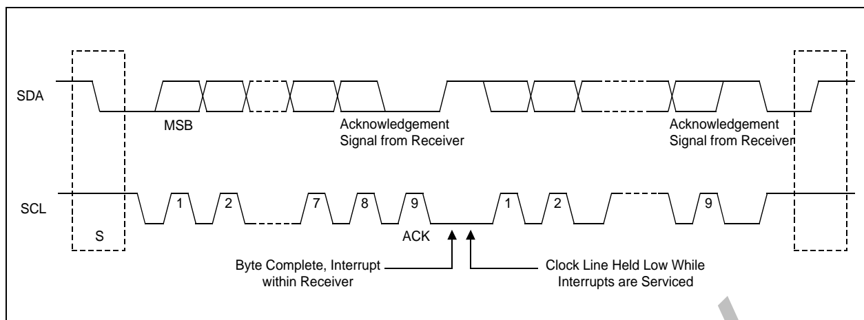
Figure 13-4. Data Transfer on the IIC-Bus
