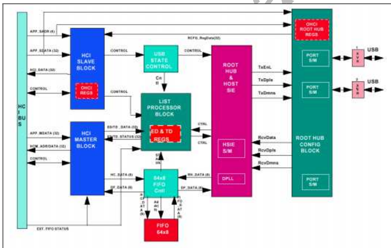
Figure 17-1. USB Host Controller Block Diagram
