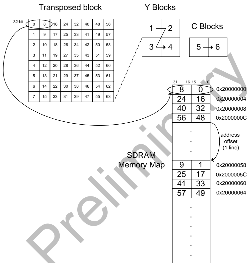
Figure 25-7. Transposed coefficient output for MB
