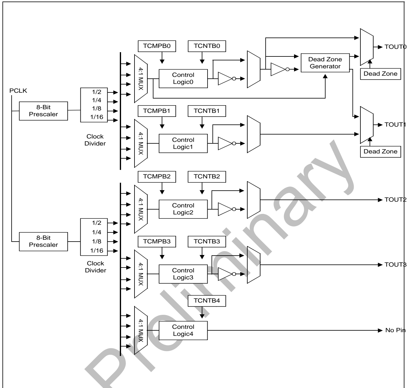
Figure 7-1. 16-bit PWM Timer Block Diagram
