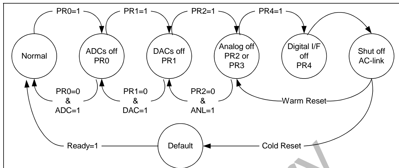
Figure 16-8 AC97 Power down/Power up Flow
