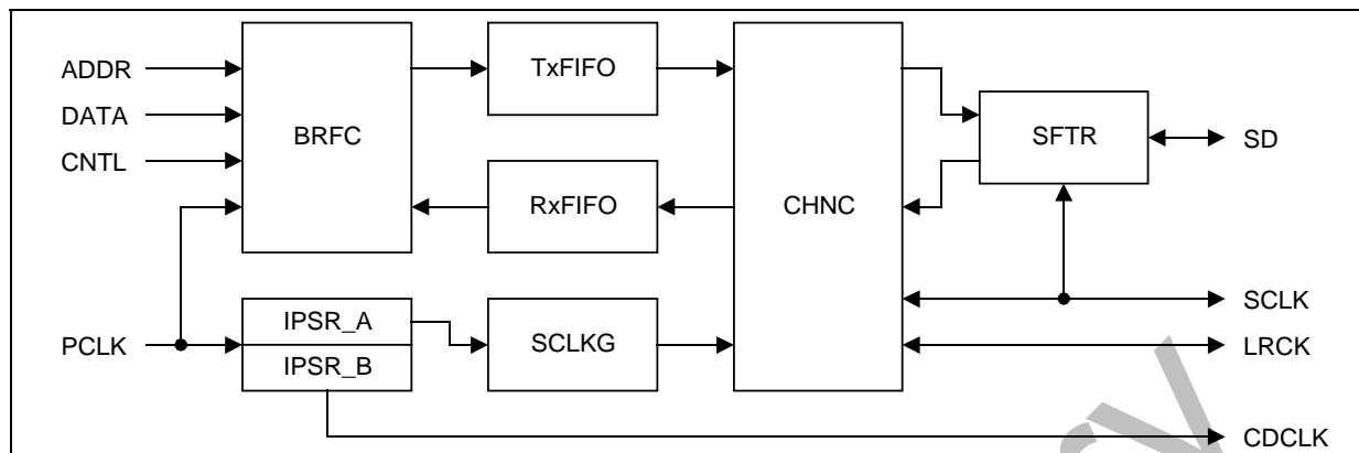
Figure 14-1. IIS-Bus Block Diagram
