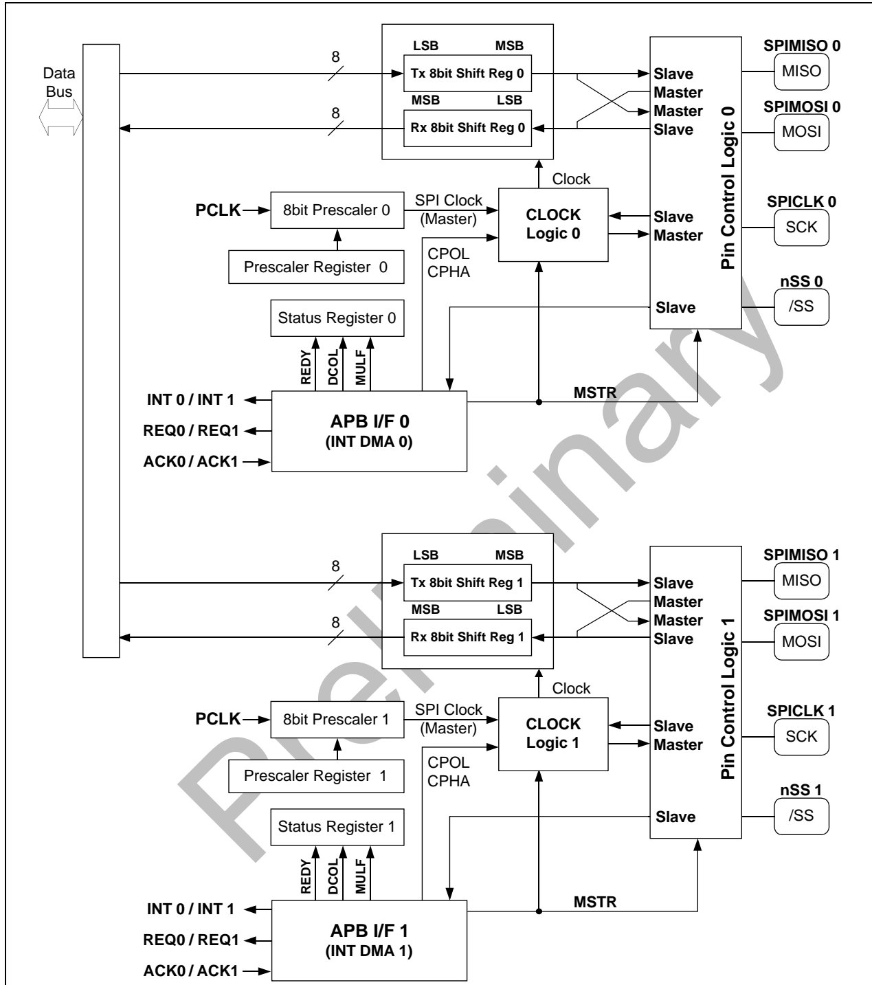
Figure 15-1. SPI Block Diagram
