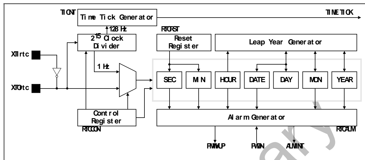
Figure 10-1. Real Time Clock Block Diagram
