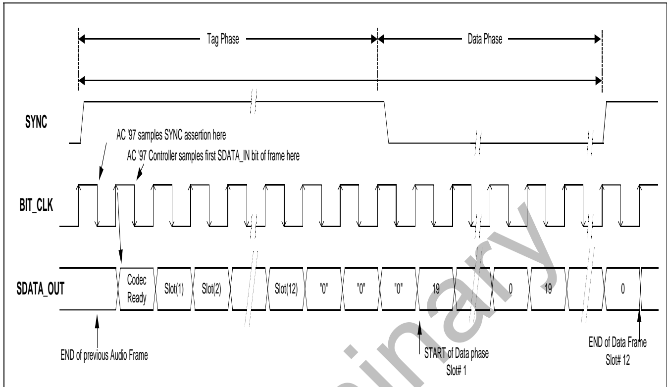
Figure 16-6. AC-link Input Frame
