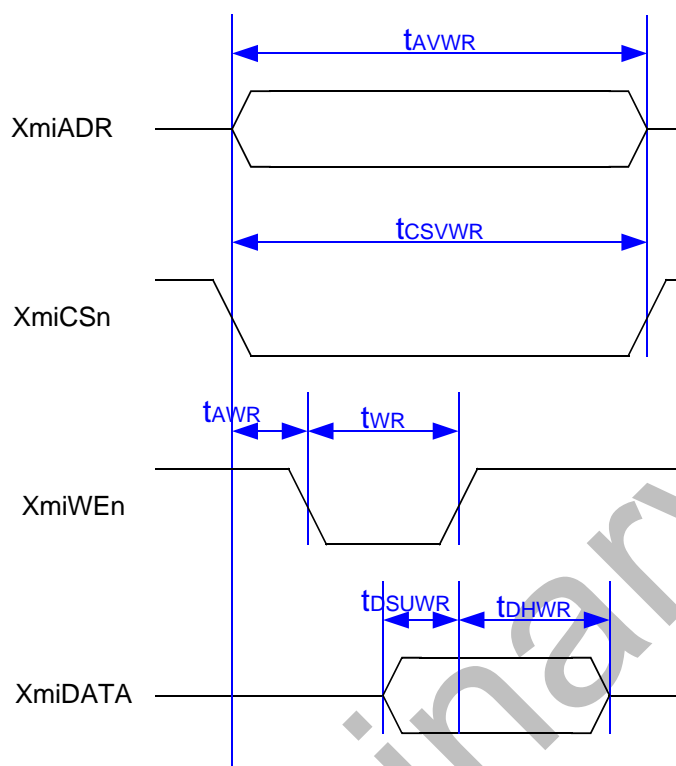
Figure 19-3 Modem interface write timing diagram
