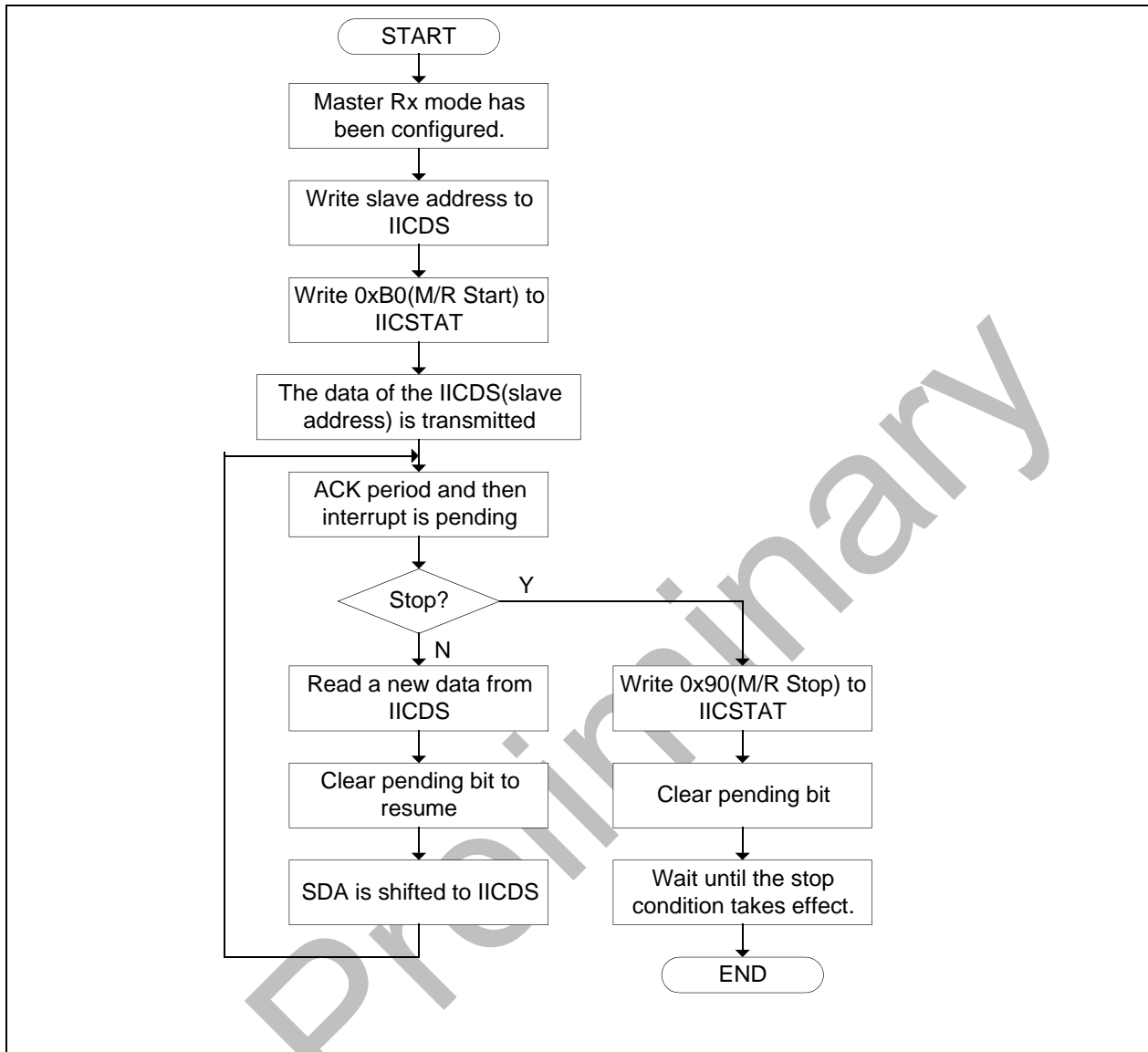
Figure 13-7 Operations for Master / Receiver Mode
