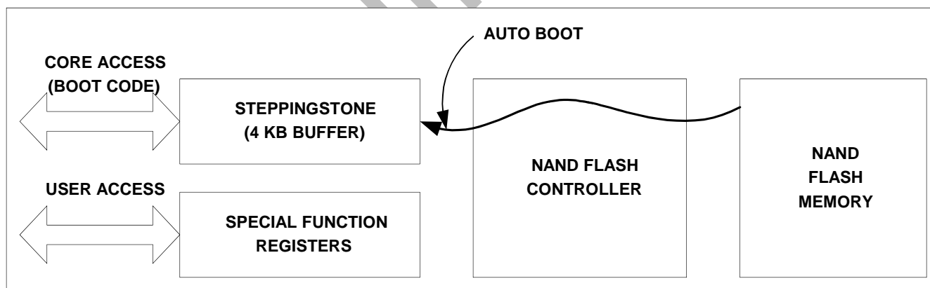
Figure 4-2 NAND Flash Controller Boot Loader Block Diagram
