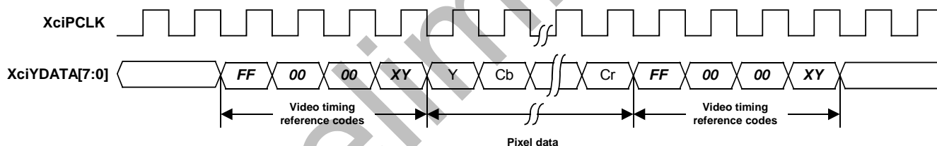
Figure 21-3. ITU-R BT 656 Input timing diagram
