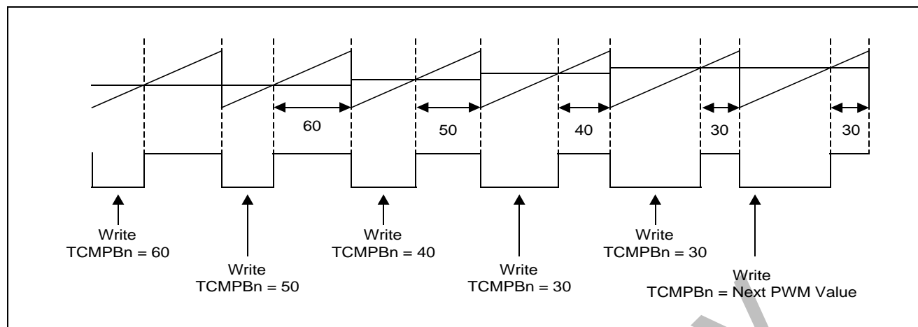
Figure 7-5. Example of PWM
