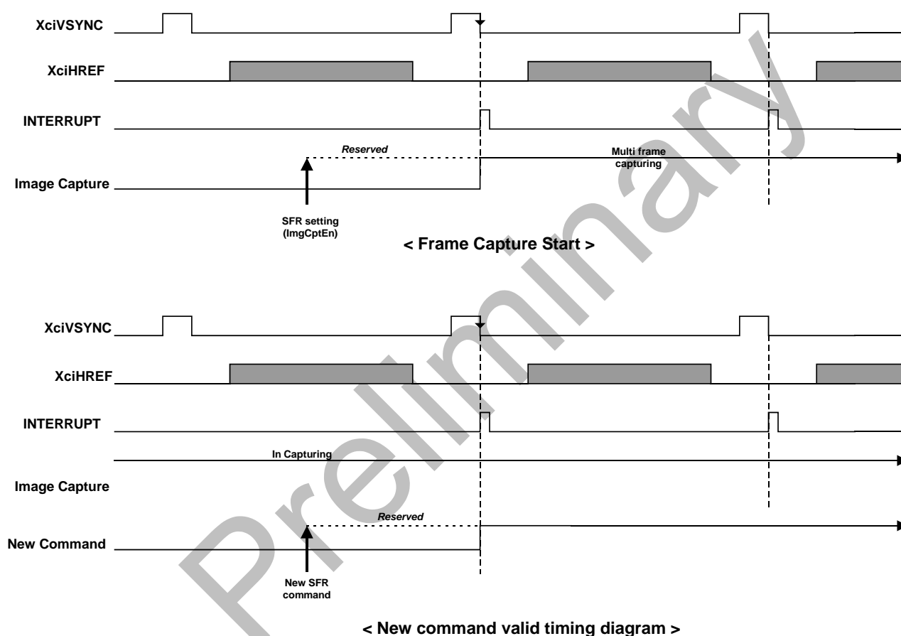
Figure 21-11. Timing diagram for register setting
