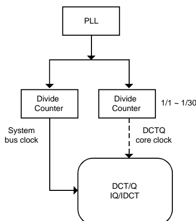
Figure 25-3. DCTQ clock domain
