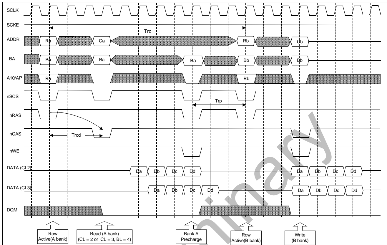
Figure 3-3. SDRAM Timing Diagram
