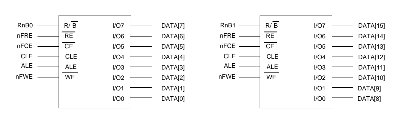
Figure 4-8 Two 8-bit NAND Flash Memory Interface
