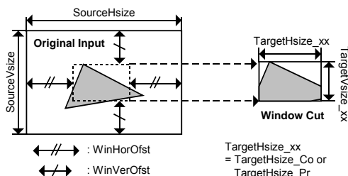
Figure 21-13 Window offset scheme
