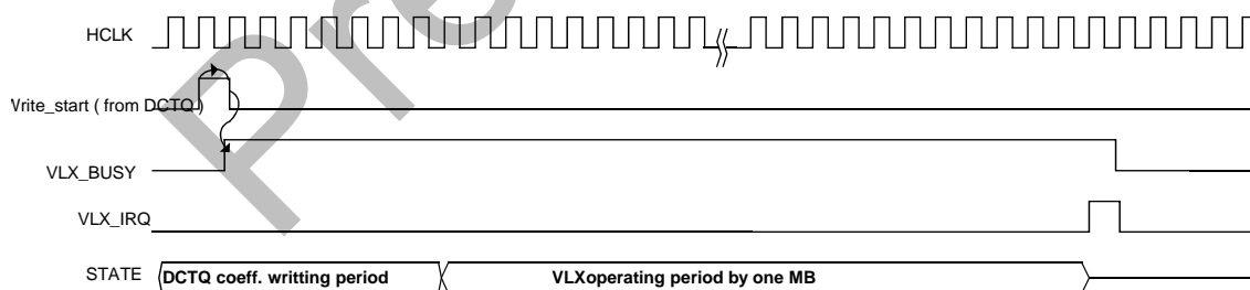
Figure 26-5 VLC start, busy, and Interrupt signal timing diagram.
