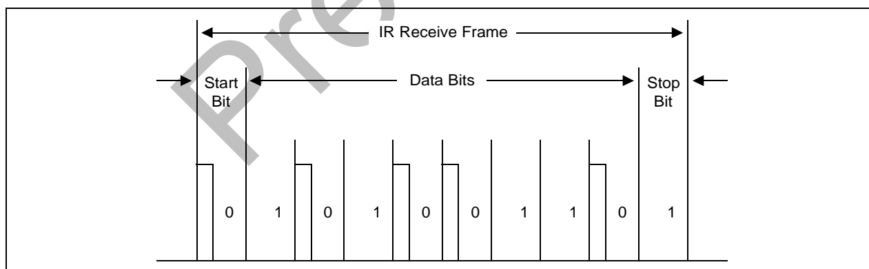
Figure 11-6. Infrared Receive Mode Frame Timing Diagram
