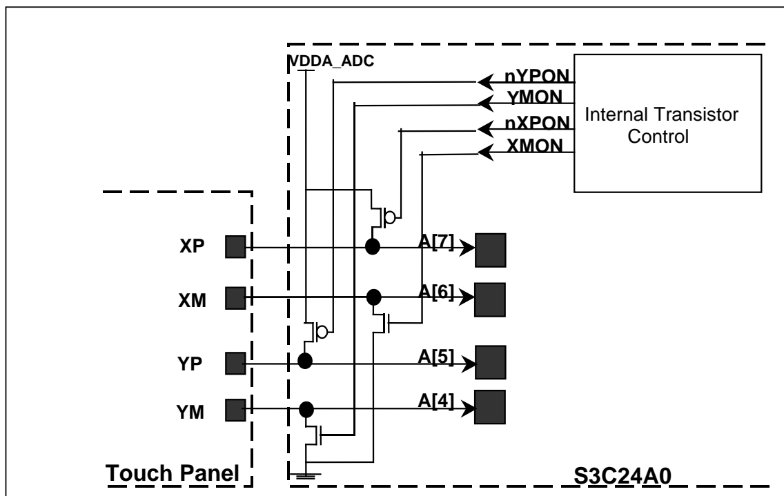
Figure 30-2. Example of ADC and Touch Screen Interface
