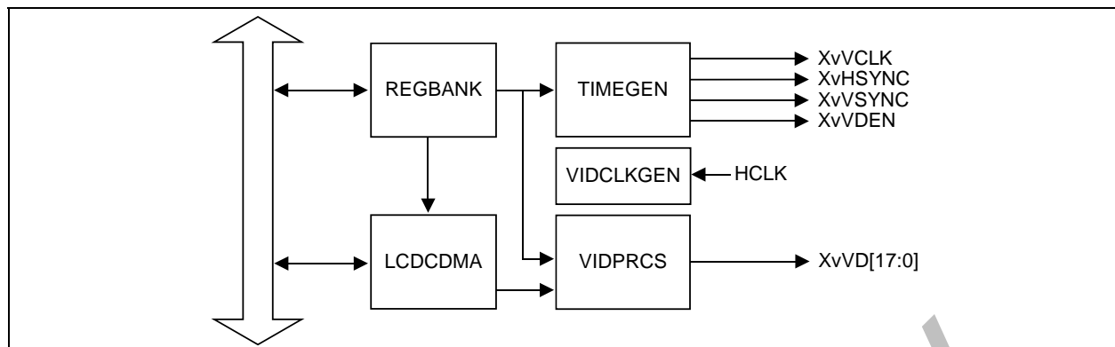
Figure 28-1. LCD Controller Block Diagram
