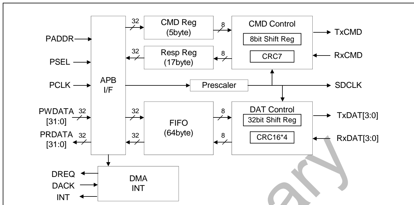
Figure 31-1. SDI Block Diagram
