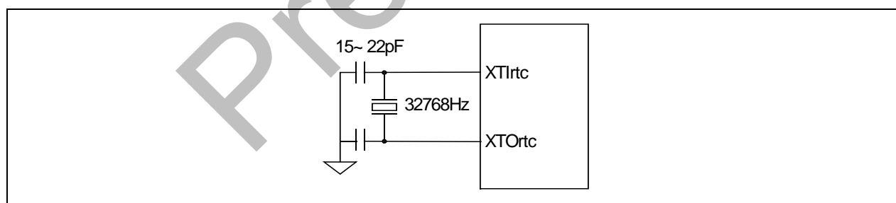
Figure 10-2. Main Oscillator Circuit Examples
