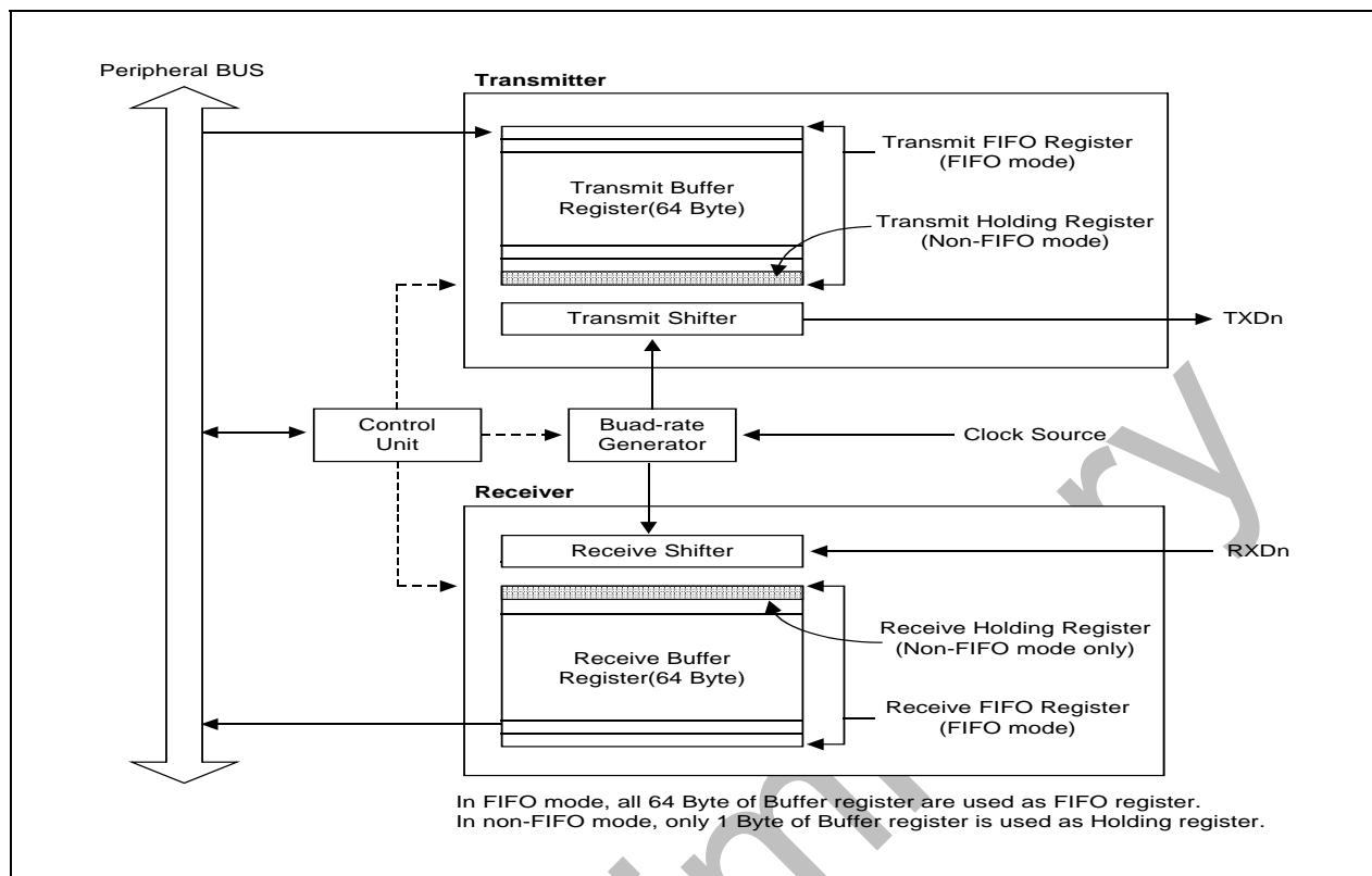
Figure 11-1. UART Block Diagram (with FIFO)
