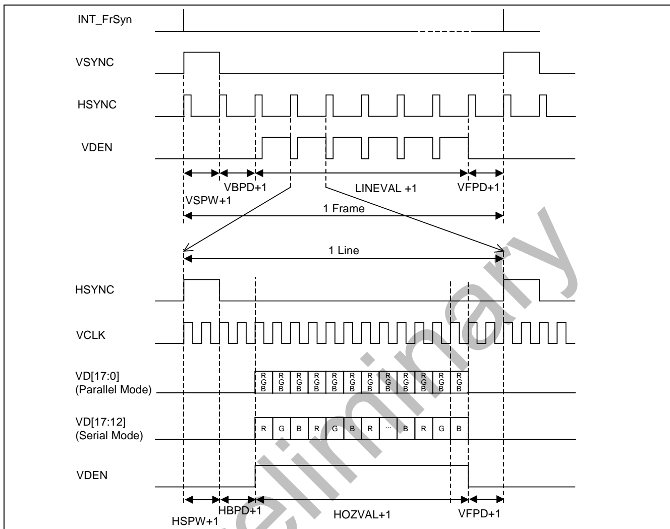
Figure 28-6. TFT LCD Timing Example
