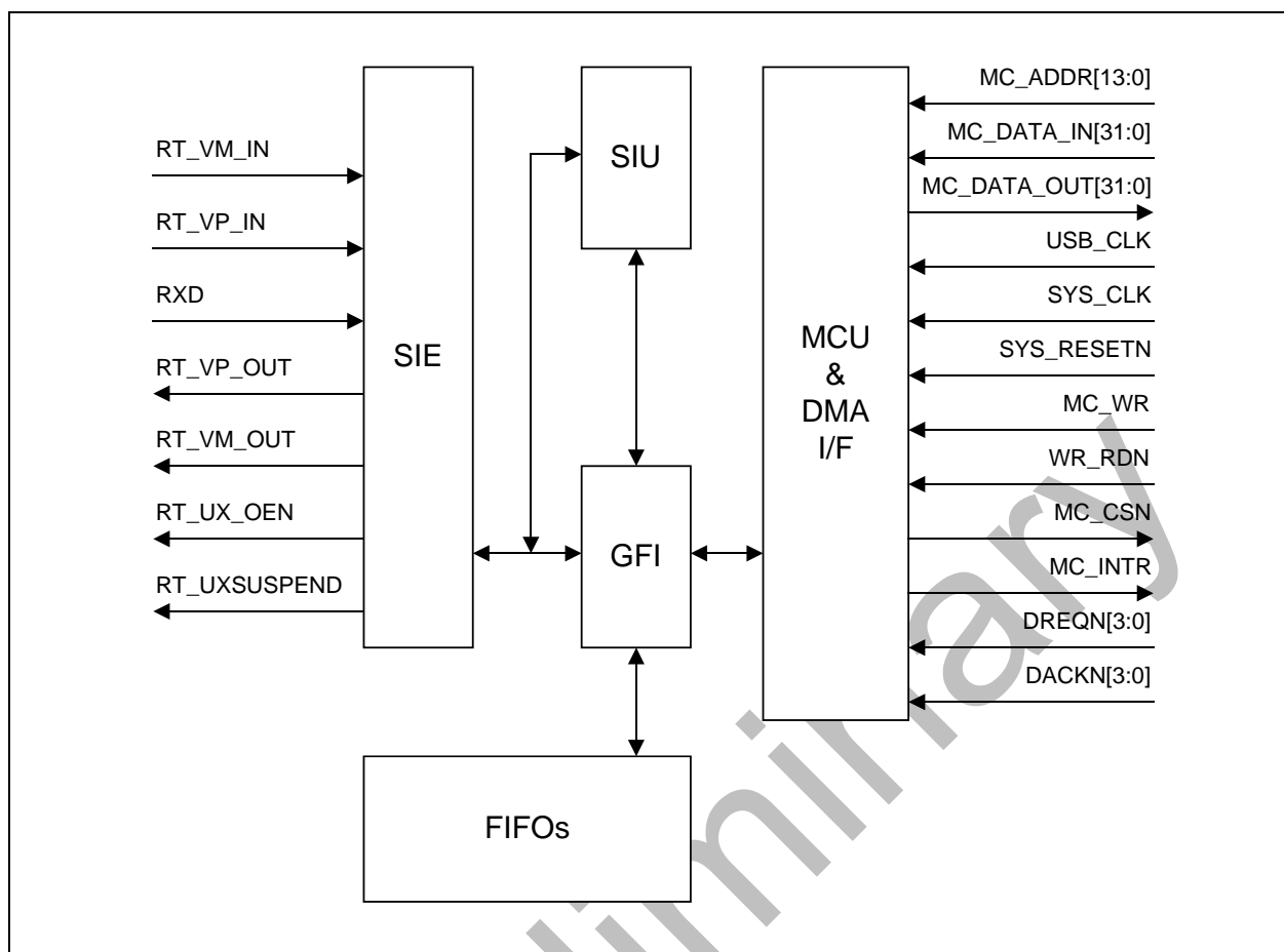
Figure 18-1. USB Device Block Diagram
