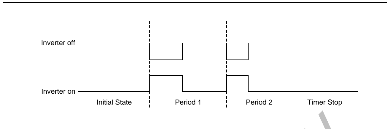
Figure 7-6. Inverter On/Off
