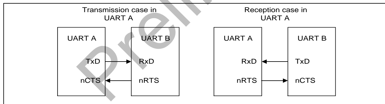
Figure 11-2. UART AFC interface
