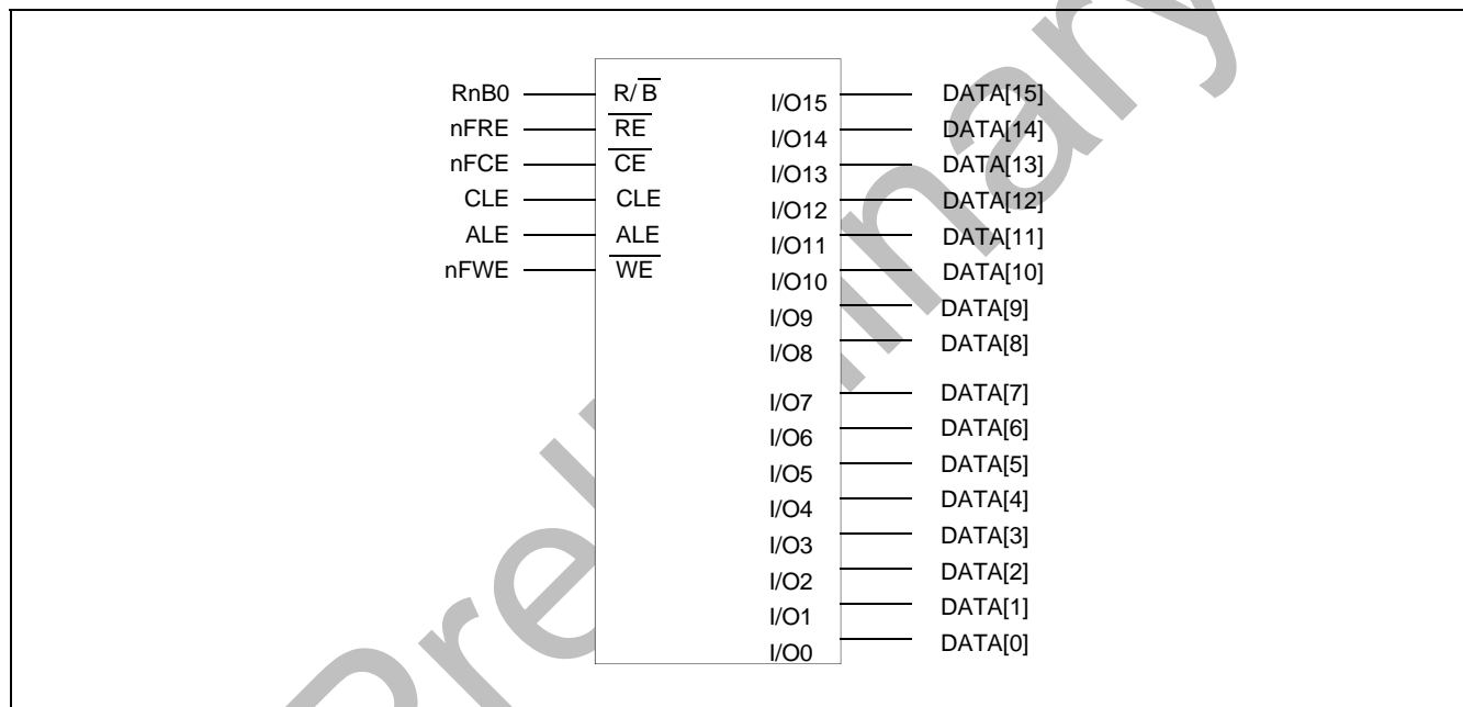
Figure 4-9 16-bit NAND Flash Memory Interface
