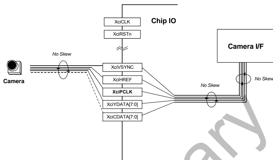
Figure 21-4. IO connection guide
