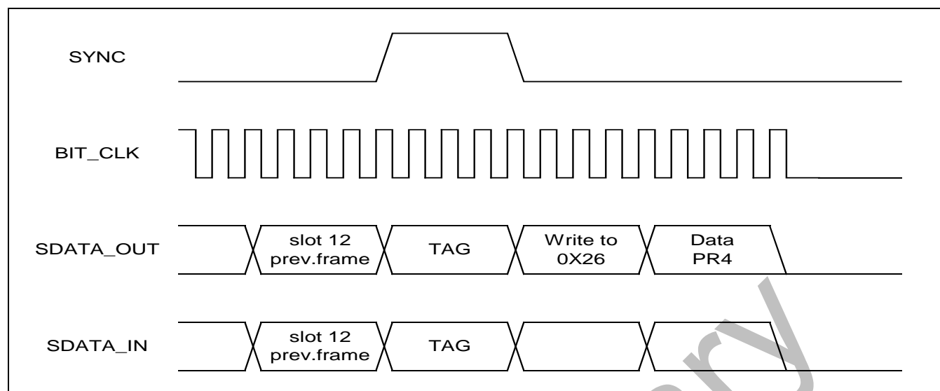
Figure 16-7. AC97 Powerdown Timing
