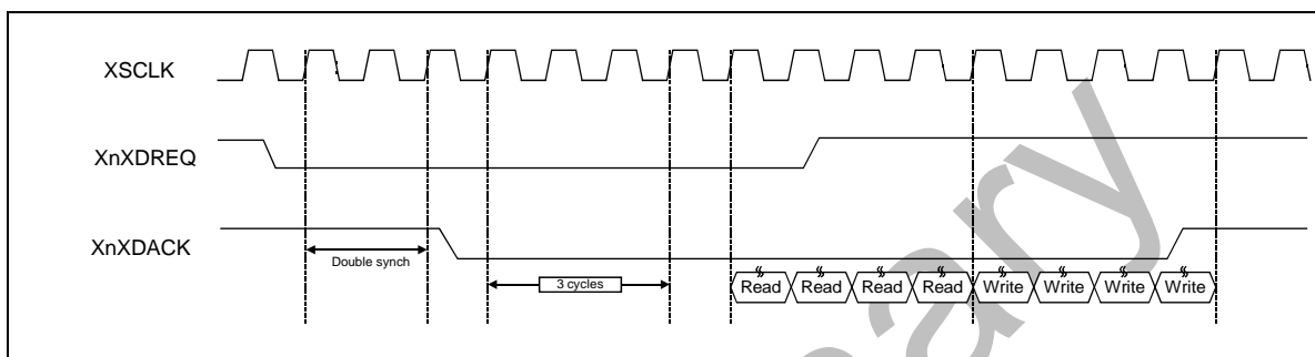
Figure 9-3. Burst 4 Transfer size
