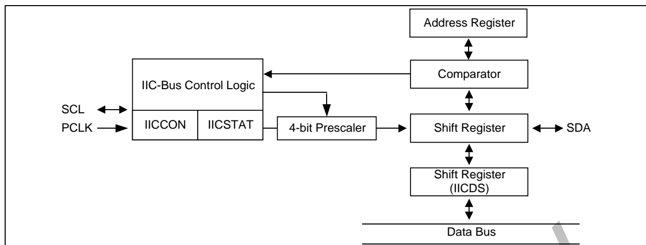
Figure 13-1. IIC-Bus Block Diagram
