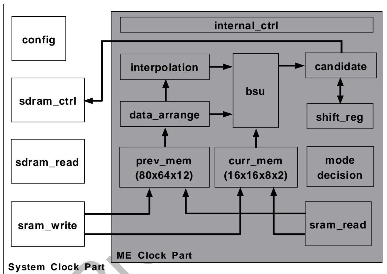
Figure 23-1. MPEG-4 Motion Estimation Block Diagram
