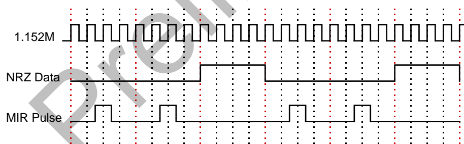
Figure 12-4. Pulse modulation in MIR mode
