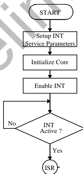
Figure 12-8 General Program Flowchart
