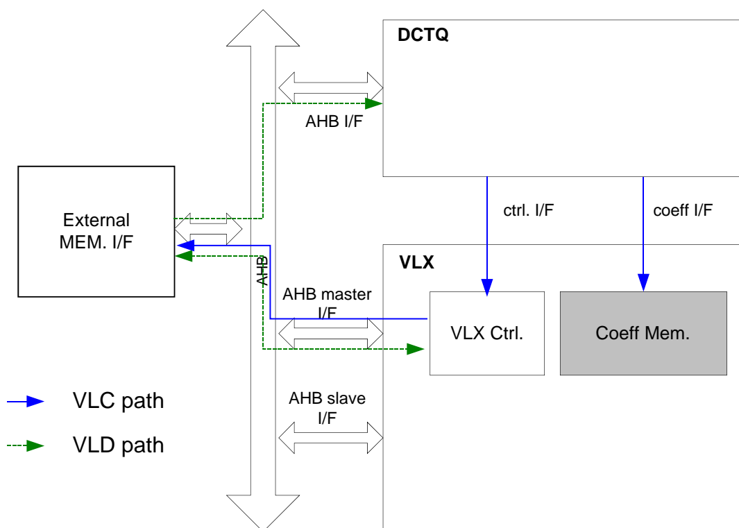
Figure 26-1 VLX top interface block diagram
