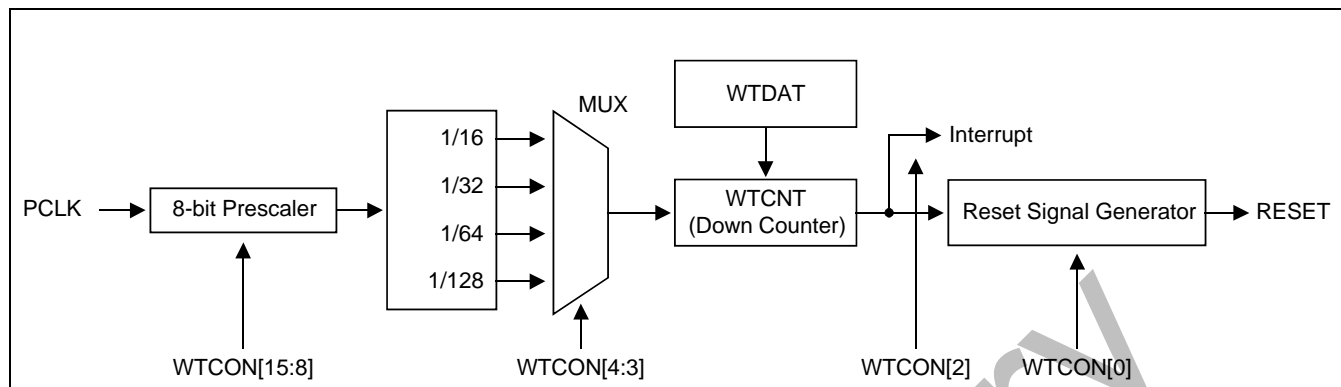
Figure 8-1. Watchdog Timer Block Diagram
