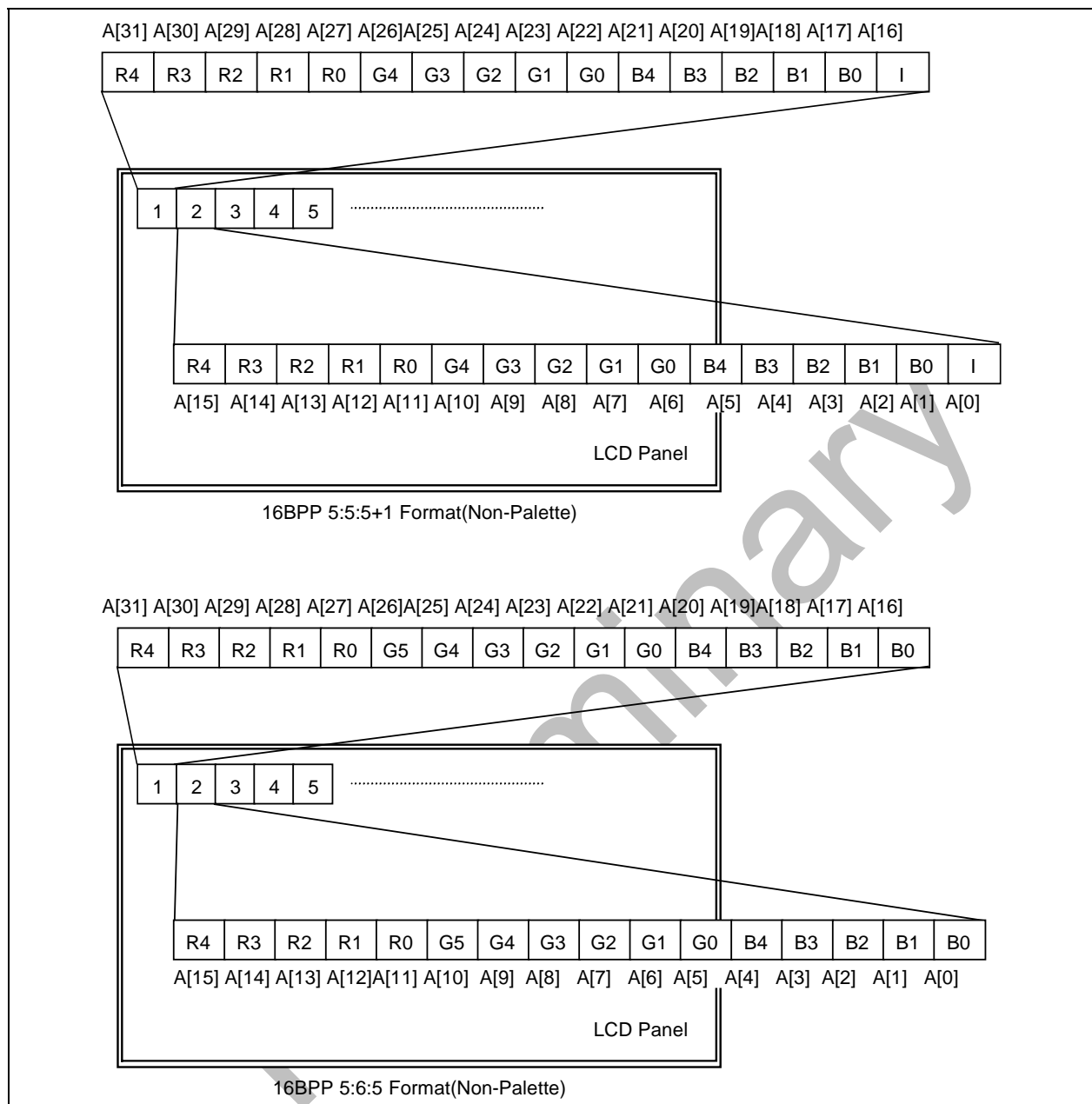
Figure 28-5. 16BPP Display Types
