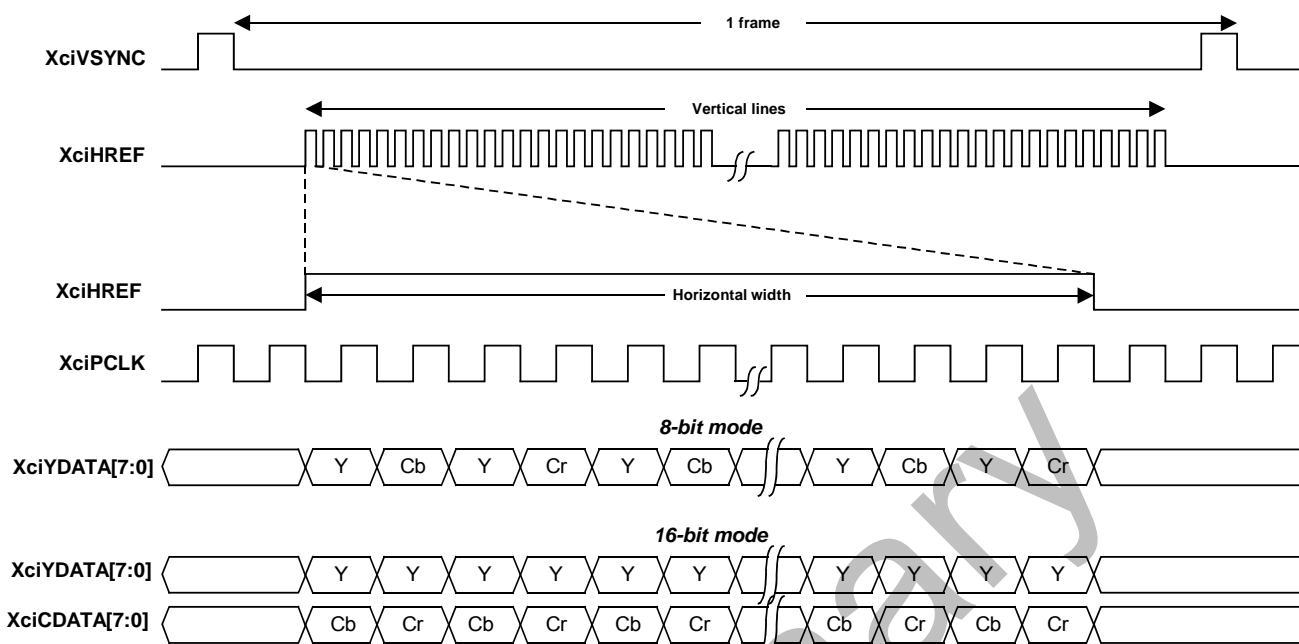
Figure 21-2. ITU-R BT 601 Input timing diagram
