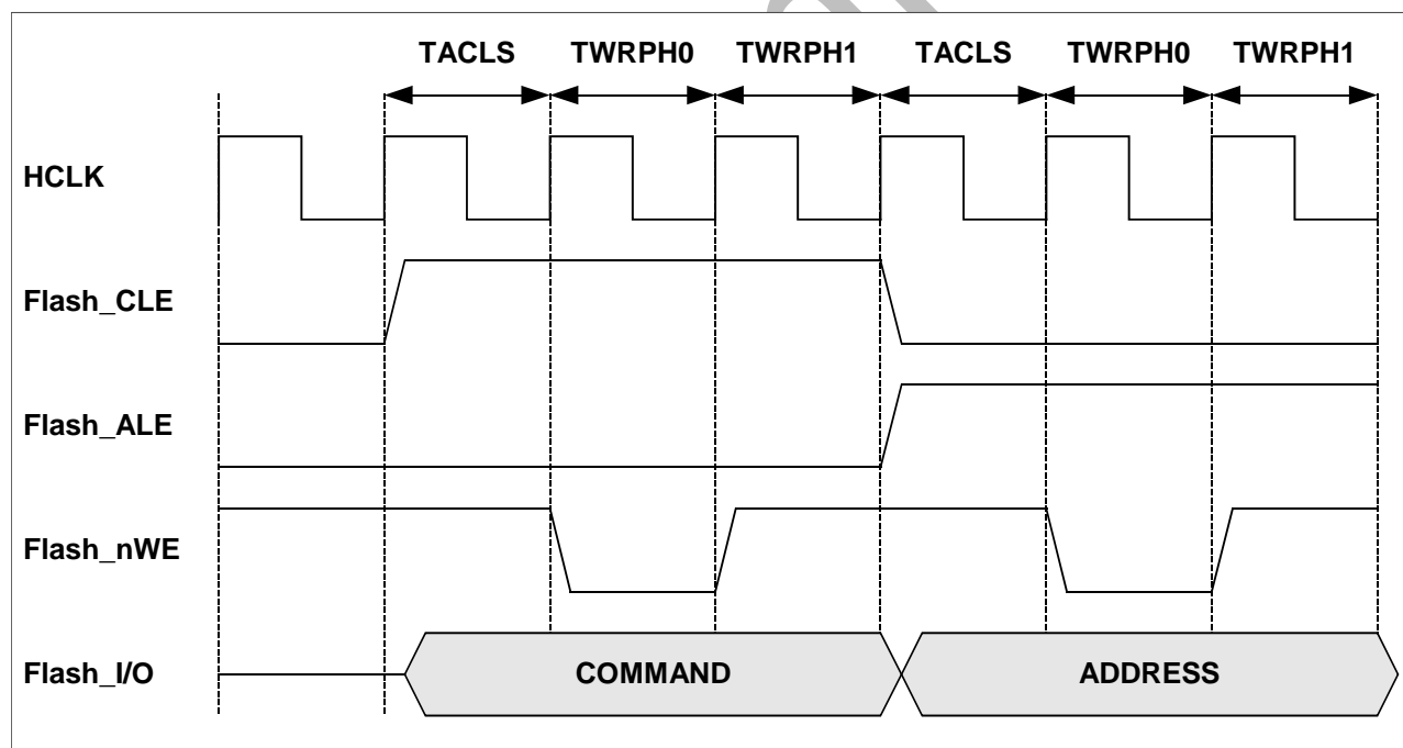
Figure 4-4 Auto Mode Timing Diagram (TACLS = 1, TWRPH0 = 0, TWRPH1 = 0)
