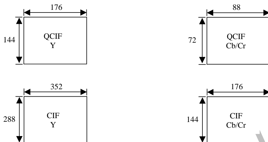
Figure 24-3. Y/Cb/Cr Configuration for QCIF/CIF Original Frame
