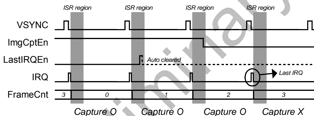
Figure 21-12. Timing diagram for last IRQ
