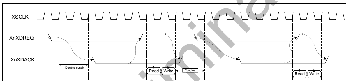
Figure 9-5. Single service, Handshake Mode, Single Transfer Size
