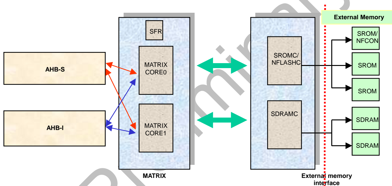
Figure 5-1 Configuration of MATRIX and Memory sub-system
