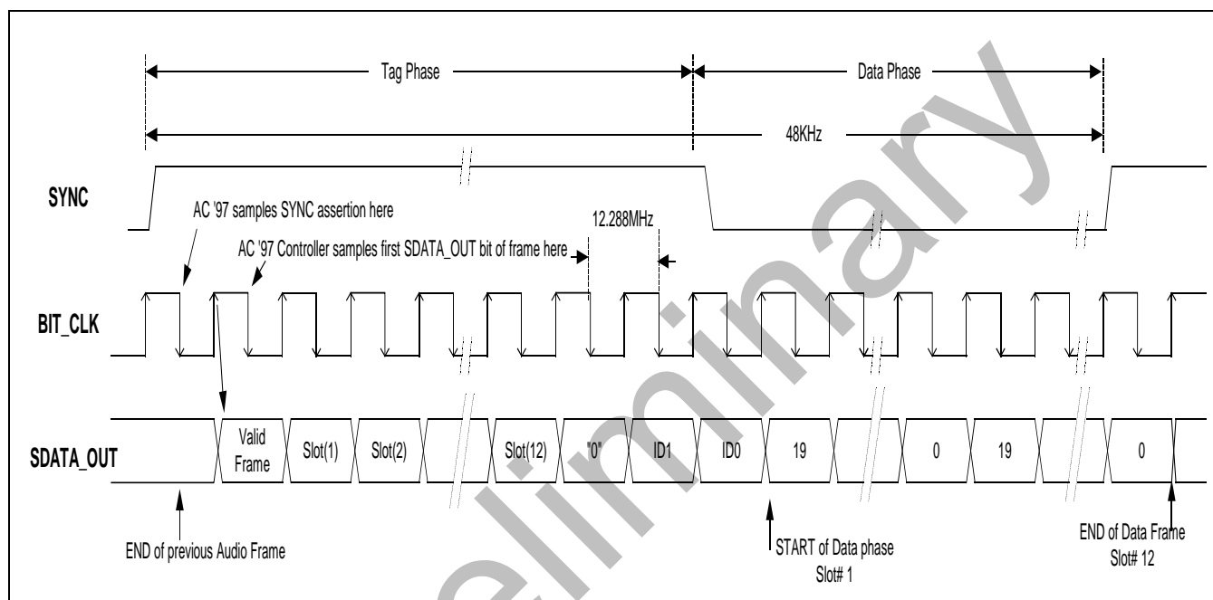
Figure 16-5. AC-link Output Frame
