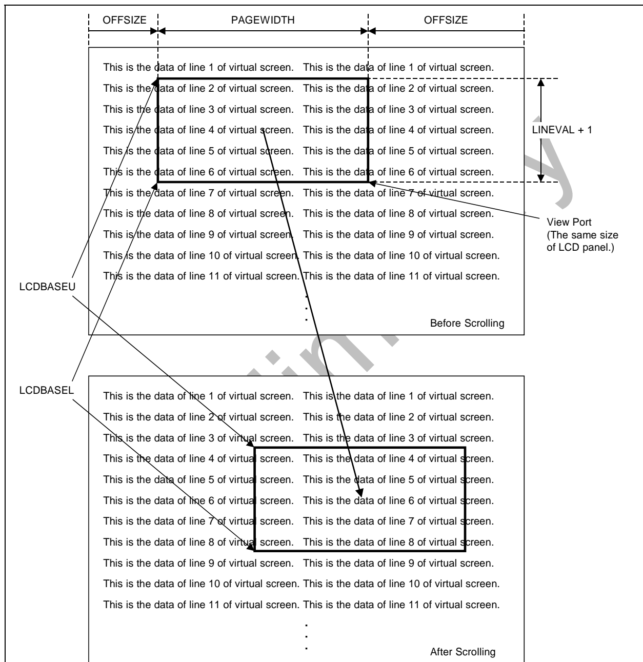
Figure 28-7. Example of Scrolling in Virtual Display
