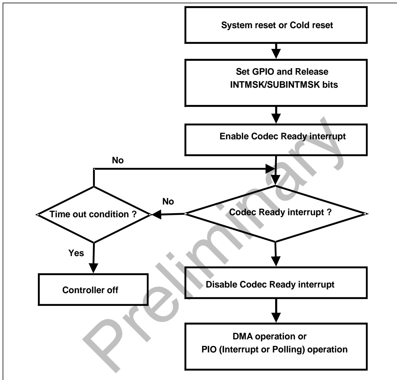
Figure 16-3. AC97 Operation Flow Chart
