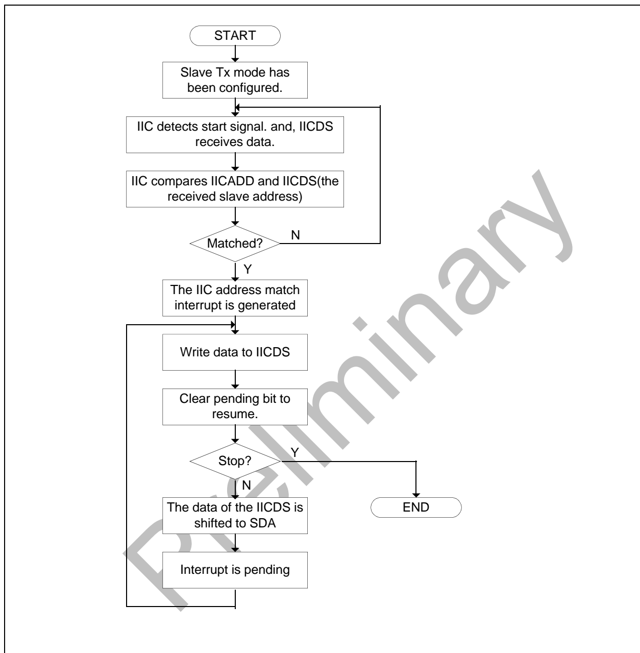
Figure 13-8 Operations for Slave / Transmitter Mode
