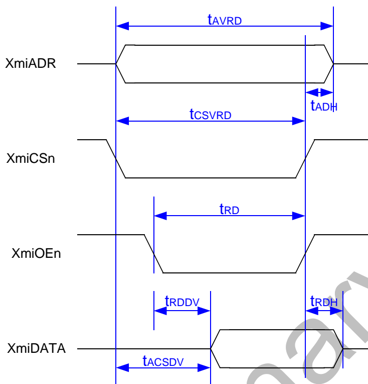
Figure 19-4 Modem interface read timing diagram
