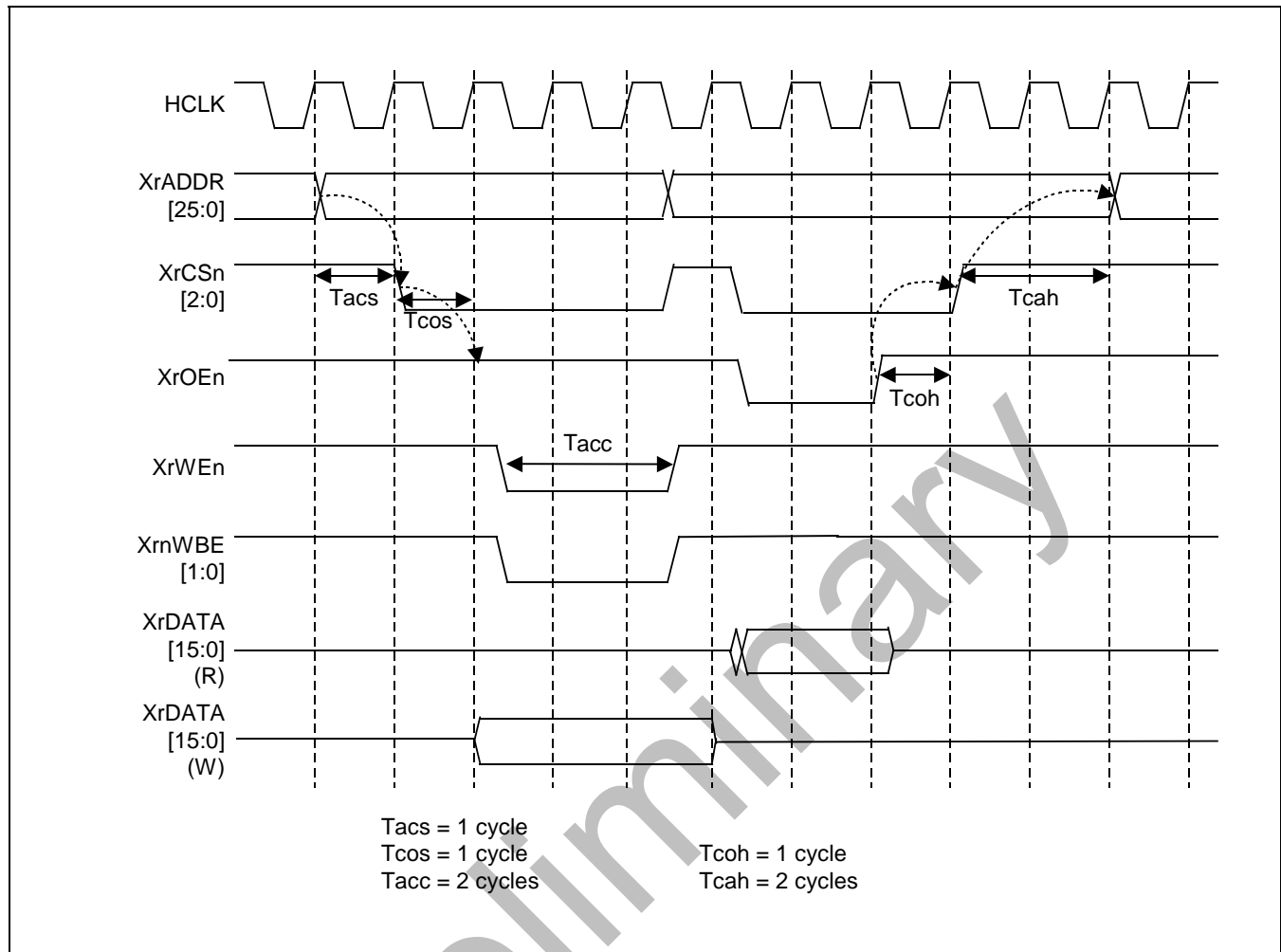
Figure 2-4 Programmable access cycle
