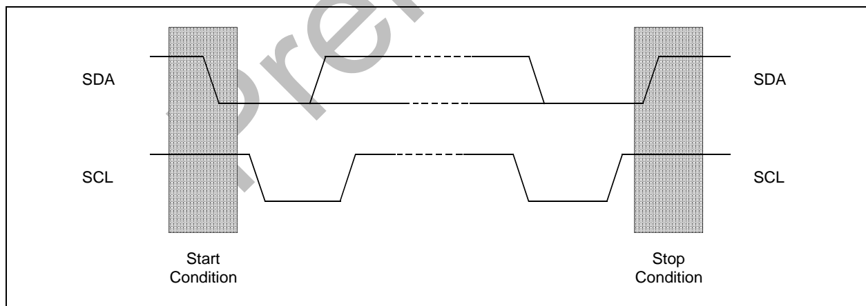
Figure 13-2. Start and Stop Condition
