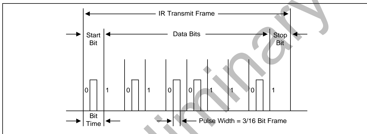
Figure 11-5. Infrared Transmit Mode Frame Timing Diagram
