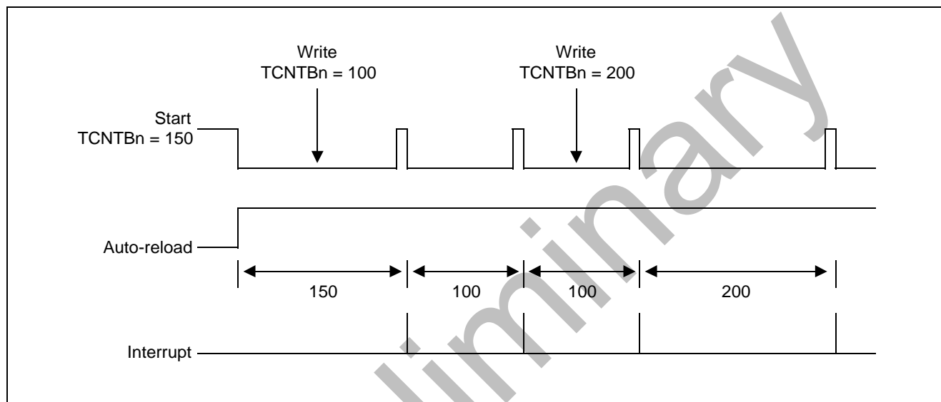
Figure 7-3. Example of Double Buffering Feature
