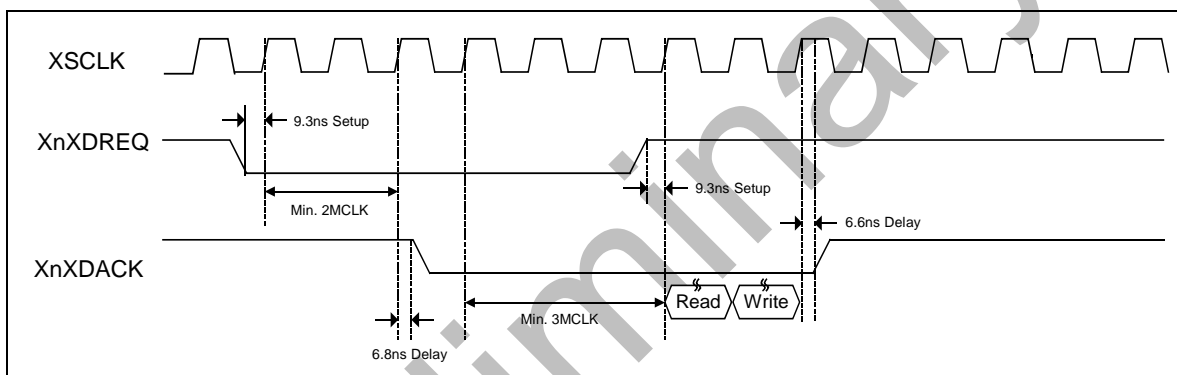
Figure 9-1. Basic DMA Timing Diagram
