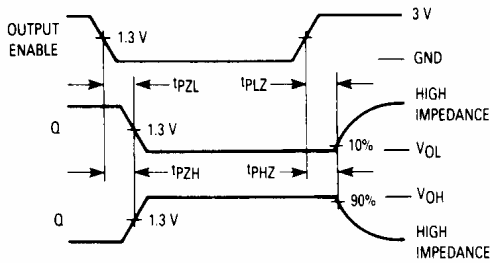
Figure 3. Switching Waveforms
