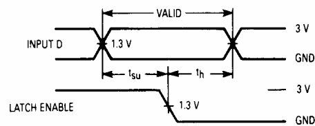
Figure 4. Switching Waveforms
