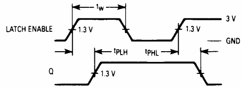
Figure 2. Switching Waveforms
