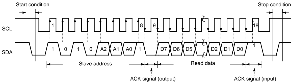
Fig.10 Current read cycle (BR24C01A / AF)
