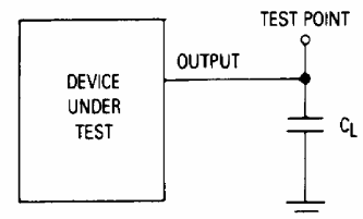
Figure 2. Test Circuit
