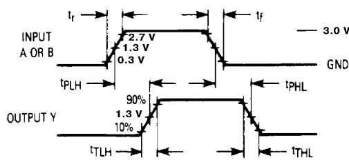
Figure 1 Switching Waveforms.
