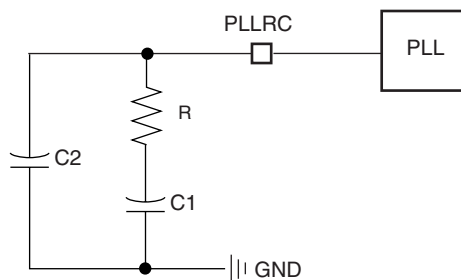
Figure 23-7. PLL Capacitors and Resistors
