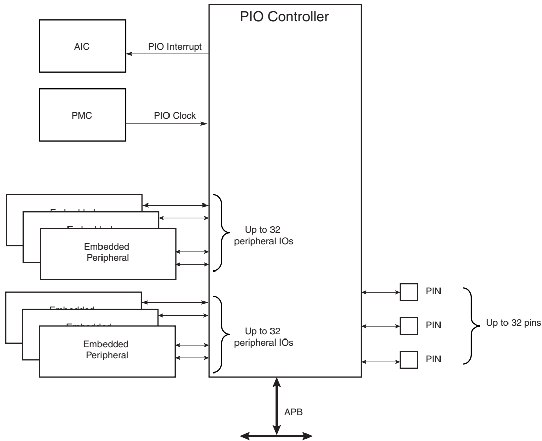
Figure 27-1. Block Diagram
