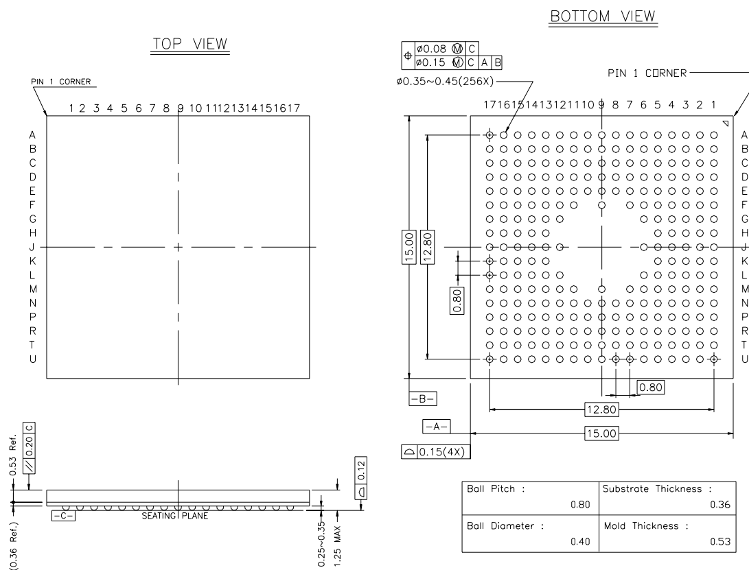
Figure 39-2. 256-ball BGA Package Drawing
