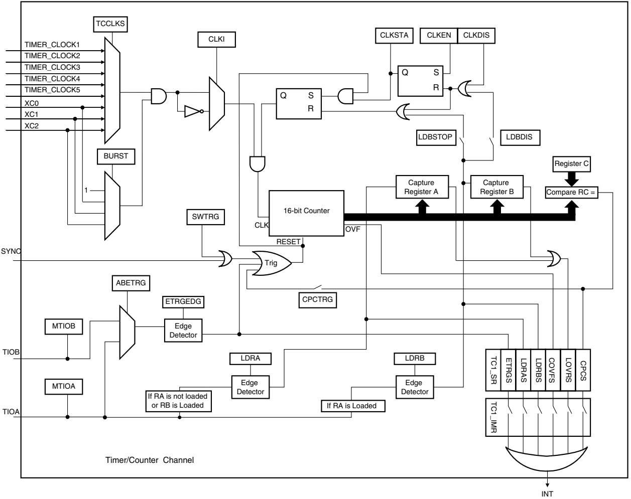
Figure 32-4. Capture Mode
