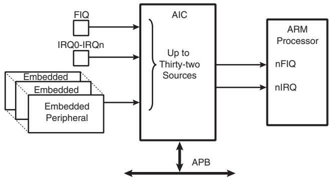
Figure 22-1. Block Diagram
