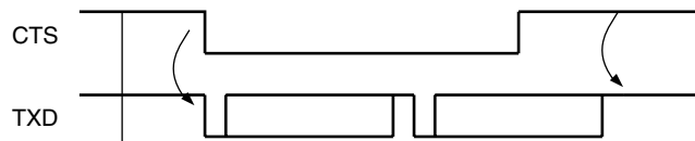
Figure 30-18. Transmitter Behavior when Operating with Hardware Handshaking
