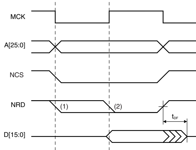
Figure 18-16. Data Float Output Delay
