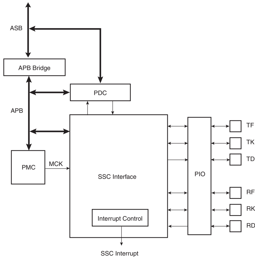
Figure 31-1. Block Diagram
