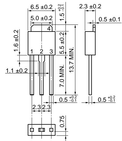
<R> TO-251 (MP-3)
