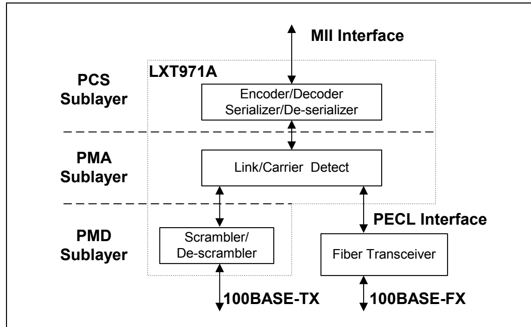
Figure 20. Protocol Sublayers
