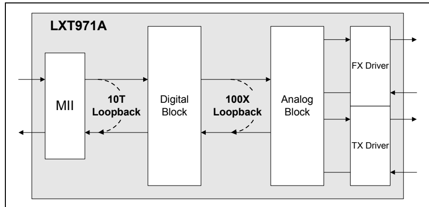
Figure 13. Loopback Paths
