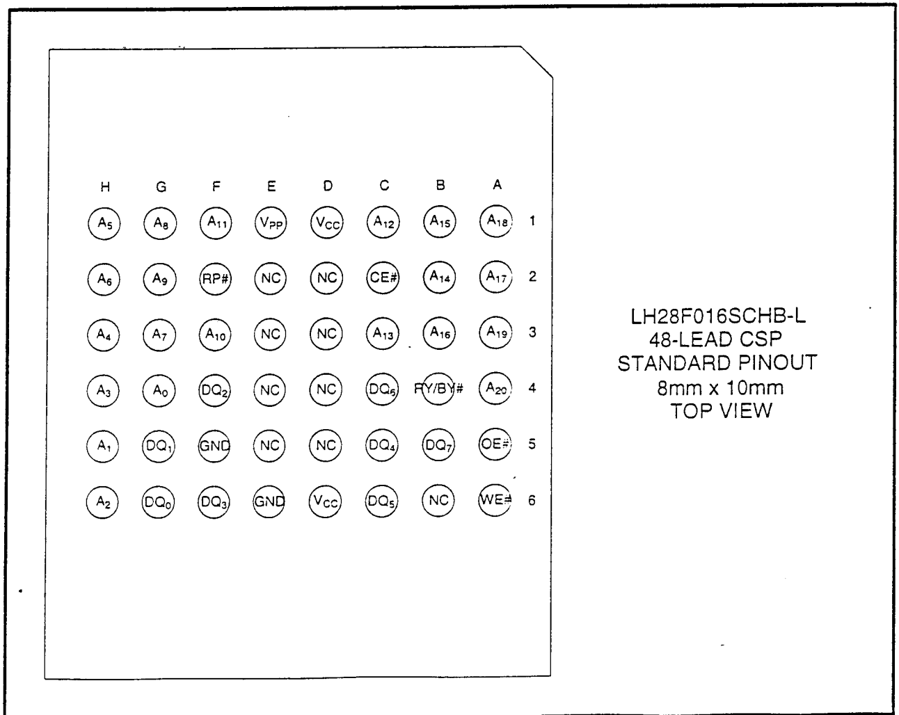
Figure 5. CSP 42-Lead Pinout
