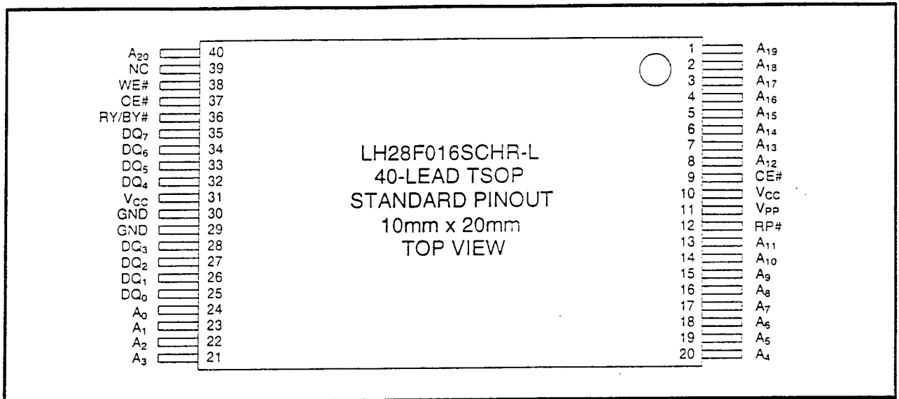
Figure 4. TSOP(Reverse Bend) 40-Lead Pinout
