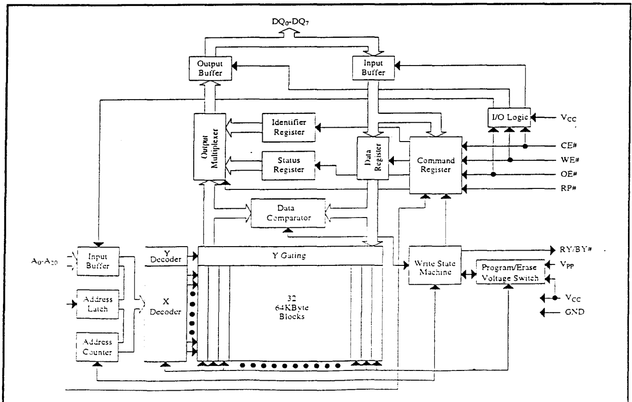
Figure 1. Block Diagram
