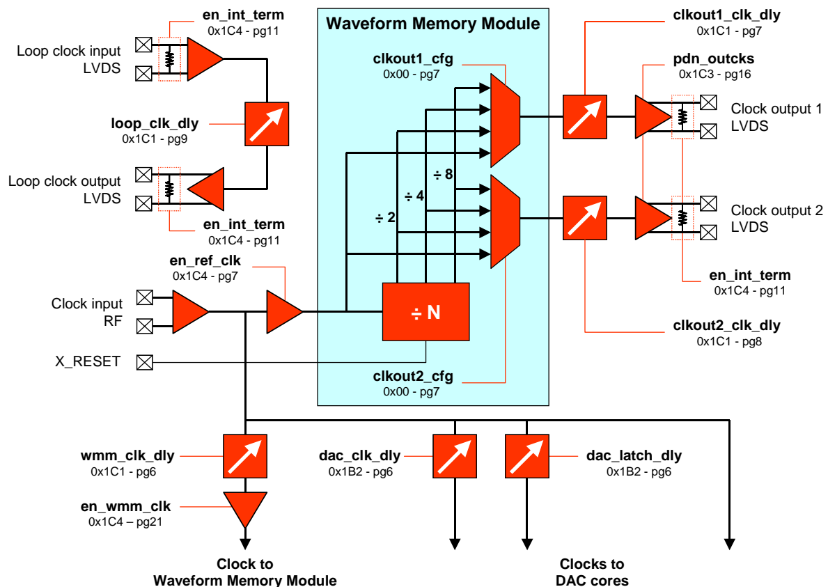
Figure 2 Clock Distribution
