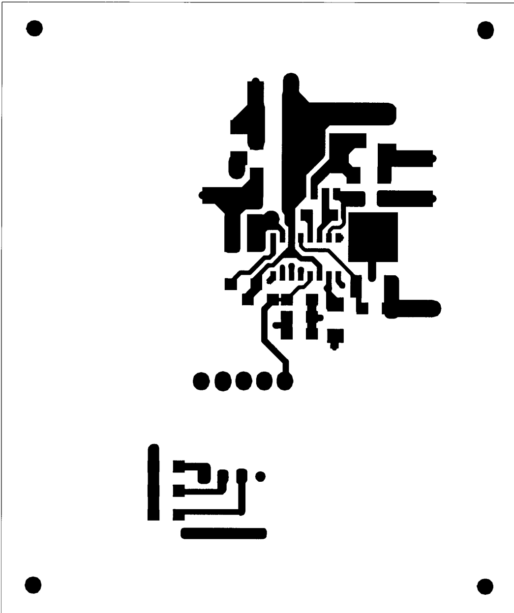
Figure 9. MAX722 EV Kit PC Layout (Component Layer, Component Side View, 2X Scale)
