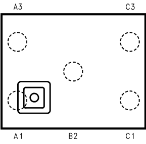
micro SMD, 5 Bump Package (BPA05, TPA05 & BLA05)
