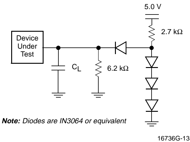
Figure 7. Test Setup
