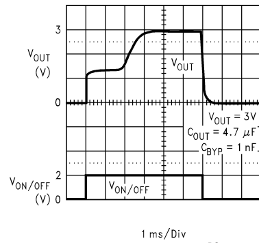
Turn-ON Waveform
