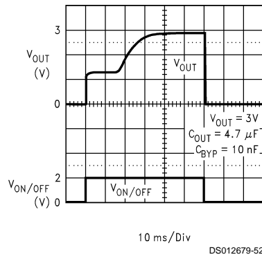
Turn-ON Waveform
