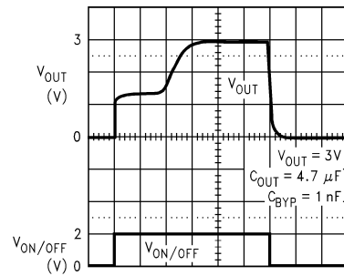
Turn-ON Waveform
