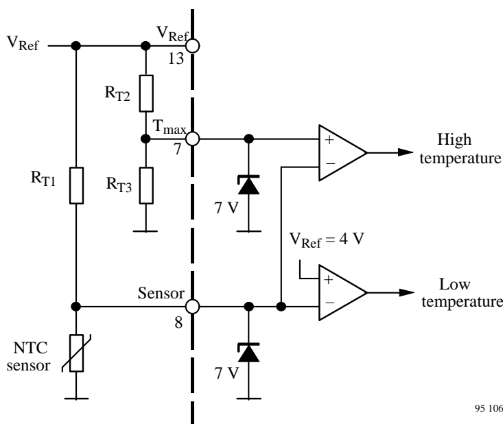
Figure 7. Temperature window
