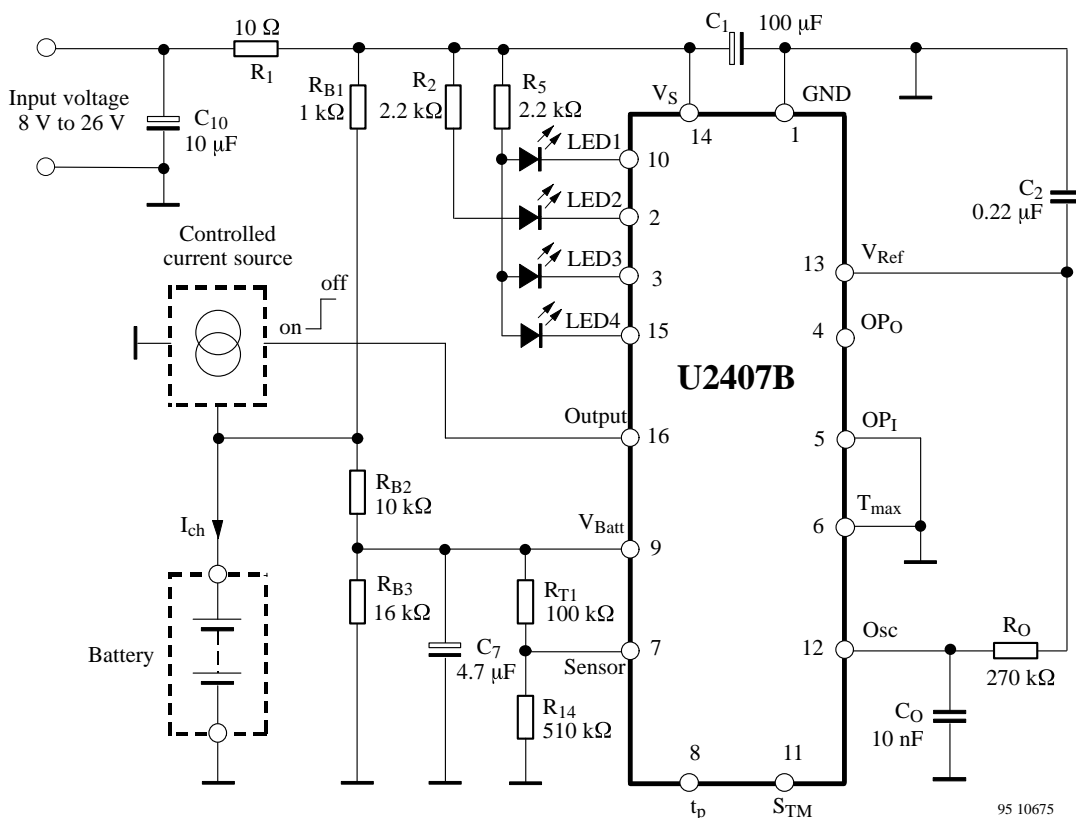
Figure 12. Minimum charge system with external current source
