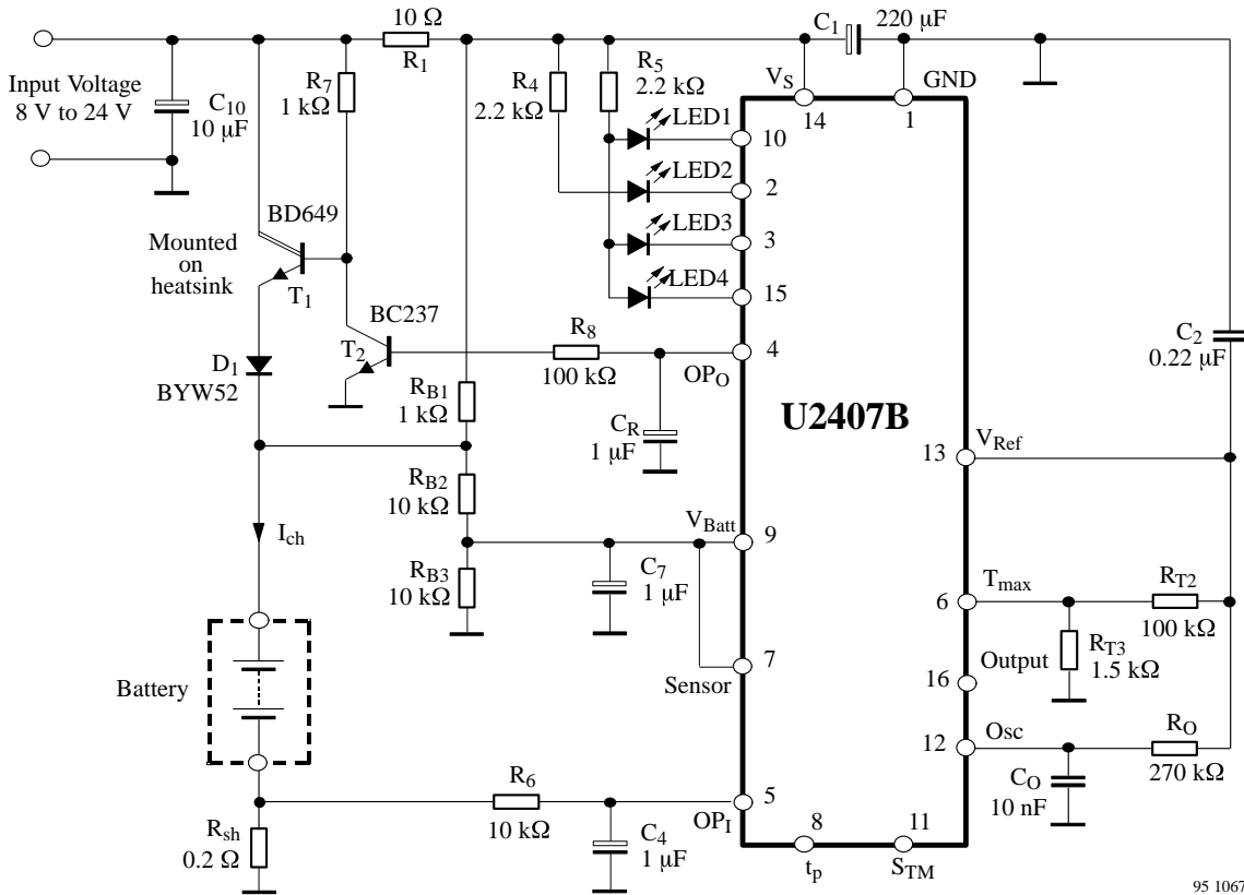
Figure 2. Scheme for DC linear regulation
