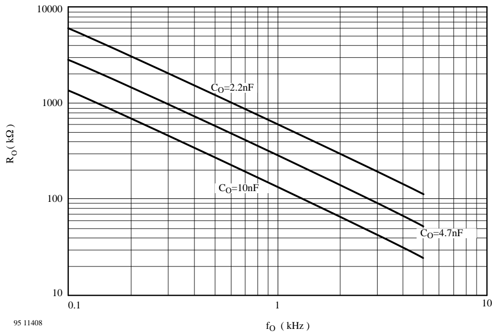
Figure 11. Frequency versus resistance for different capacitance values
