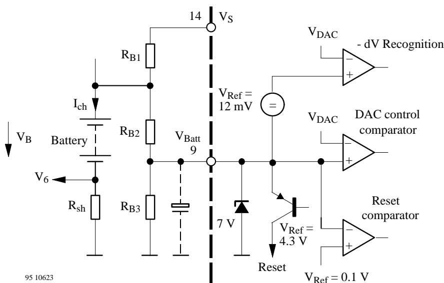
Figure 5. Input configuration for the battery voltage measurement
