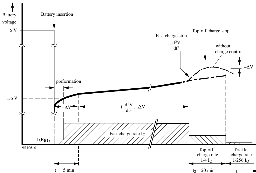
Figure 3. Charge function diagram, f_{osc} = 800 \text{ Hz}
