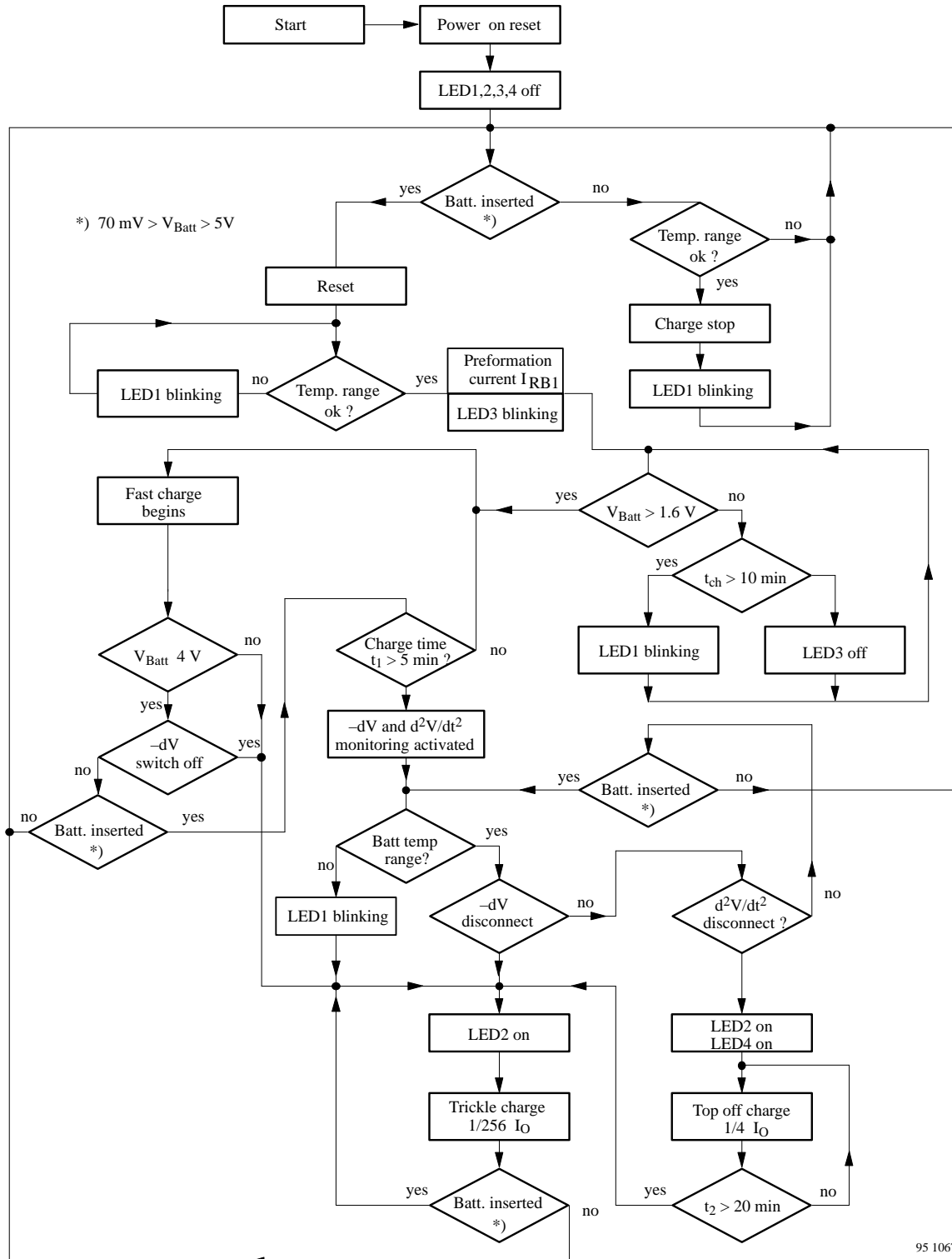
Figure 4. Flow chart
