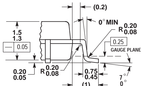
VIEW AA
