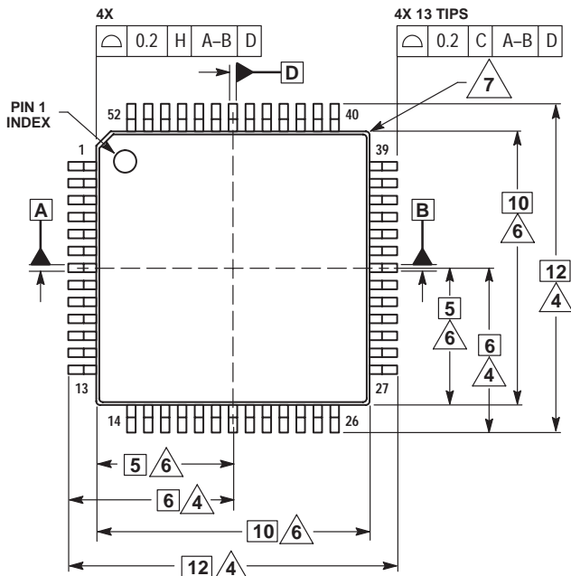
VIEW AA
