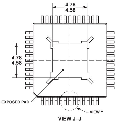
VIEW J-J
