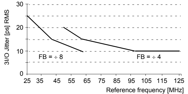
Figure 5. Maximum I/O Jitter versus frequency
