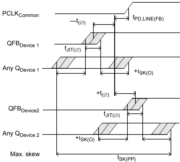
Figure 4. MPC9653A maximum device-to-device skew
