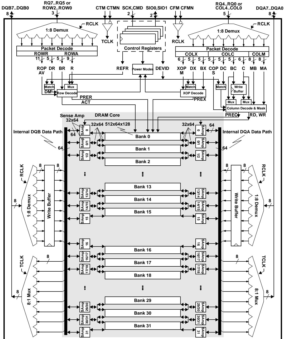
Figure 2: 128Mbit(256Kx16x32s) RDRAM Device Block Diagram
