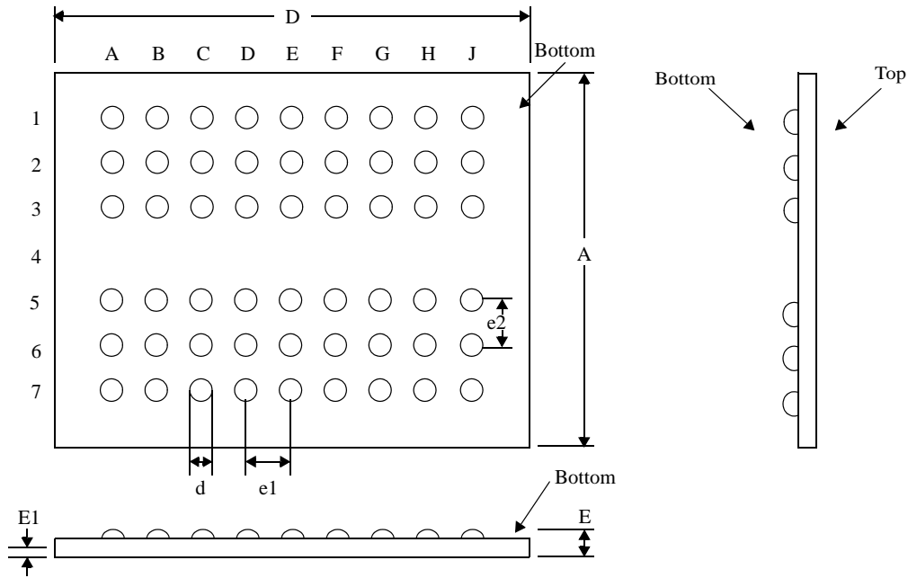
Figure 4: Center-Bonded fanout CSP Package
