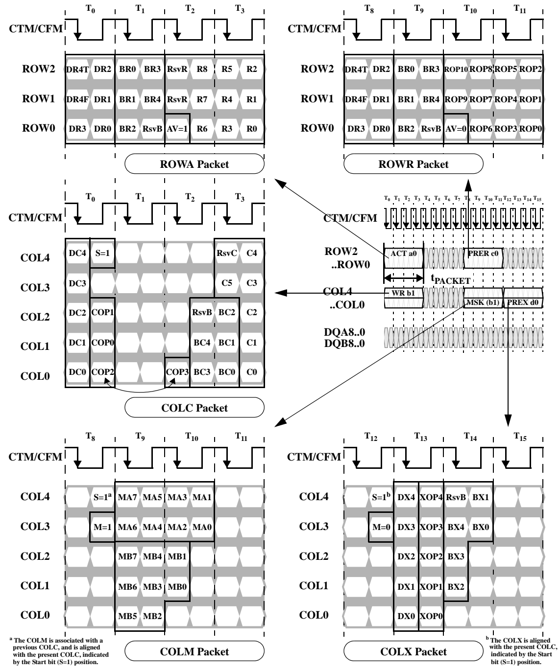
Figure 3: Packet Formats
