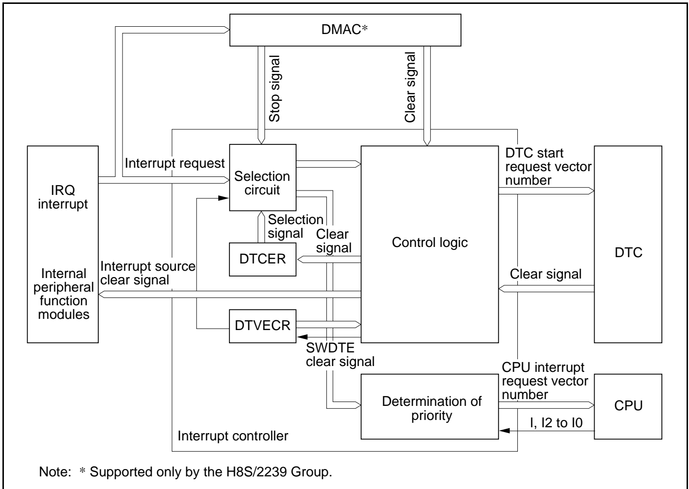
Figure 5.8 DTC and DMAC* Interrupt Control
