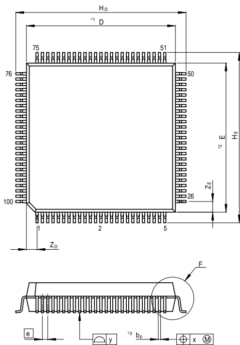
Figure C.4 FP-100B Package Dimensions
