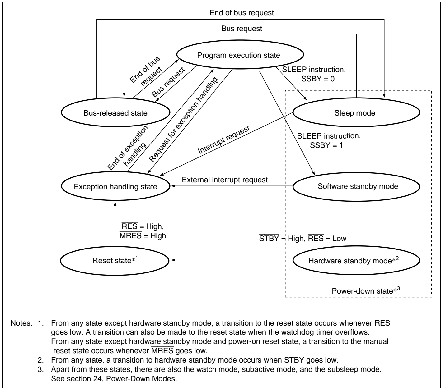
Figure 2.13 State Transitions
