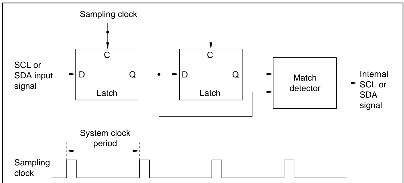
Figure 16.20 Block Diagram of Noise Canceler
