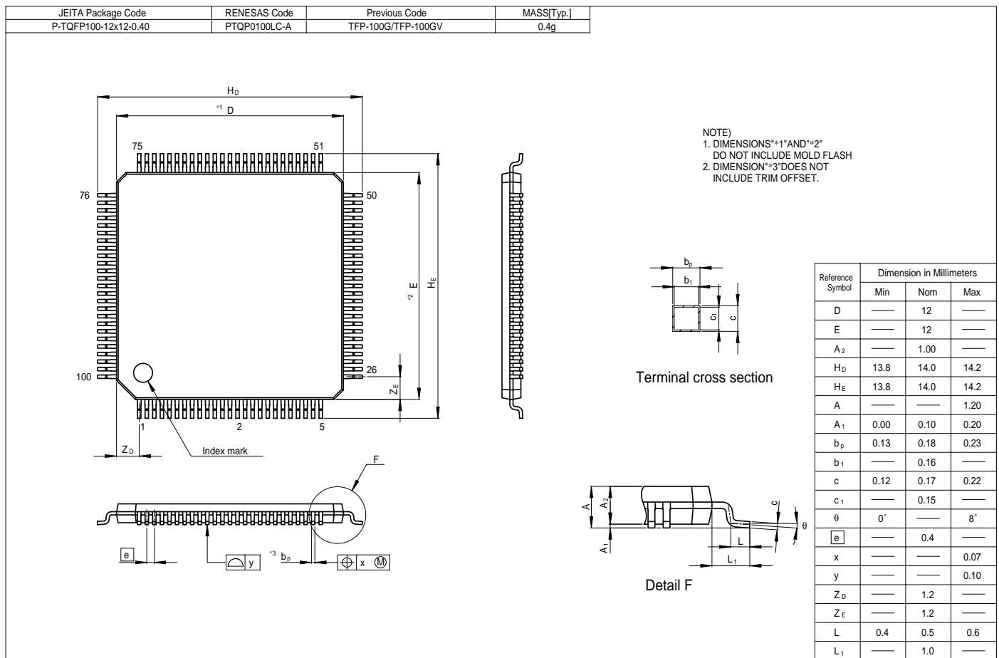
Figure C.2 TFP-100G Package Dimensions
