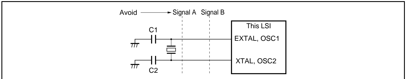
Figure 23.11 Note on Board Design of Oscillator Circuit
