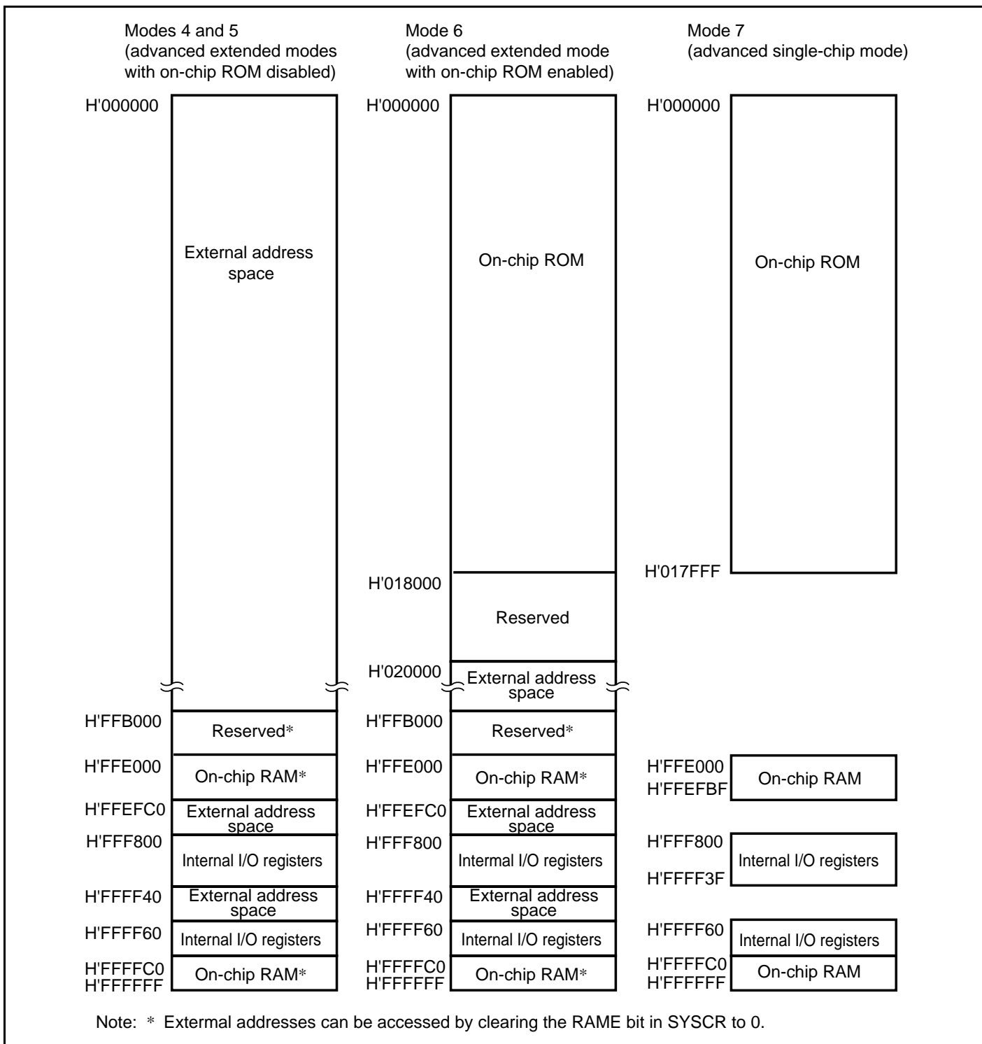
Figure 3.8 H8S/2224 Memory Map in Each Operating Mode
