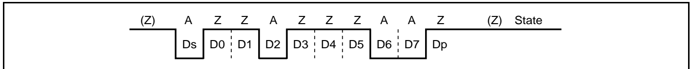
Figure 15.26 Direct Convention (SDIR = SINV = O/\bar{E} = 0 )
