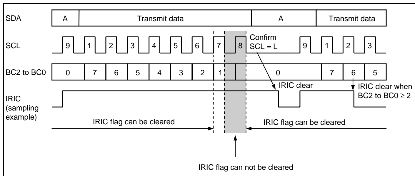
Figure 16.28 IRIC Flag Clearing Timing in Wait Operation
