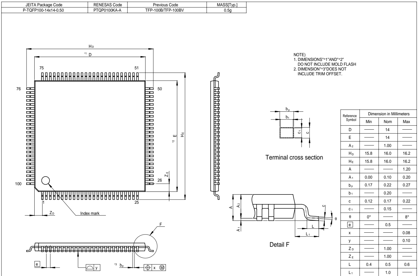
Figure C.1 TFP-100B Package Dimensions
