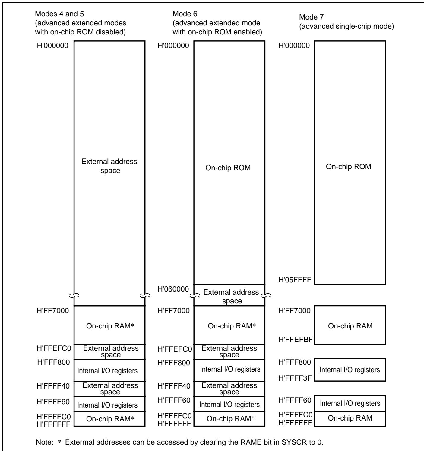
Figure 3.3 H8S/2239 Memory Map in Each Operating Mode
