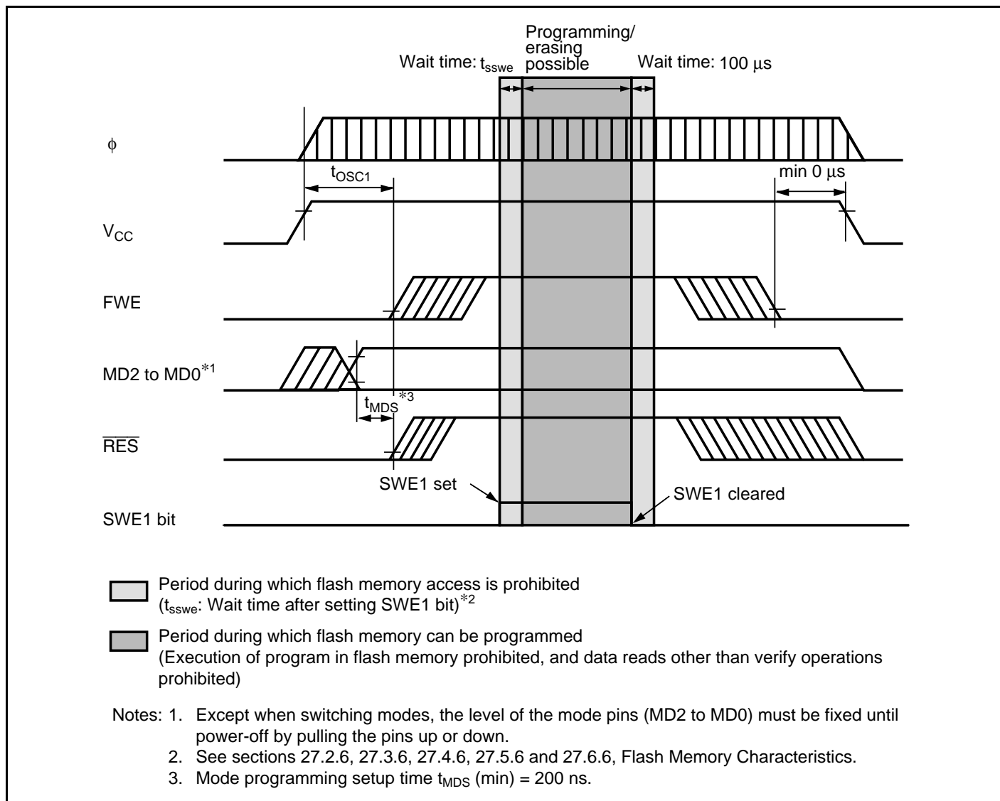
Figure 20.15 Power-On/Off Timing (User Program Mode)
