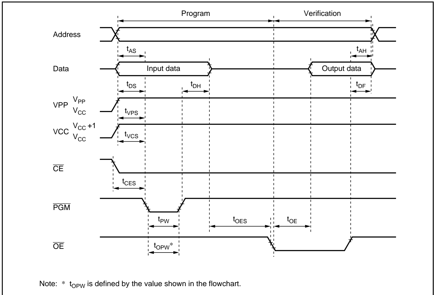
Figure 22.5 PROM Programming/Verification Timing
