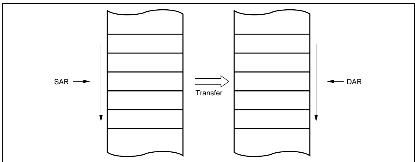
Figure 9.6 Memory Mapping in Normal Mode
