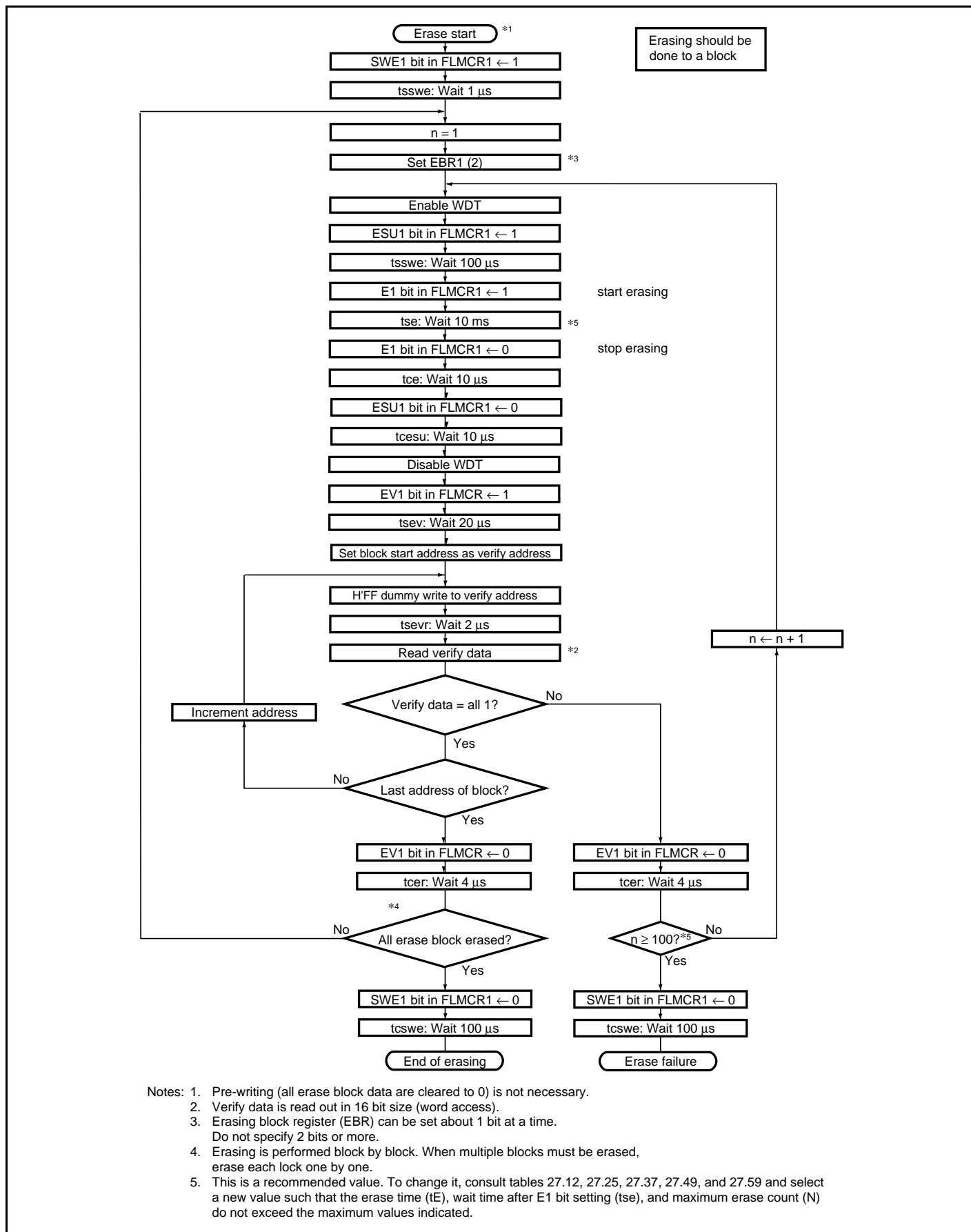
Figure 20.12 Erase/Eraser-Verify Flowchart
