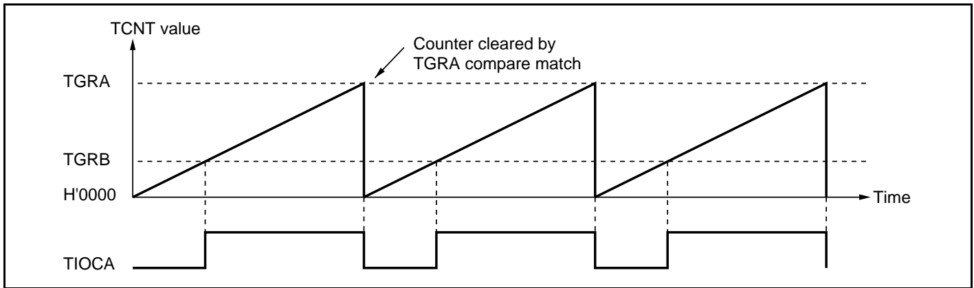
Figure 11.22 Example of PWM Mode Operation (1)
