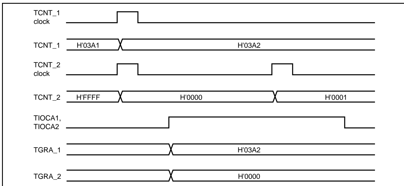
Figure 11.19 Example of Cascaded Operation (1)
