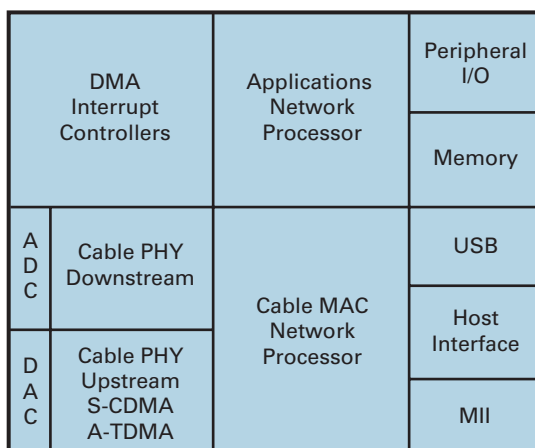
CX24951 Single-Chip Cable Modem IC Block Diagram
