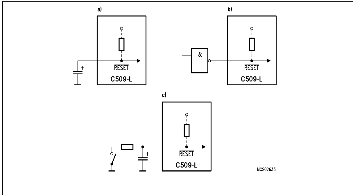
Figure 12 Reset Circuitries
