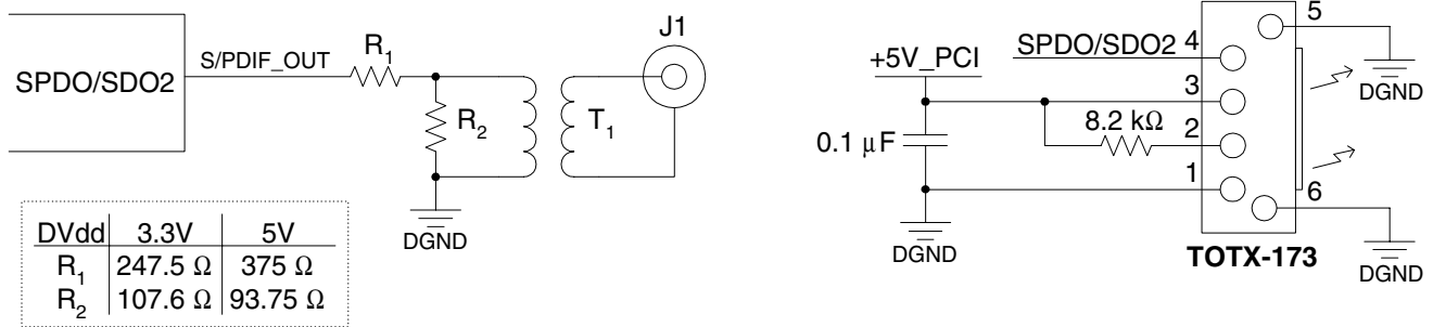
Figure 15. S/PDIF Output
