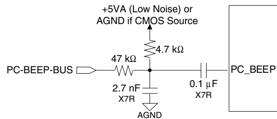
Figure 22. PC_BEEP Input
