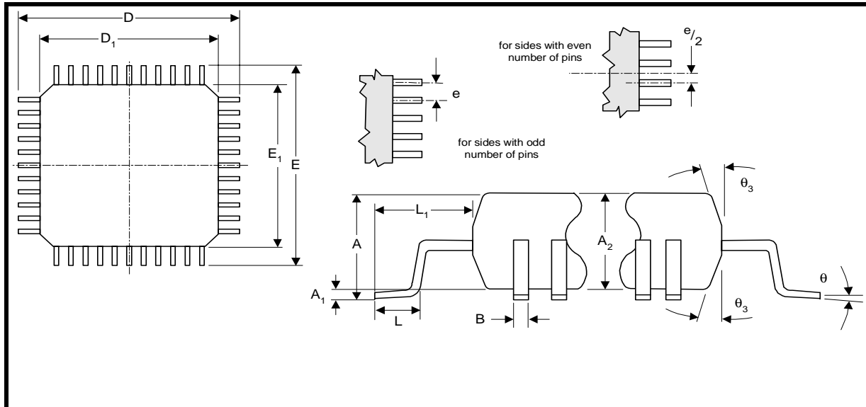
Figure 30. LXT6155LE Package Specification
