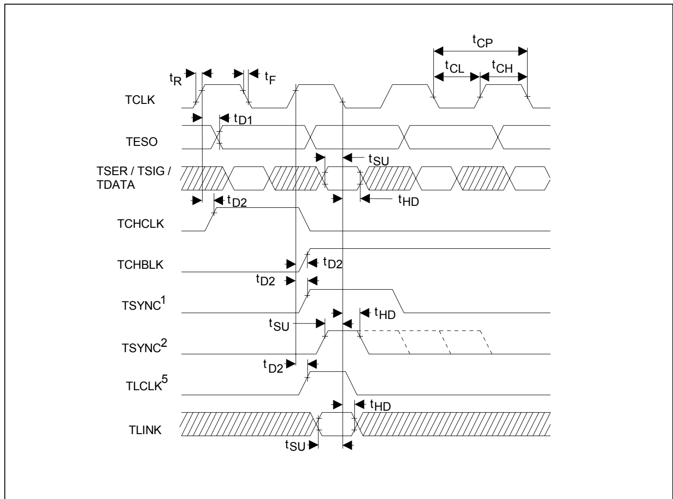
Figure 37-12. Transmit-Side Timing
