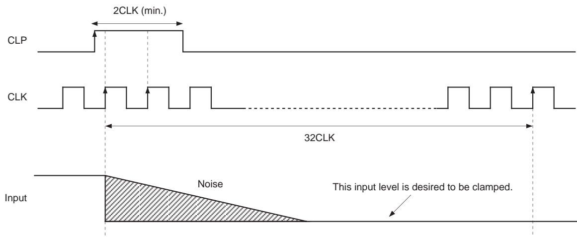
Timing III (When SEL=low)
