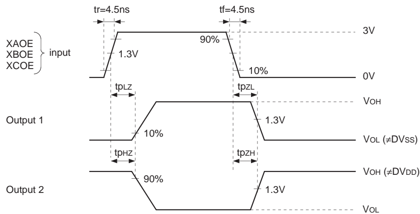
Timing Chart I-2.
