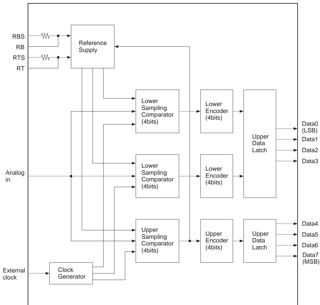
Fig. 1. 8-bit ADC block diagram
