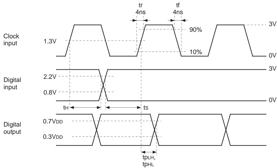
Timing Chart I-1.
