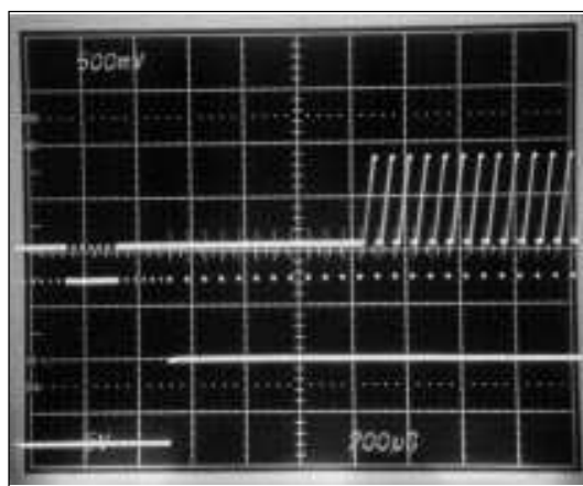
Timing III (When SEL=low)
