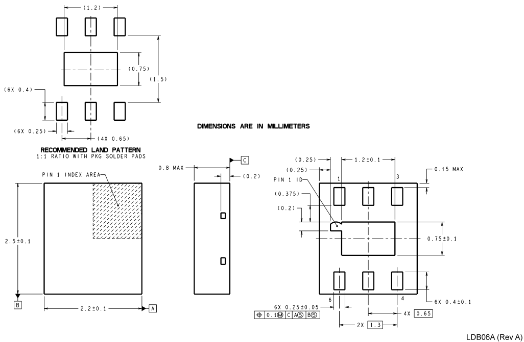
6-Lead LLP (NLDBB006) For Ordering, refer to Ordering Information table NS Package Number LDB06A
