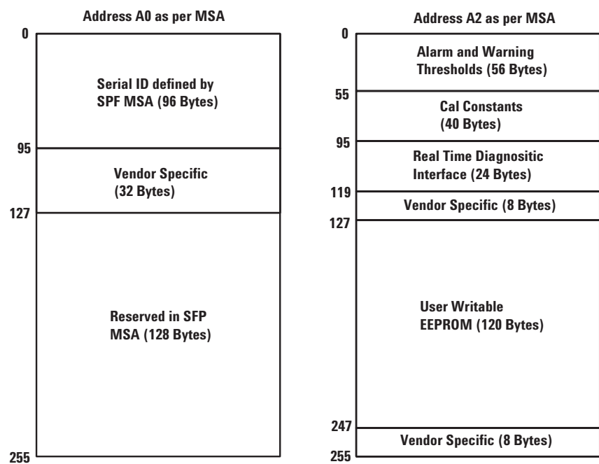
Figure 4. Memory Map
