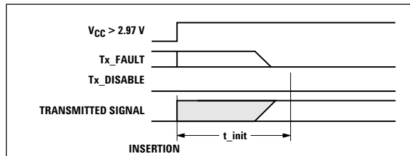
t_{\text{init}} : TX DISABLE NEGATED, MODULE HOT PLUGGED
