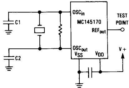
Figure 9. Test Circuit
