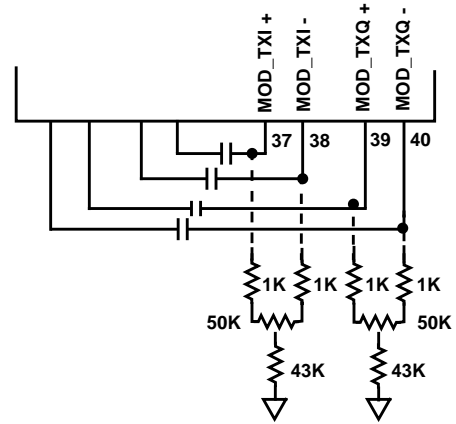
FIGURE 25. CARRIER NULL BIASING
