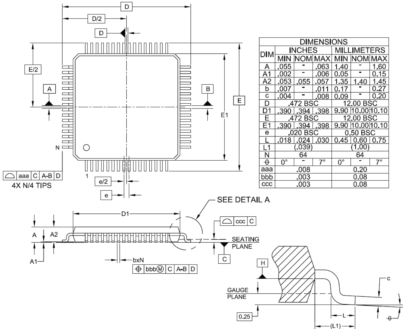
Figure 6 LQFP Package
