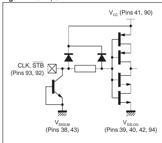
Figure 4. CLK, \overline{STB}
