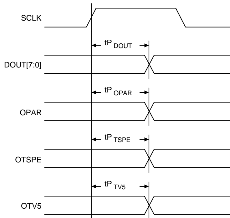
Figure 22 - Output Timing
