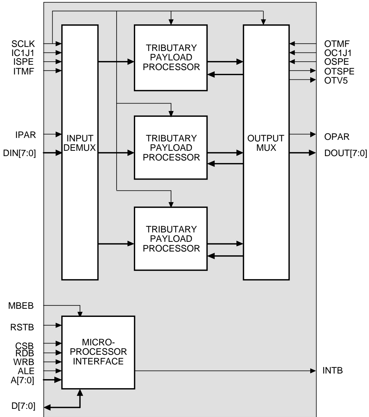
Figure 2 - Overall Device
