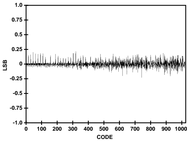
FIGURE 4. DIFFERENTIAL LINEARITY
