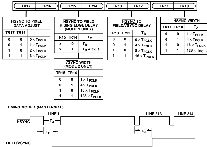
Figure 44. Timing Register 1
