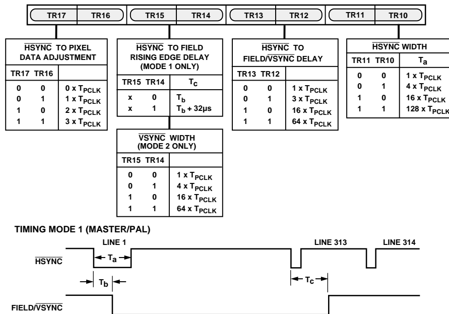
Figure 37. Timing Register 1
