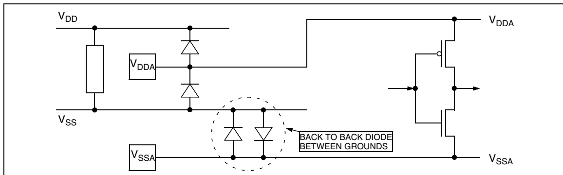
Figure 80. Multisupply Configuration
