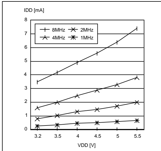
Figure 62. Typical I_{DD} in RUN vs. f_{CPU}
