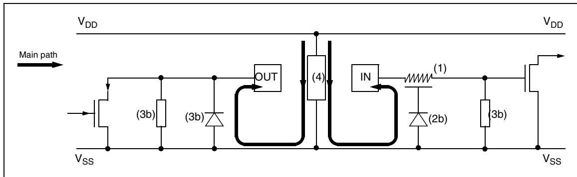
Figure 80. Multisupply Configuration
