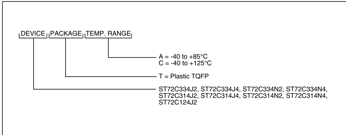
Figure 102. Flash User Programmable Device Types
