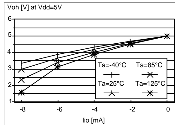
Figure 85. Typical V_{OH} at V_{DD}=5V
