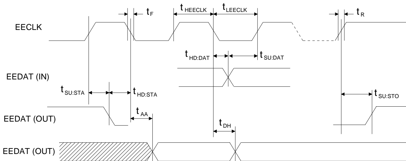
Figure 5. EEPROM Timing
