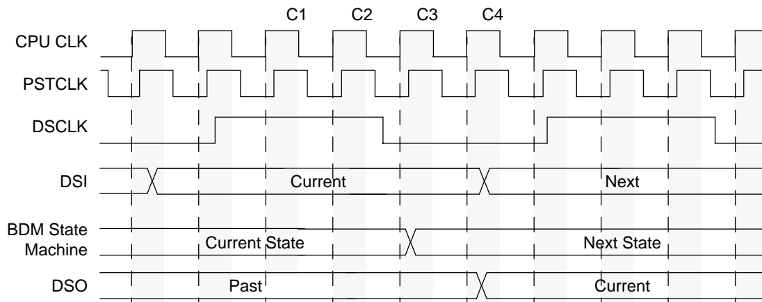
Figure 5-13. BDM Serial Interface Timing
