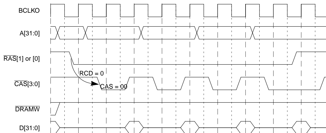
Figure 11-11. EDO Read Operation (3-2-2-2)
