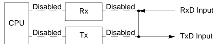
Figure 14-25. Remote Loop-Back
