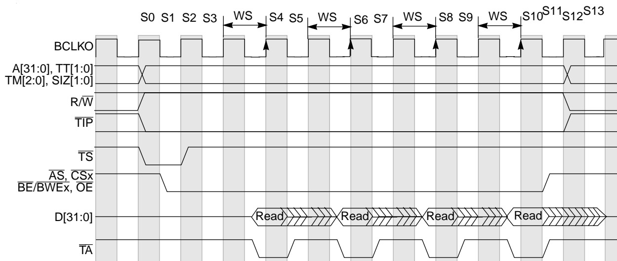
Figure 18-14. Line Read Burst (3-2-2-2), External Termination
