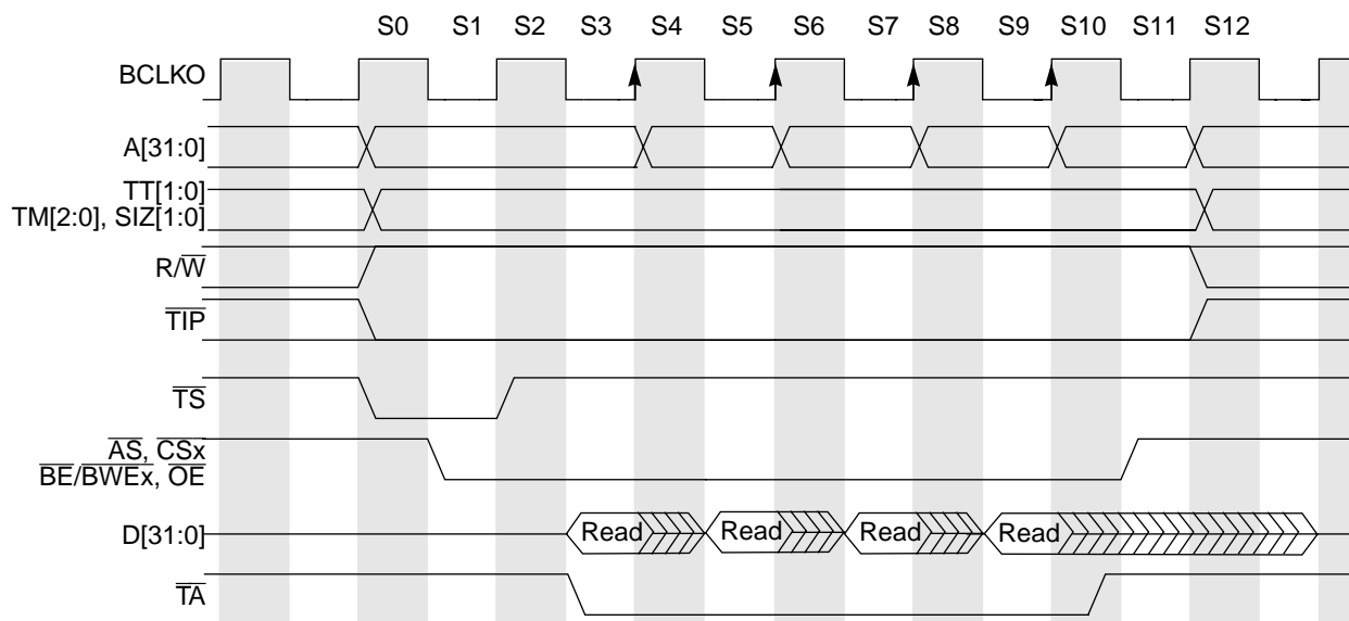
Figure 18-13. Line Read Burst (2-1-1-1), Internal Termination
