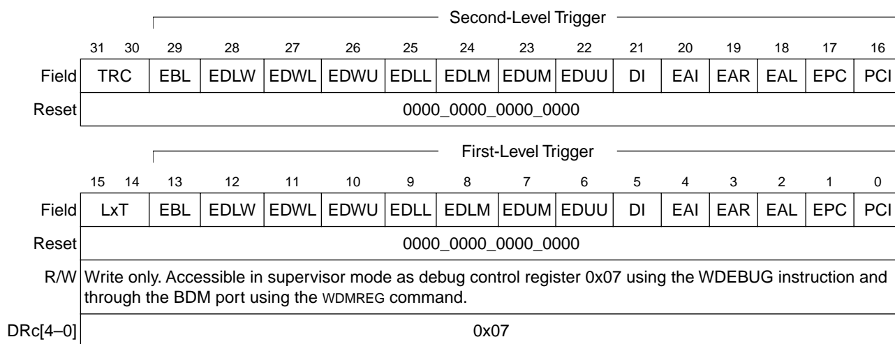
Figure 5-12. Trigger Definition Register (TDR)
