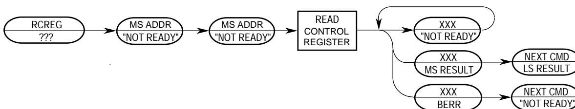
Figure 5-37. RCREG Command Sequence
