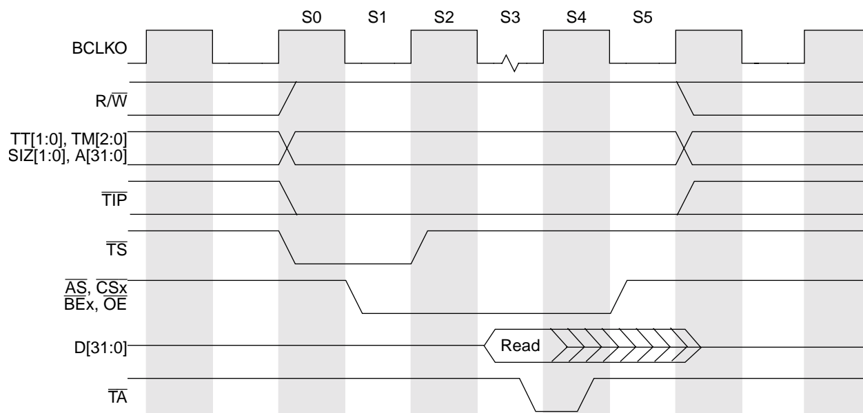
Figure 18-6. Basic Read Bus Cycle
