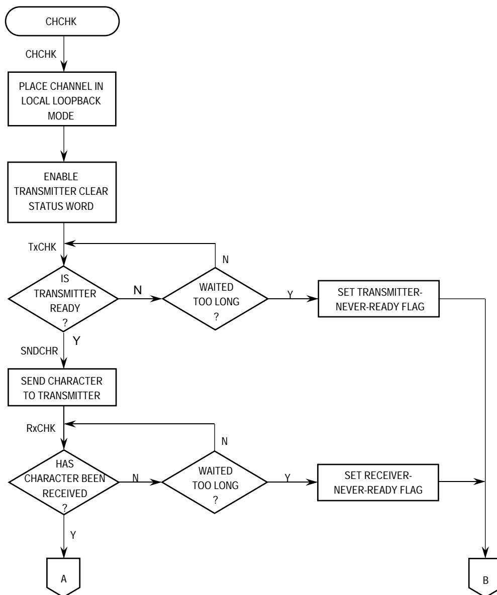
Figure 14-27. UART Mode Programming Flowchart (Sheet 2 of 5)
