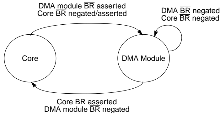
Figure 6-12. Park on DMA Module Priority (PARK = 10)
