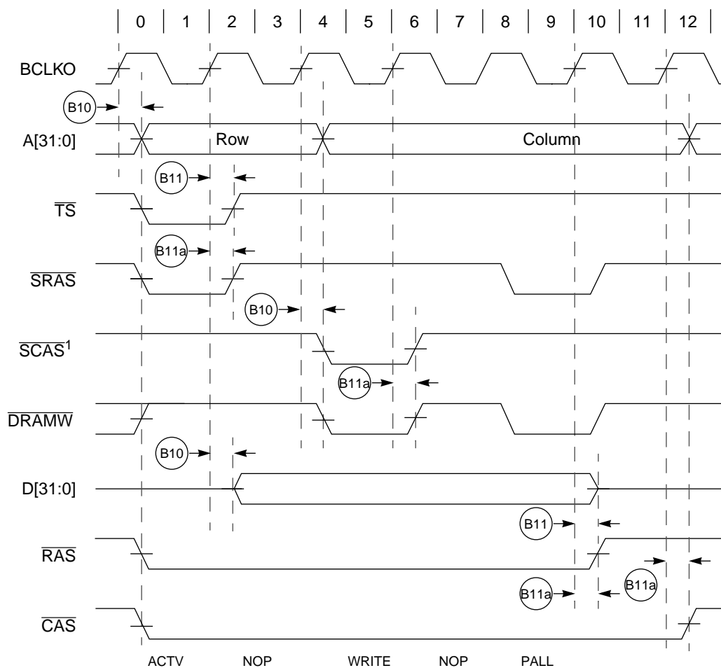
Figure 20-7. SDRAM Write Cycle with EDGESEL Tied High
