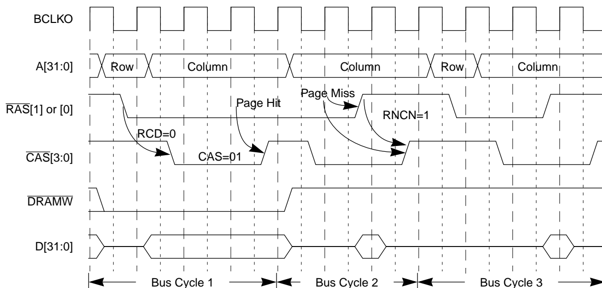
Figure 11-9. Continuous Page-Mode Operation
