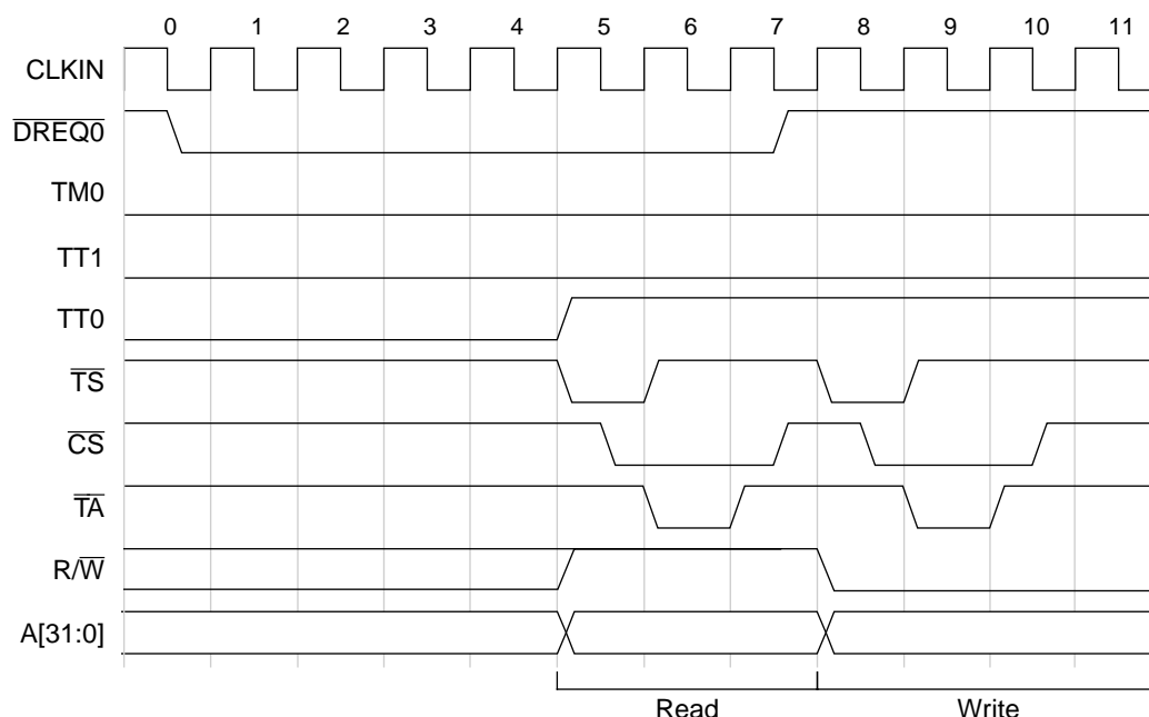
Figure 12-11. \overline{\text{DREQ}} Timing Constraints, Dual-Address DMA Transfer
