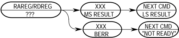
Figure 5-19. RAREG/RDREG Command Sequence
