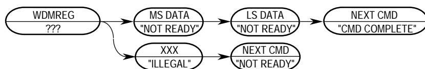
Figure 5-43. WDMREG Command Sequence
