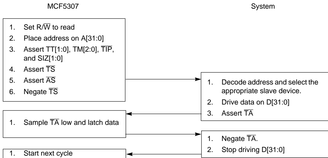
Figure 18-5. Read Cycle Flowchart
