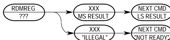
Figure 5-41. RDMREG Command Sequence
