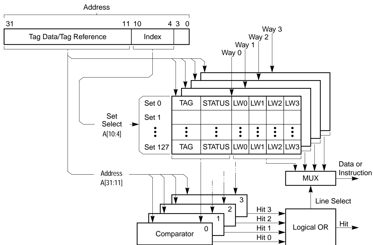
Figure 4-5. Caching Operation
