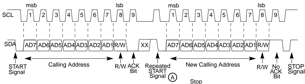
Figure 8-3. Repeated START
