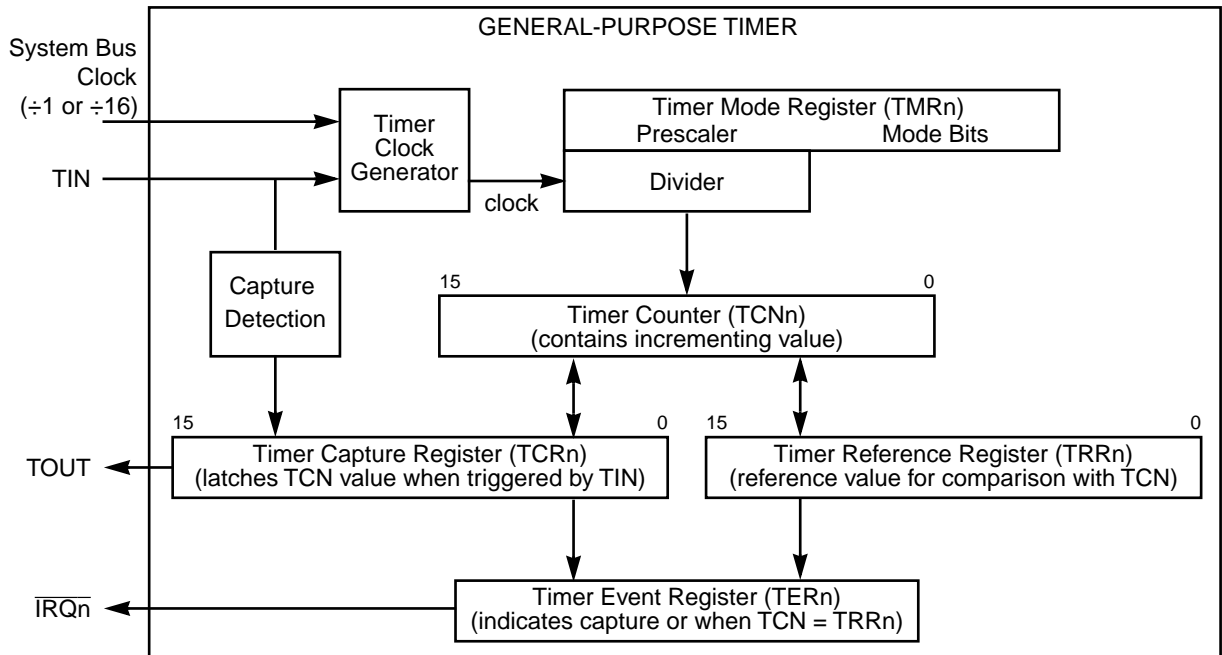
Figure 13-1. Timer Block Diagram
