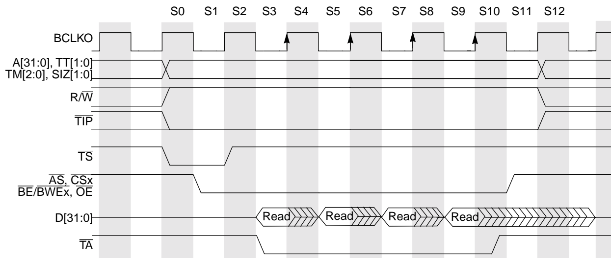
Figure 18-12. Line Read Burst (2-1-1-1), External Termination
