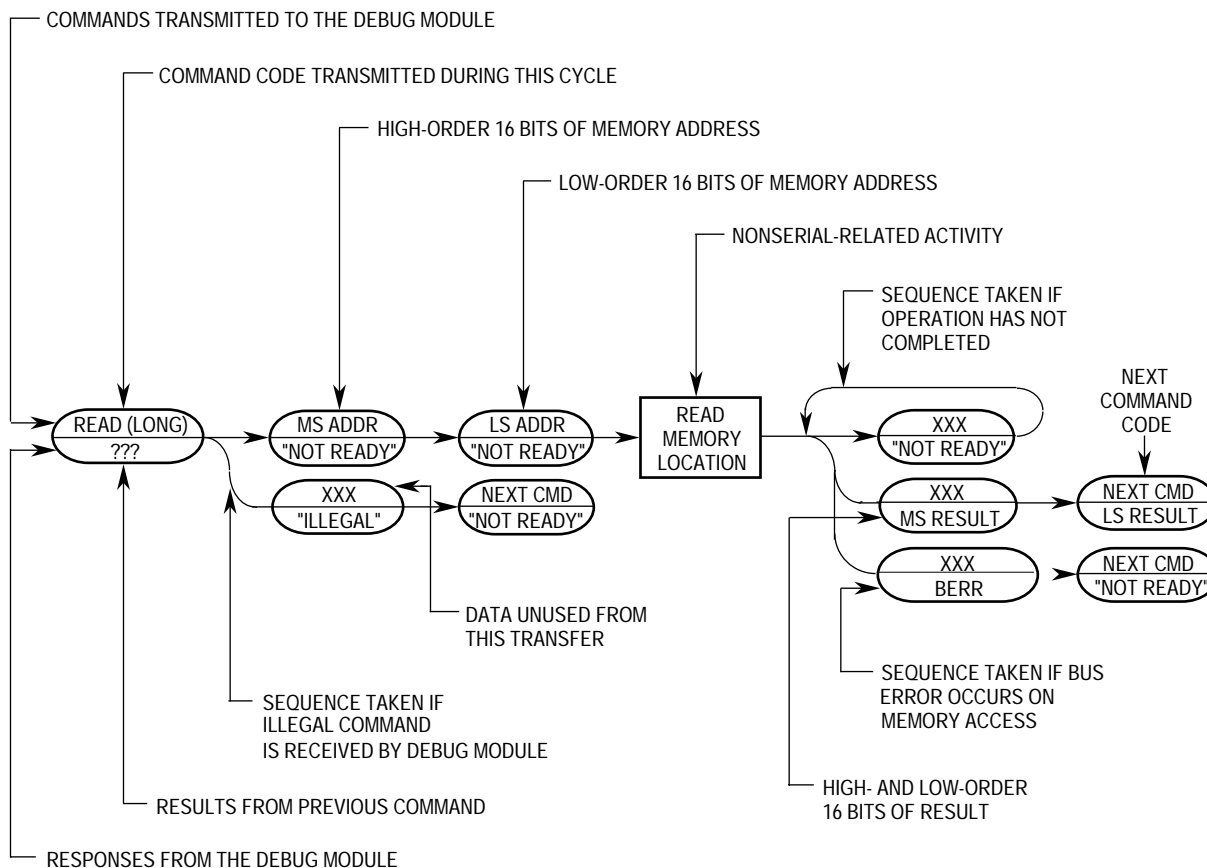
Figure 5-17. Command Sequence Diagram
