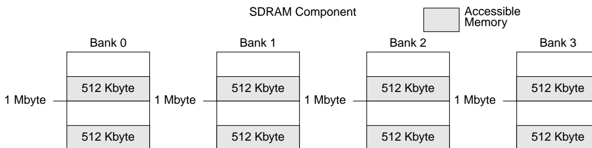
Figure 11-26. SDRAM Configuration
