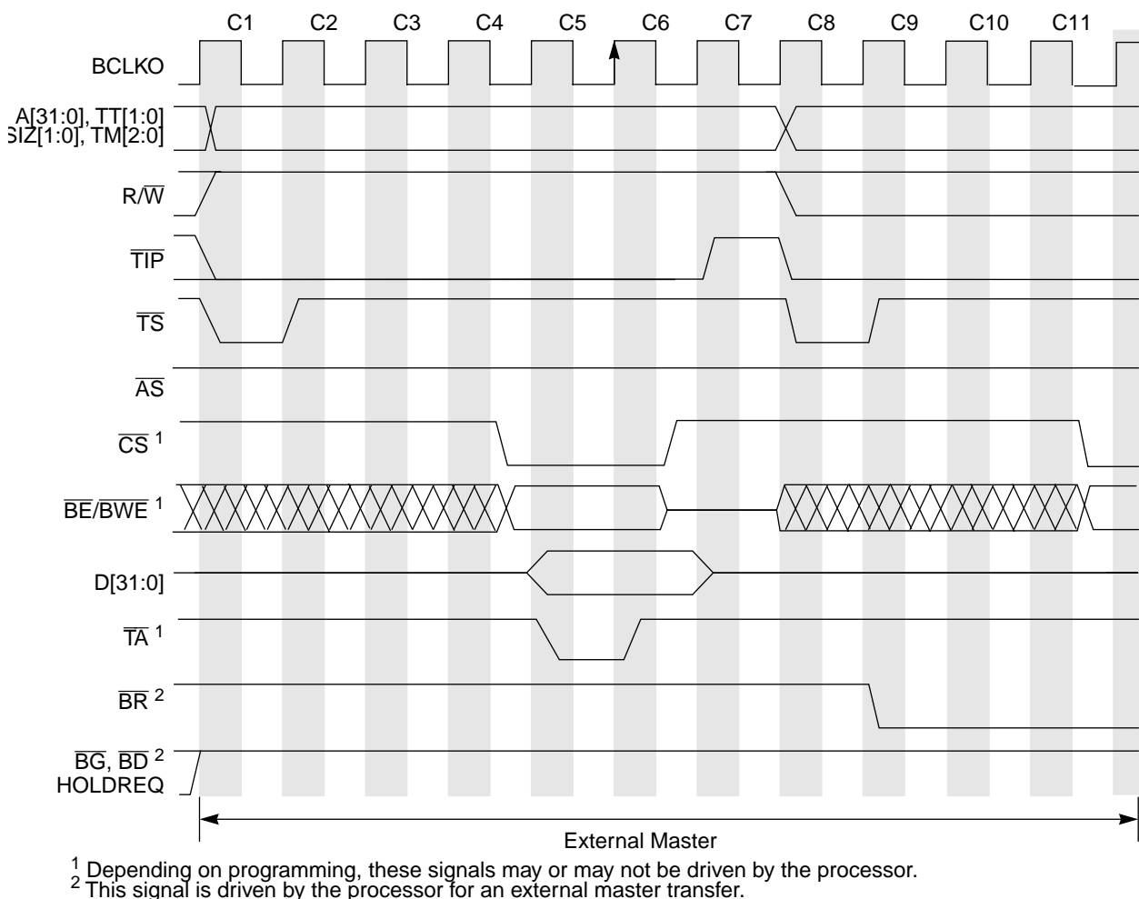
Figure 18-24. Basic No-Wait-State External Master Access
