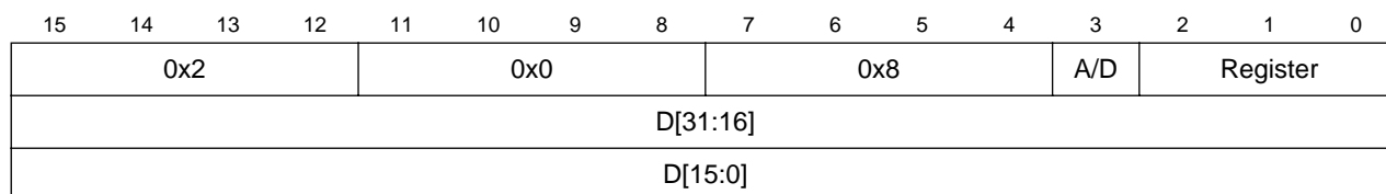
Figure 5-20. WAREG/WDREG Command Format
