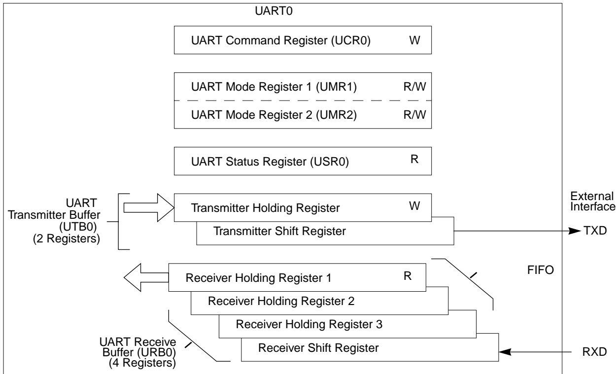
Figure 14-20. Transmitter and Receiver Functional Diagram
