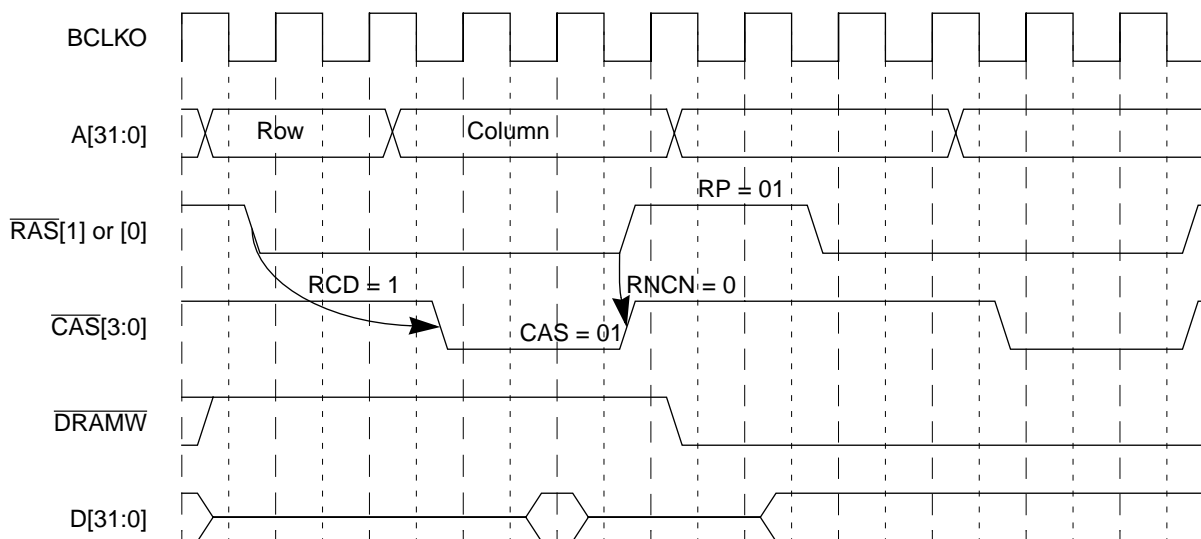
Figure 11-6. Basic Non-Page-Mode Operation RCD = 1, RNCN = 0 (5-5-5)
