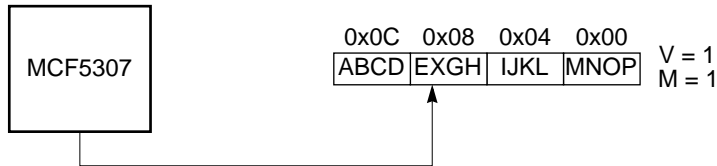
Figure 4-6. Write-Miss in Copyback Mode
