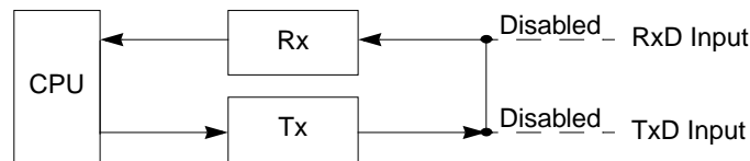
Figure 14-24. Local Loop-Back
