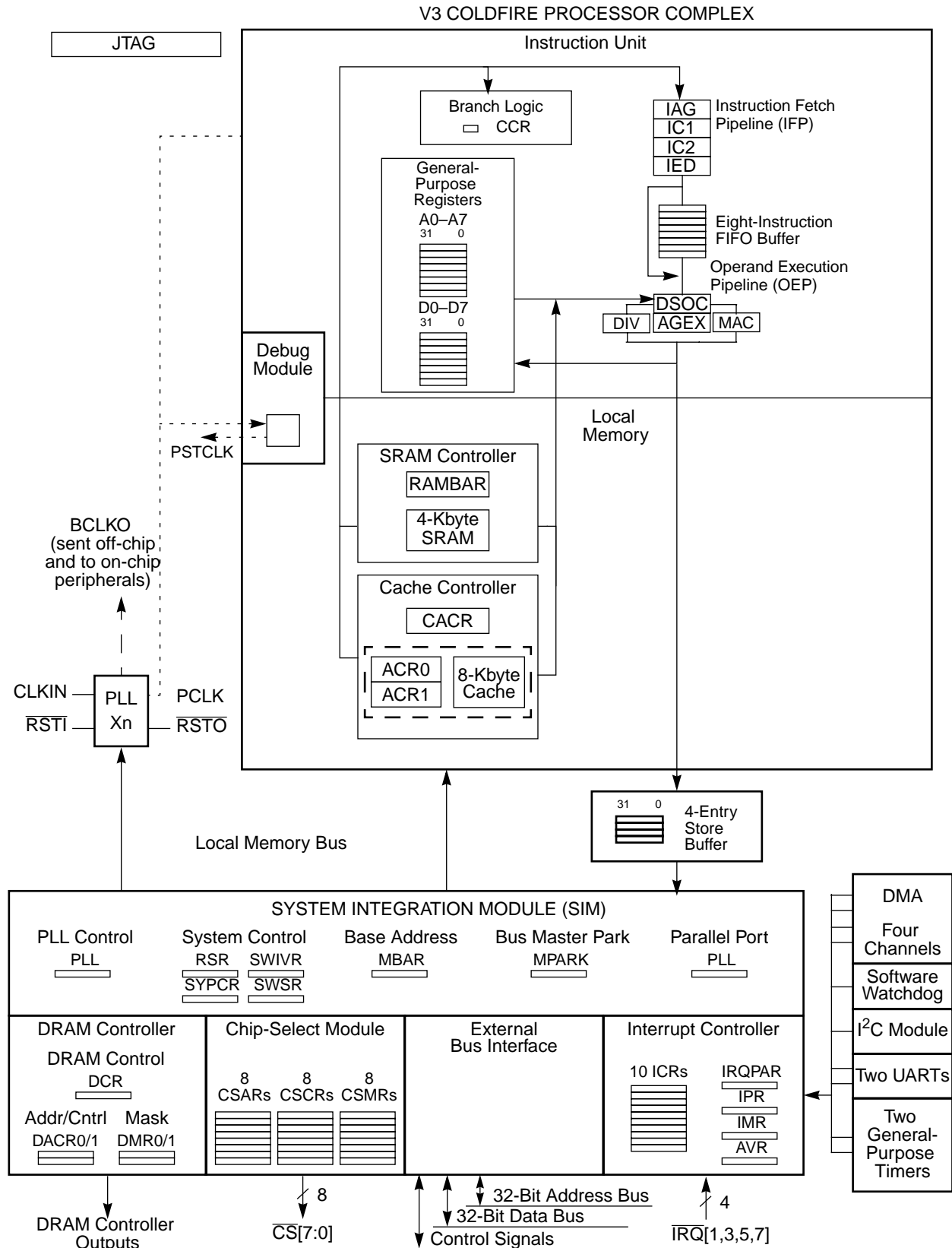
Figure 1-1. MCF5307 Block Diagram
