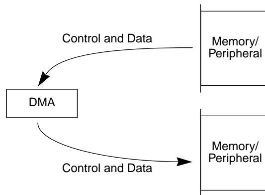
Figure 12-2. Dual-Address Transfer
