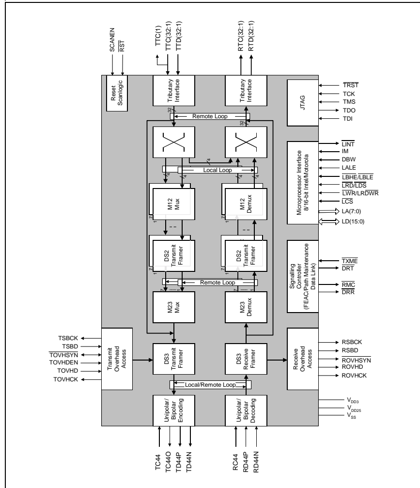
Figure 4 Block Diagram
