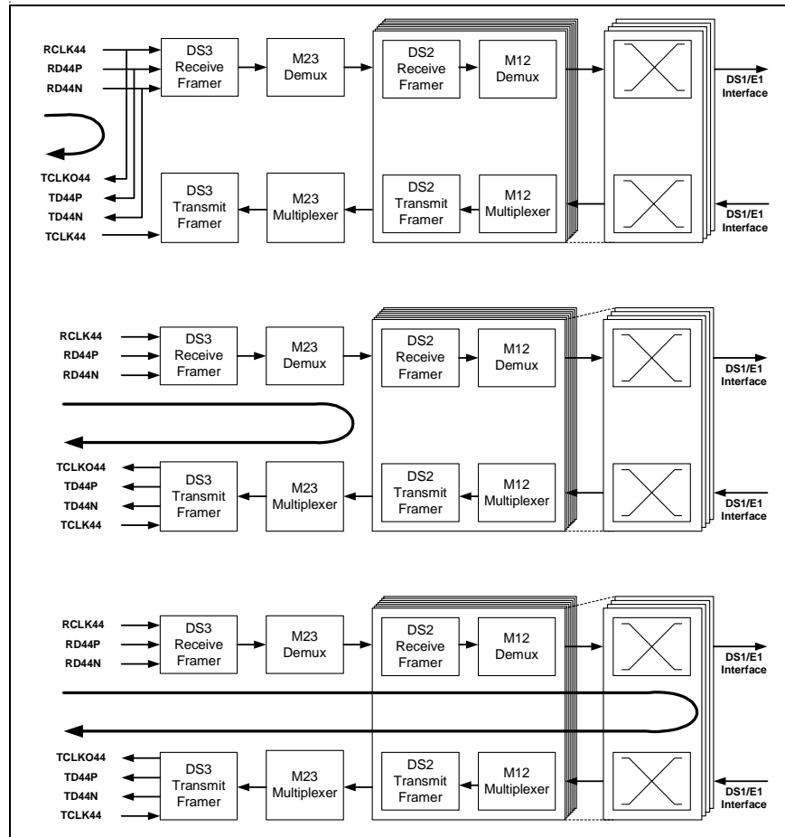
Figure 6 Remote Loops
