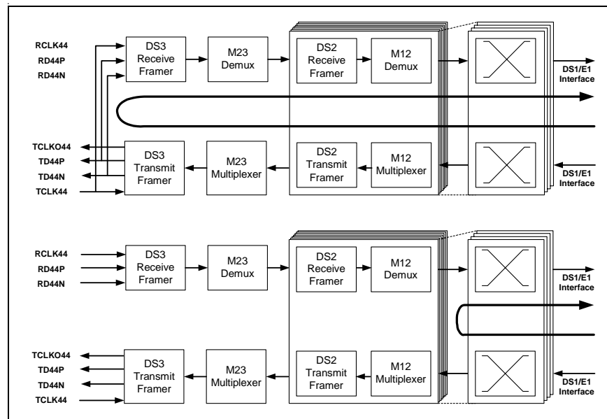
Figure 5 Local Loops
