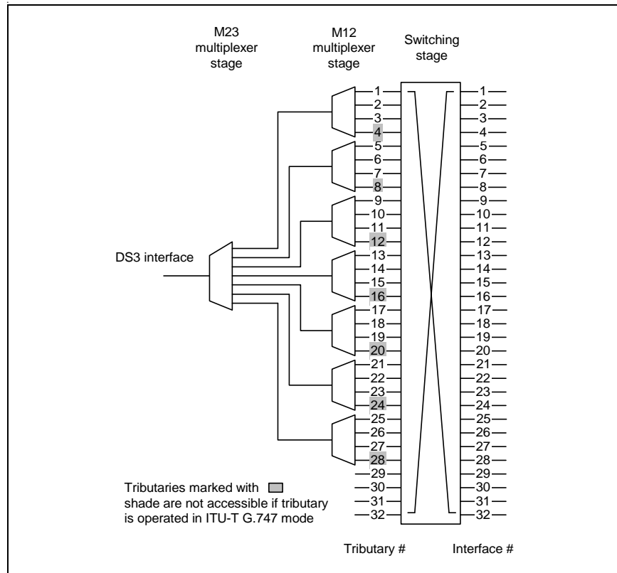
Figure 7 Tributary Mapper
