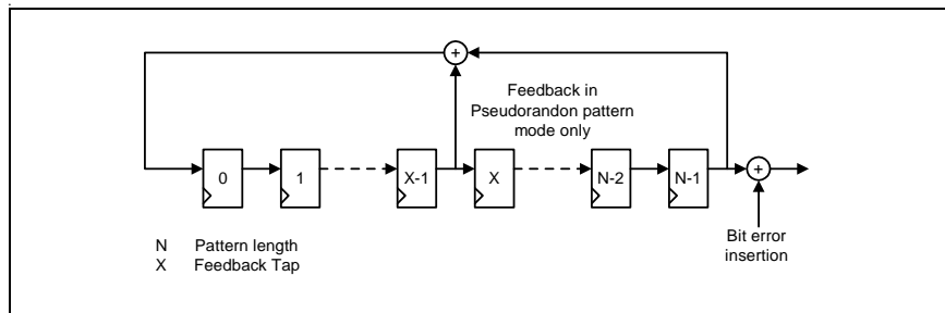
Figure 15 Pattern Generator
