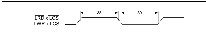
Figure 27 Read, Write Control Interval in Multiplexed Bus Mode
