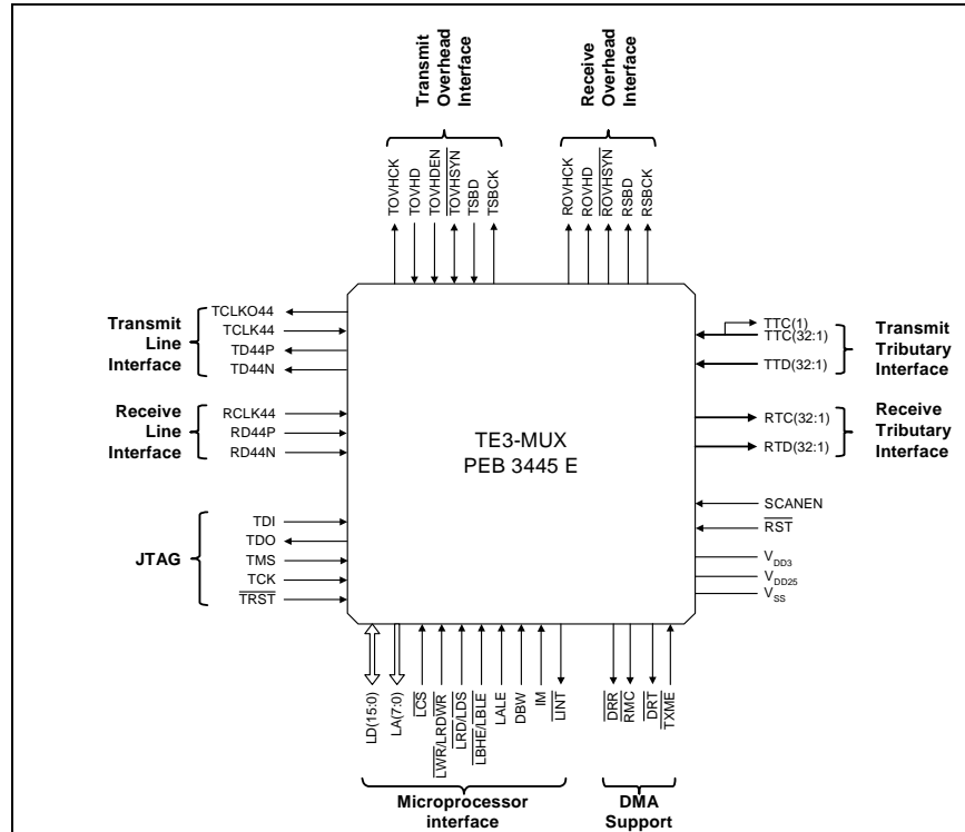
Figure 1 Logic Symbol
