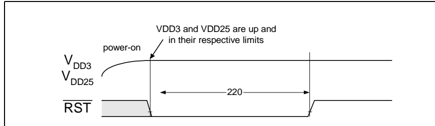
Figure 51 Reset Timing
